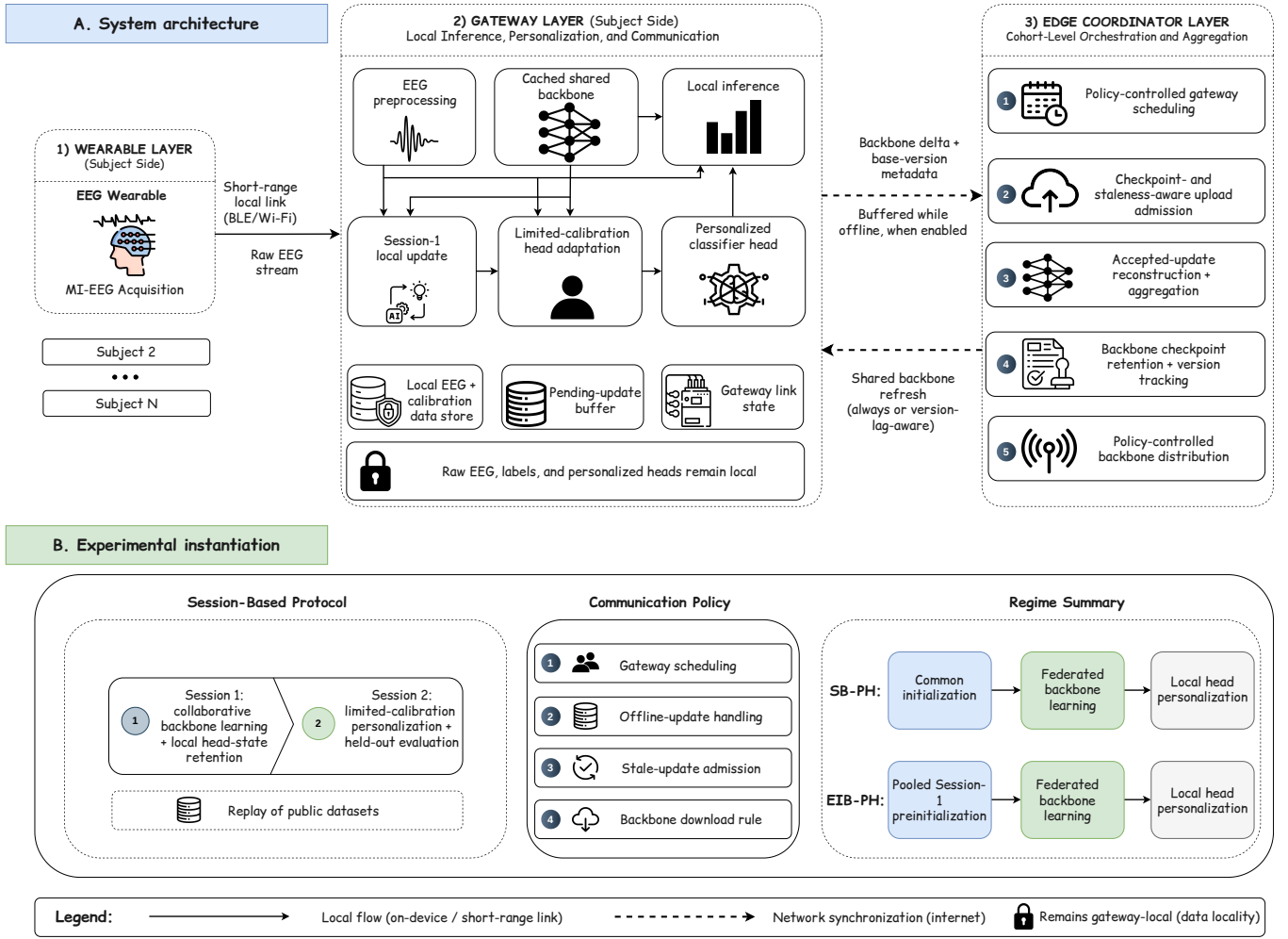
Fig. 1. System architecture and experimental instantiation of NEXUS-MI. (A) The system follows a three-tier wearable–gateway–edge design for communication-aware federated MI-BCI personalization. The wearable acquires MI-EEG signals and streams them to a subject-side gateway, where EEG preprocessing, local inference, Session-1 local updates, limited-calibration head adaptation, local data storage, link monitoring, and update buffering are performed. Raw EEG, calibration labels, and personalized classifier heads remain local to the gateway. The gateway communicates backbone deltas and associated base-version metadata to the edge coordinator, which performs policy-controlled gateway scheduling, checkpoint- and staleness-aware upload admission, accepted-update reconstruction and aggregation, backbone checkpoint retention and version tracking, and policy-controlled backbone distribution according to the active download rule. (B) The architecture in (A) represents the intended deployment workflow, whereas the experiments instantiate this workflow through replay of public session-based MI-EEG datasets rather than a live online deployment. Session 1 supports collaborative backbone learning, while Session 2 uses limited calibration for local head personalization followed by held-out evaluation. The communication policy is defined by four synchronization dimensions: gateway scheduling, offline-update handling, stale-update admission, and backbone download control; the detailed policy configurations are provided in Table I. SB-PH follows common initialization, federated backbone learning, and local head personalization, whereas EIB-PH uses pooled Session-1 preinitialization followed by the same federated backbone-learning and local head-personalization pipeline.
