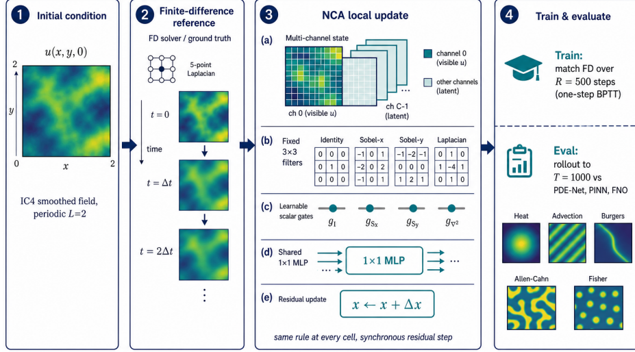
Figure 1: One NCA forward pass: fixed-filter perception with learnable scalar gates, a shared point-wise MLP producing a proposed update, and a synchronous residual update. Repeated application rolls the state forward in time and is trained against ground-truth finite-difference trajectories.
