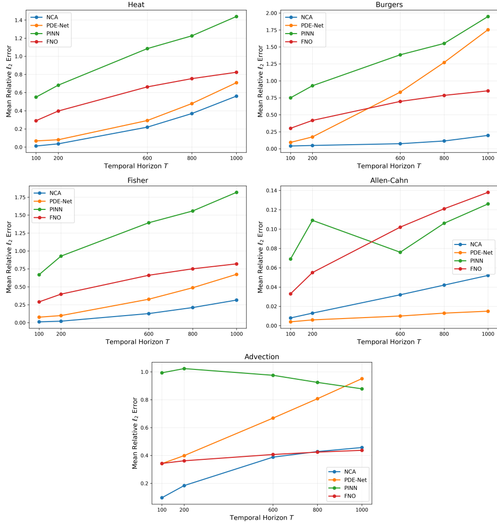
Figure 3: Error growth across temporal horizon for different methods.
