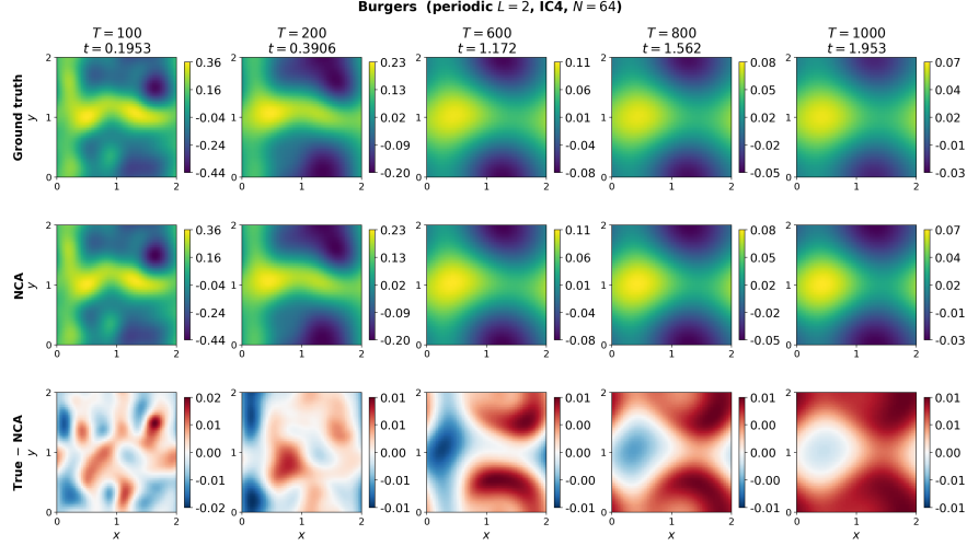
Figure 2: A sample true and learned solution of the Burgers equation using NCA, along with the difference of true solution and learned solution.
