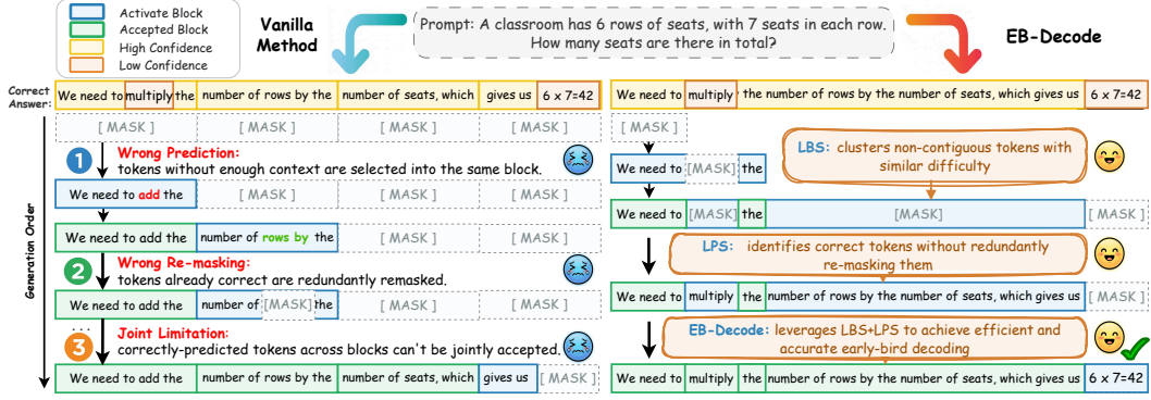
Figure 1: Conceptual comparison illustrating the differences between vanilla block-wise decoding (Left) [1] and the proposed EB-Decode framework (Right).
