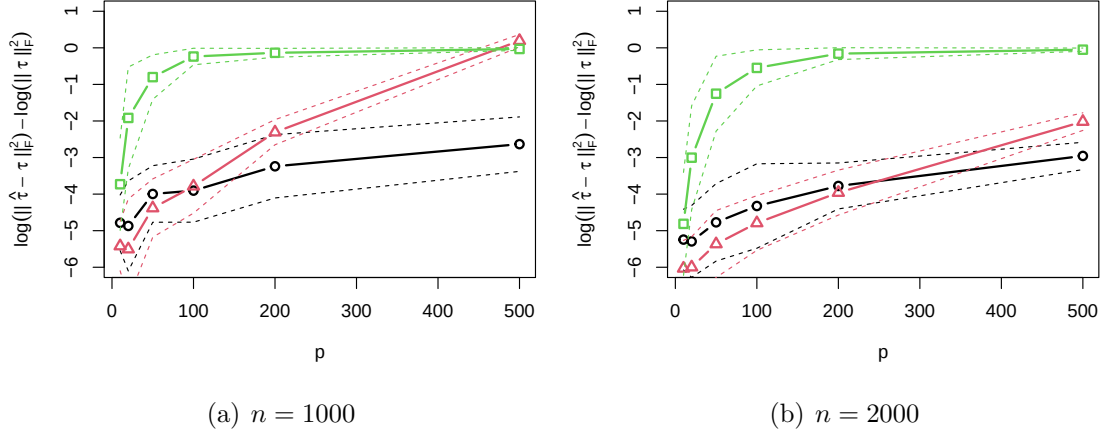
Figure 2: Average estimation error for I(f_X) when X \sim N(\mathbf{0}, \tau^{-1}) using (i) \Sigma_X^{-1} ( -\triangle- ); (ii) \tilde{\Sigma}_X^{-1} ( -\square- ); and (iii) I(\mathcal{X}, k_0, k_1)^* ( -\circ- ). The dashed lines indicate one standard error deviations from the mean.
