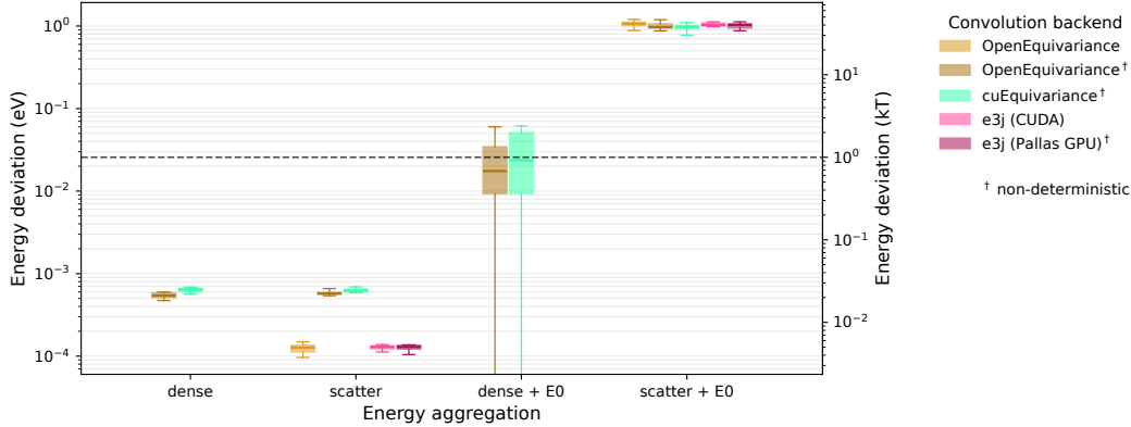
Figure 9: Run-to-run energy deviation of a MACE model (a) on GPU. The trained model used for NPT simulations (table 2) is evaluated on a batch of 8 water boxes totaling 21,016 atoms and 889,840 edges, over a 100 times. The experiment was repeated using different energy aggregation schemes: including or dropping the constant atomic energies ( E_0 ); using mlip ’s default scatter aggregation of node energies over graphs or a dense matrix-vector product for the energy head. The plot represents 5th/95th percentiles as whiskers and 25th/75th percentiles as boxes. When a box is missing, it means that all runs were rigorously deterministic. Hyperparameters are detailed in table 3.
