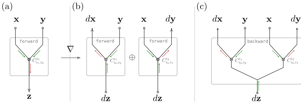
Figure 11: Computation graphs for the tensor product forward pass (a) and backward pass (b-c). Back-propagating through a tensor product operation yields two transposed tensor product operations, by the Leibniz rule. Instead of calling two tensor product kernels, a dedicated backward kernel reuses device code for batch-wise bilinear coupling, while streaming through batches of the dz cotangents only once and thus saving memory traffic.
