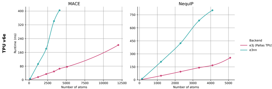
Figure 3: Runtime (ms) for end-to-end force inference of MACE and NequIP on TPU. Inference is performed through integration of additional convolution backends for the mlip library [14] and run on real protein systems with 5Å cutoff. Hyperparameters can be found in table 3: MACE (a) (correlation 2) has 2 layers and NequIP has 5 layers, both have 128 channels.
