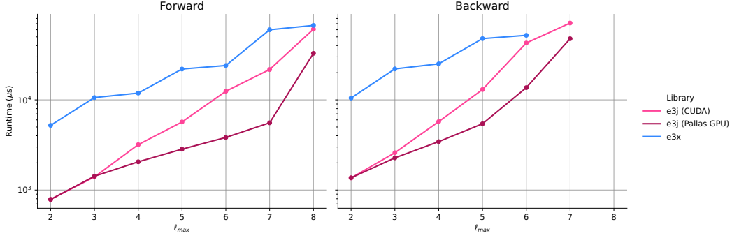
Figure 6: Comparison of e3j and e3x’s FusedTensor tensor products. Benchmarks show the runtime scaling with L = l_{max} with a fixed batch size B = 32,768 and channels C = 128 . Every Clebsch-Gordan path (l_1, l_2, l_3) is symmetric. Runtimes are obtained on a single NVIDIA H100.
