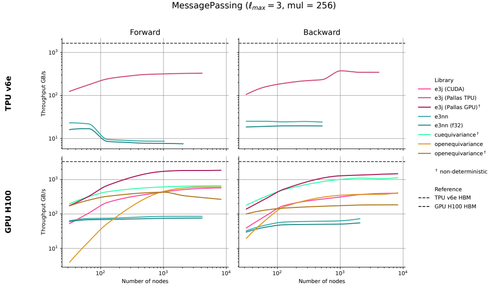
Figure 2: Throughputs (GB/s) for the convolution operation on TPU (top) and GPU (bottom). Here we present results for \ell_{max} = 3 256 channels, alongside the theoretical maximum throughput of a TPU v6e Trillium (1.64 TB/s) and the theoretical maximum throughput of the NVIDIA H100 HBM3 GPU ( \sim 3.35 TB/s) on which the benchmarks were performed. When lines are not complete, it indicates that the library reached the memory bound of the device.
