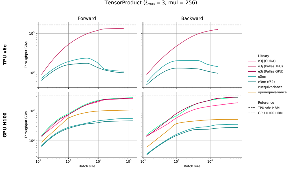
Figure 1: Throughputs (GB/s) for the tensor product operation on TPU (top) and GPU (bottom). The e3j CUDA implementation is compared against cuEq (jax), and e3nn_jax (single precision and default half precision). The e3j Pallas implementation is compared against the only available baseline e3nn_jax for the universal ("full") Clebsch-Gordan tensor product. Results for \ell_{max} = 2 and \ell_{max} = 3 and multiplicities up to 256 channels, alongside the (a) theoretical maximum throughput of the NVIDIA H100 GPU ( \sim 3.35 TB/s) and (b) theoretical maximum throughput of a TPU v6e ( \sim 1.64 TB/s) on which the benchmarks were performed. When lines are not complete, it indicates that the library reached the memory bound.
