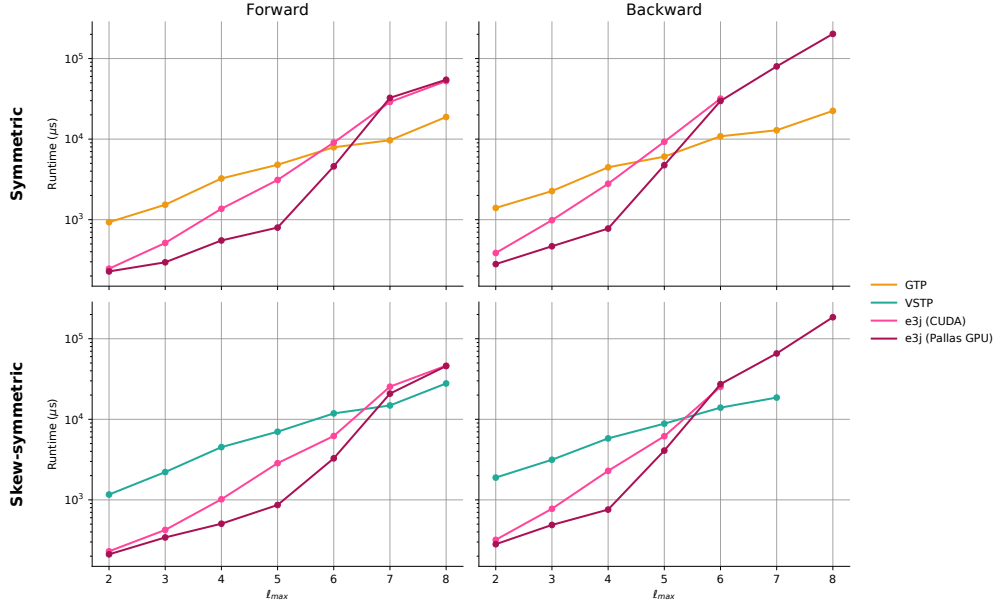
Figure 5: Comparison with Gaunt and Vector Signal Tensor Products. Benchmarks show the runtime scaling with L = l_{max} with a fixed batch size B = 32,768 and channels C = 128 . Every Clebsch-Gordan path (l_1, l_2, l_3) is symmetric or skew-symmetric, according to the parity of l_1 + l_2 + l_3 . The symmetric panel, where the sum is even, benchmarks the \mathbf{e}3\mathbf{j} tensor product on symmetric paths against the Gaunt tensor product (GTP) [19], whilst the skew-symmetric panel benchmarks against the vector signal tensor product (VSTP) [20, 21]. Both the GTP and the VSTP are evaluated through integral formulas on a spherical t -design quadrature [36]. Runtimes are obtained on a single NVIDIA H100.
