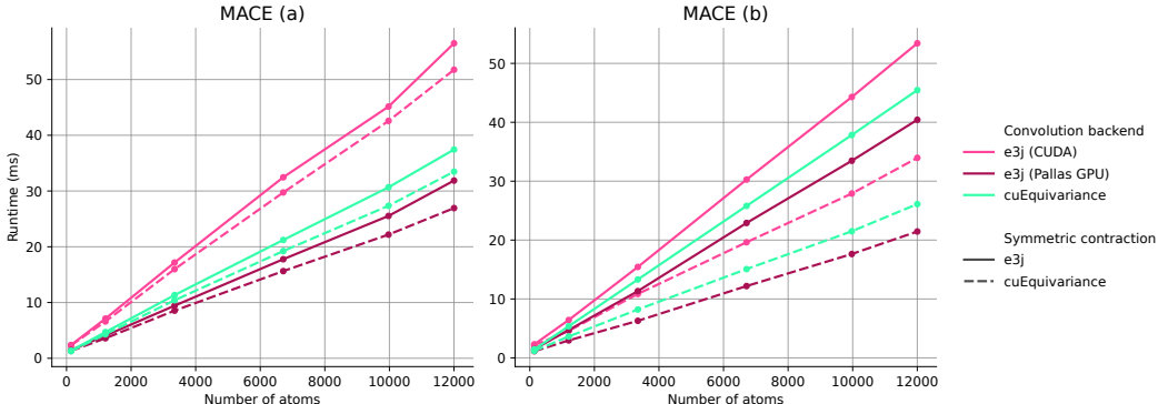
Figure 8: Effect of the SymmetricContraction backend for the MACE model on GPU. We compare the effect of replacing the naive e3j -based power expansion, followed by a species-wise linear projection of higher-order features, with the dedicated SymmetricContraction kernel of cuEquivariance . The two variants (a) and (b) of the MACE model are detailed in table 3.
