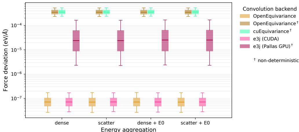
Figure 10: Run-to-run force deviation of a MACE model (a) on GPU. The trained model used for NPT simulations (table 2) is evaluated in the same conditions as figure 9. Because XLA can eliminate the addition of atomic energies, and because the VJP of the scatter operation is a deterministic gather operation, we see that the addition of E_0 and the aggregation method have no effect on the deviation of forces. Even with deterministic convolution kernels, forces have non-zero deviations due to some forward gather operations being transposed as non-deterministic scatter operations. Interestingly the Pallas GPU kernel, only deterministic in the forward pass, lies in between.
