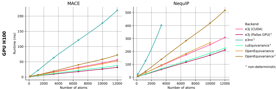
Figure 4: Runtime (ms) for end-to-end force inference of MACE and NequIP on GPU. Inference is performed through integration of additional convolution backends for the mlip library [14] and run on real protein systems with 5Å cutoff. Hyperparameters can be found in table 3: MACE (a) (correlation 2) has 2 layers and NequIP has 5 layers, both have 128 channels.
