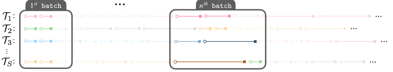
Figure 6. Maintaining S independent slots ( \mathcal{T}_1, \dots, \mathcal{T}_S ) enables (i) learning child segments before their parents and (ii) mixing diverse sample lengths within batches. Each slot begins by emitting single-step leaves, as illustrated by the 1 st batch; as slots drain and refill at different rates, they become desynchronized, mixing short-horizon and long-horizon segments, as in the n^{\text{th}} batch. Each slot schedules a new tree once its current one is consumed.
