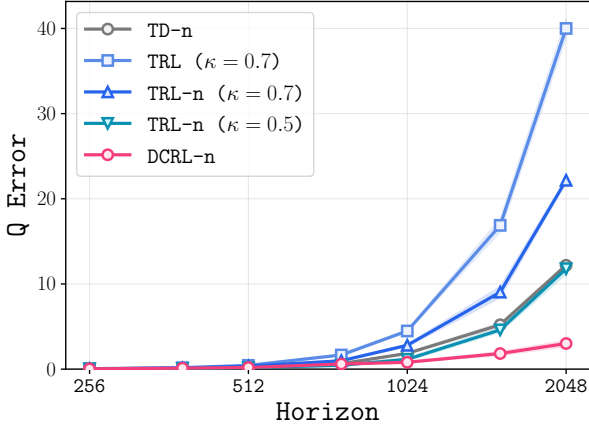
Figure 10. On combination-lock, accumulated error \mathcal{A}(H) from Eq. (8) (3 seeds; shading: \pm 1 s.d.). Adding n -step propagation reduces TRL’s error, while symmetric transitive regression ( \kappa = 0.5 ) further lowers TRL- n ’s error to the TD- n level. DCRL- n remains lowest and grows slowest, consistent with its logarithmic bootstrap depth and child-to-parent scheduling.
