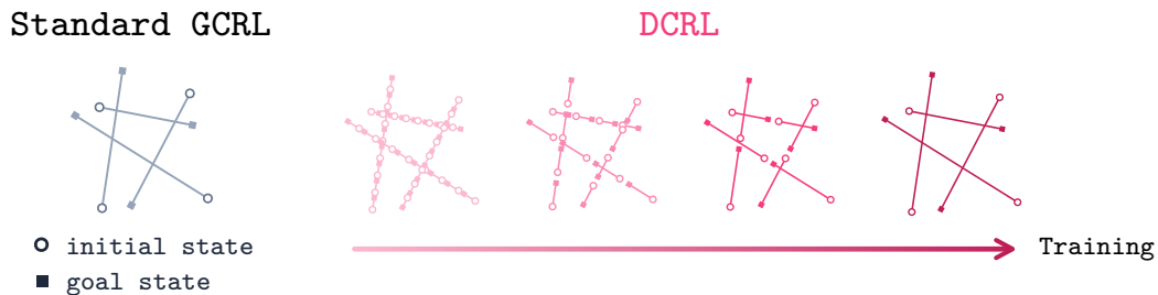
Figure 1. DCRL (right) learns short segments first, then uses them to learn longer ones, whereas standard GCRL (left) randomly samples pairs of all lengths in no particular order.
