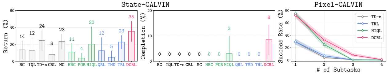
Figure 8. DCRL achieves the highest four-subtask completion rate on state-based CALVIN (8%), versus 3% for the best hierarchical baseline and 0% for all flat baselines. On pixel-based CALVIN, which excludes privileged object poses, DCRL reaches at least three subtasks in 8% of rollouts and all four in 1%, whereas all three baselines remain at 0% beyond two subtasks.
