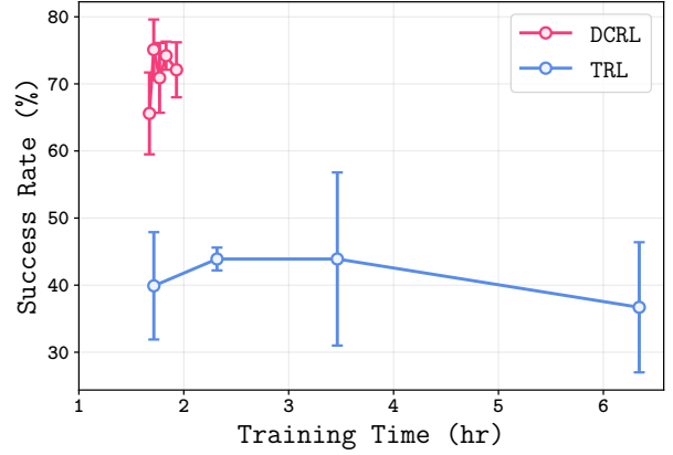
Figure 17. Same Pareto analysis as Fig. 16 in cube-triple. DCRL consistently achieves a better trade-off between performance and training efficiency than TRL. DCRL is trained with varying numbers of slots ( S ) and a fixed batch size (1024), while TRL is trained with varying batch sizes ( bs ).
