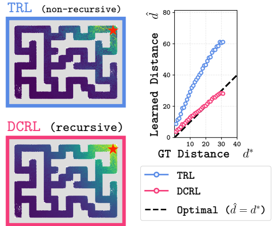
Figure 2. In humanoidmaze-giant , DCRL learns near-optimal distance estimates. We measure the distances predicted by DCRL and TRL from each state to a fixed goal (red star).
