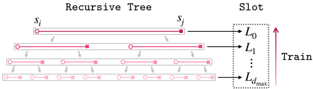
Figure 5. A recursive tree is flattened into a slot, ordered from leaves ( L_{d_{\max}} ) to the root ( L_0 ), so every child is learned before its parent.
