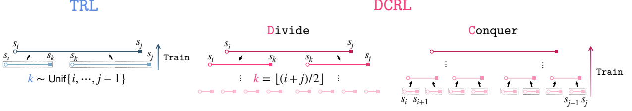
Figure 3. DCRL explicitly implements divide-and-conquer . Divide: Split a root segment (s_i, s_j) at its midpoint, then recursively split each half until reaching single-step leaves. Conquer: Train the value function on leaves first and then on their parents, proceeding up to the root. In contrast, TRL backs up from a single random subgoal s_k , where k \in \{i, \dots, j-1\} .
