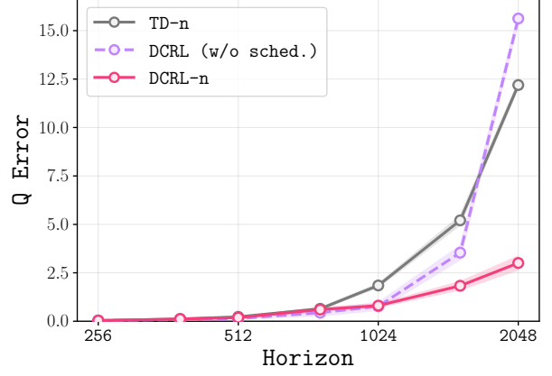
Figure 11. On combination-lock, we isolate child-to-parent scheduling while holding the factorized backup and n -step propagation fixed (3 seeds; shading: \pm 1 s.d.). I.i.d. sampling performs comparably for H \lesssim 1024 , but its error rises sharply at longer horizons and approaches TD- n ’s. DCRL- n remains flat, showing that ordering becomes important as dependency chains deepen.
