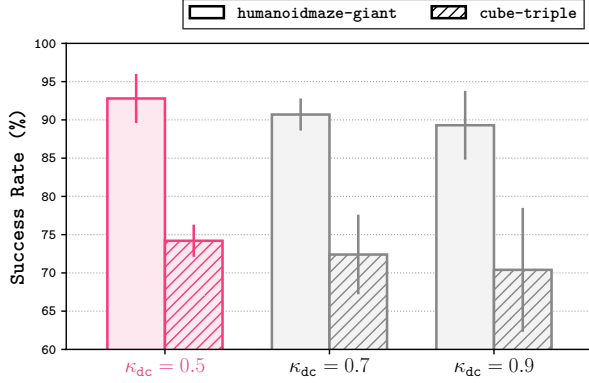
Figure 14. Ablation of the expectile parameter \kappa_{dc} for the divide-and-conquer loss \mathcal{L}^{dc} . Performance peaks at \kappa_{dc} = 0.5 (our default).
