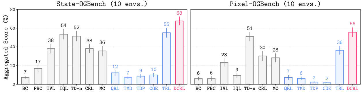
Figure 7. DCRL achieves state-of-the-art performance on standard OGBench tasks across diverse task domains and observation modalities. Full results are in Tables 15 and 16.
