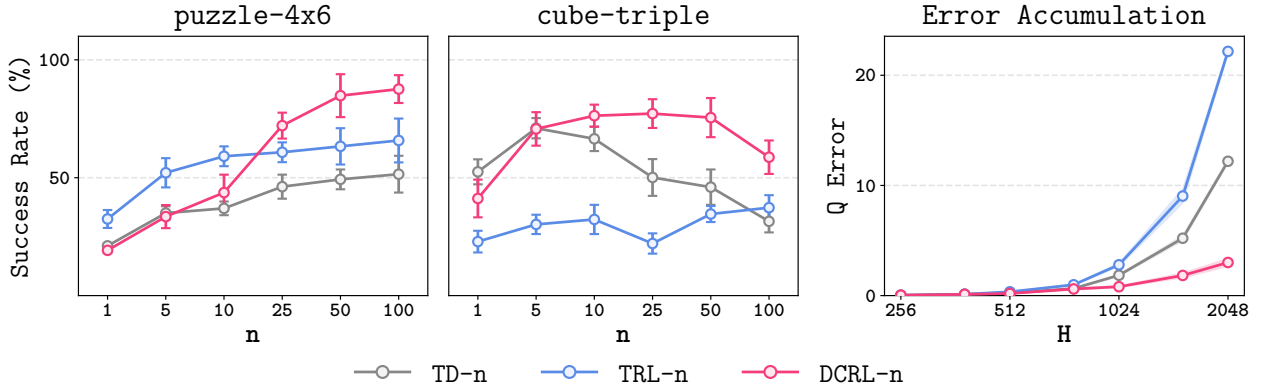
Figure 9. Left: DCRL- n surpasses TD- n and TRL- n at long propagation horizons ( n \geq 25 ). Right: Q-error in DCRL- n grows far more slowly with task horizon H than in the others.
