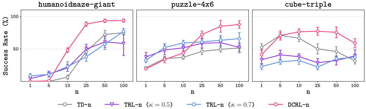
Figure 12. Exhaustive comparison across propagation horizons n on three long-horizon environments. We report success rate across n \in \{1, 5, 10, 25, 50, 100\} . DCRL- n performs best for n \geq 25 on all tasks, while the two TRL- n variants perform similarly overall.
