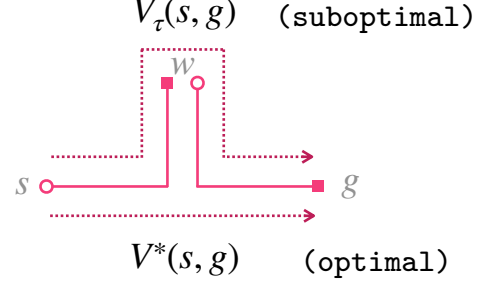
Figure 4. Optimal values require composing segments across trajectories. Given s \rightarrow w and w \rightarrow g , the optimal route from s to g cannot be recovered from V_\tau alone.
