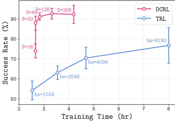
Figure 16. Across training budgets, DCRL outperforms TRL. In humanoidmaze-giant, we plot success rate (%) against training time (hours), while varying the number of slots ( S=16, 32, 64, 128, 256 ) for DCRL at a fixed batch size (1024), and varying the batch size ( bs=1024, 2048, 4096, 8192 ) for TRL.
