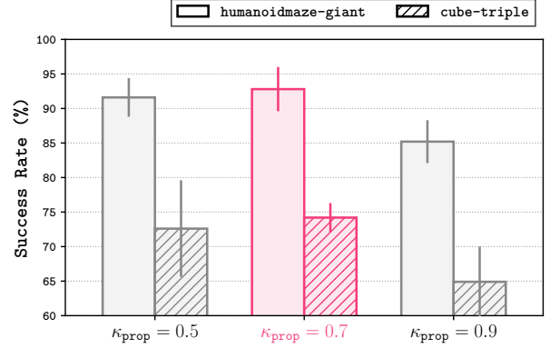
Figure 15. Ablation of the expectile parameter \kappa_{prop} for the propagation loss \mathcal{L}^{prop} . Performance peaks at \kappa_{prop} = 0.7 (our default).
