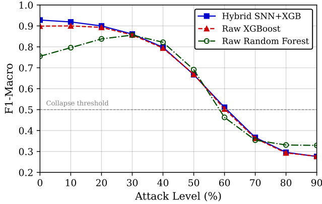
(a) F1-Macro degradation across attack levels.
