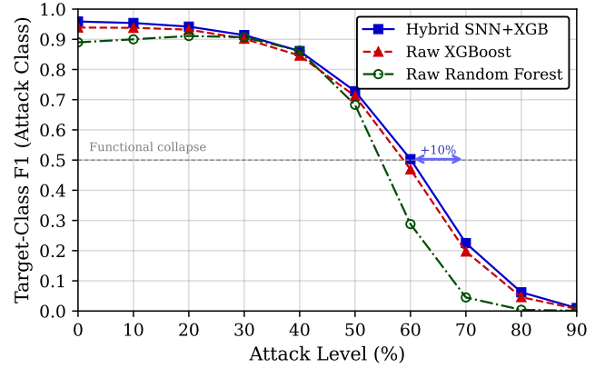
(b) Target-class F1 showing collapse delay.
