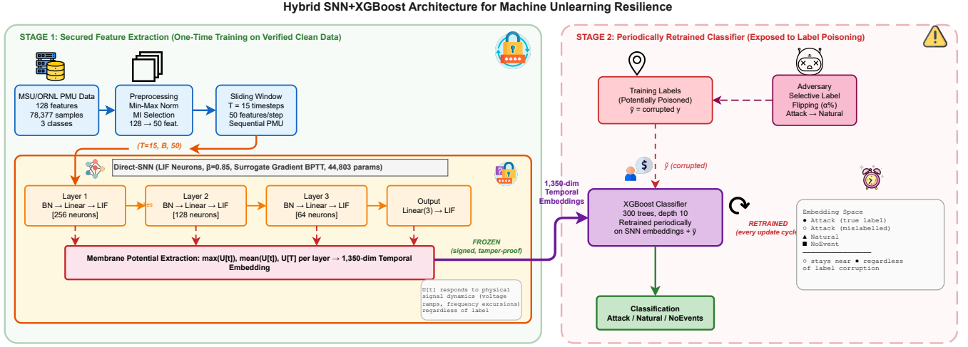
Fig. 1: Proposed hybrid SNN+XGBoost architecture for machine unlearning resilience. The SNN feature extractor (Stage 1) is trained once on verified clean data and deployed as a fixed neuromorphic frontend. Only the XGBoost classifier (Stage 2) is exposed to periodic retraining with potentially poisoned labels. The SNN temporal embeddings encode physical signal dynamics that are invariant to label corruption.
