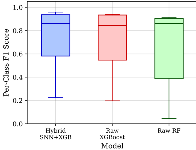
Fig. 4: Distribution of target-class F1 scores across attack levels (0–70%). The hybrid exhibits the highest median and tightest interquartile range, demonstrating more consistent robustness. Raw Random Forest shows the largest spread, reflecting its catastrophic collapse at moderate attack levels.
