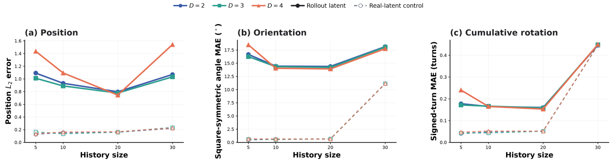
Figure 12: History-length and predictor-depth ablation on 2D square dataset at a common 32-step rollout horizon. Solid lines use predicted rollout latents; dashed lines use real encoder latents and isolate representation and probe error. Color and marker shape denote predictor depth. Lower is better.
