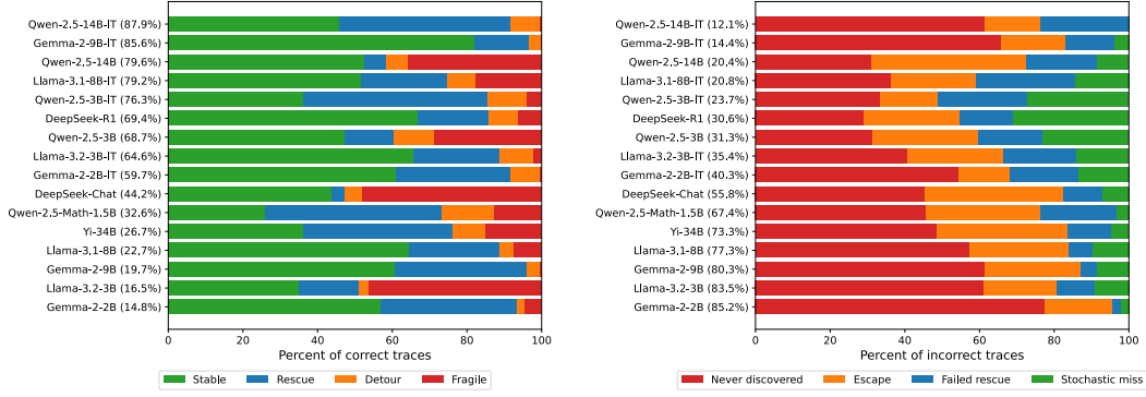
(a) Success mechanisms among correct traces.
