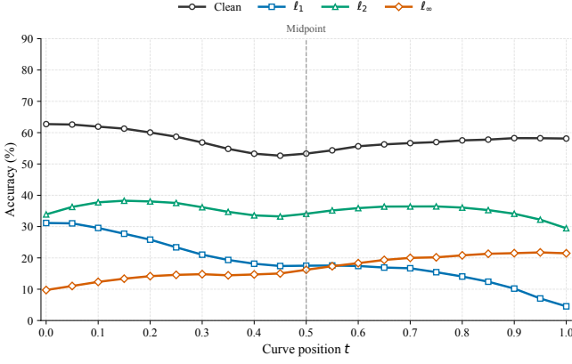
Fig. 2. Clean and norm-specific adversarial accuracy along the robust connectivity curve of WideResNet-28-10 on CIFAR-100, evaluated using AutoAttack. Different curve locations exhibit distinct robustness preferences.
