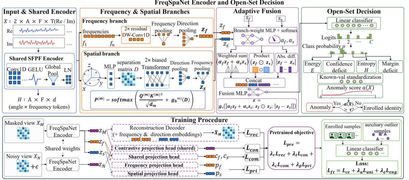
Fig. 1. Architecture and learning pipeline of FreqSpaNet.
