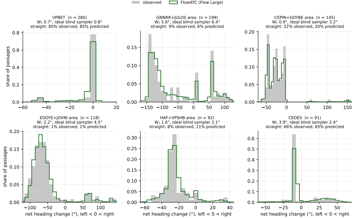
Fig. 14 Observed and sampled maneuver distributions at the six branch points with the most test passages. Gray bars: share of observed test passages per bin of net heading change \theta (left turns negative, right turns positive, straight flight near zero). Green line: share of FlowATC samples (Flow Large, K=50 per passage) in the same bins. Titles give the number of passages n , the 1-Wasserstein distance W_1 between the two distributions, the value an ideal history-blind sampler would reach on this test set, and the observed and predicted shares of straight flight ( |\theta| < 10^\circ ). The horizontal range covers the 1st to 99th percentiles of both distributions. No catalogue information enters the figure.
