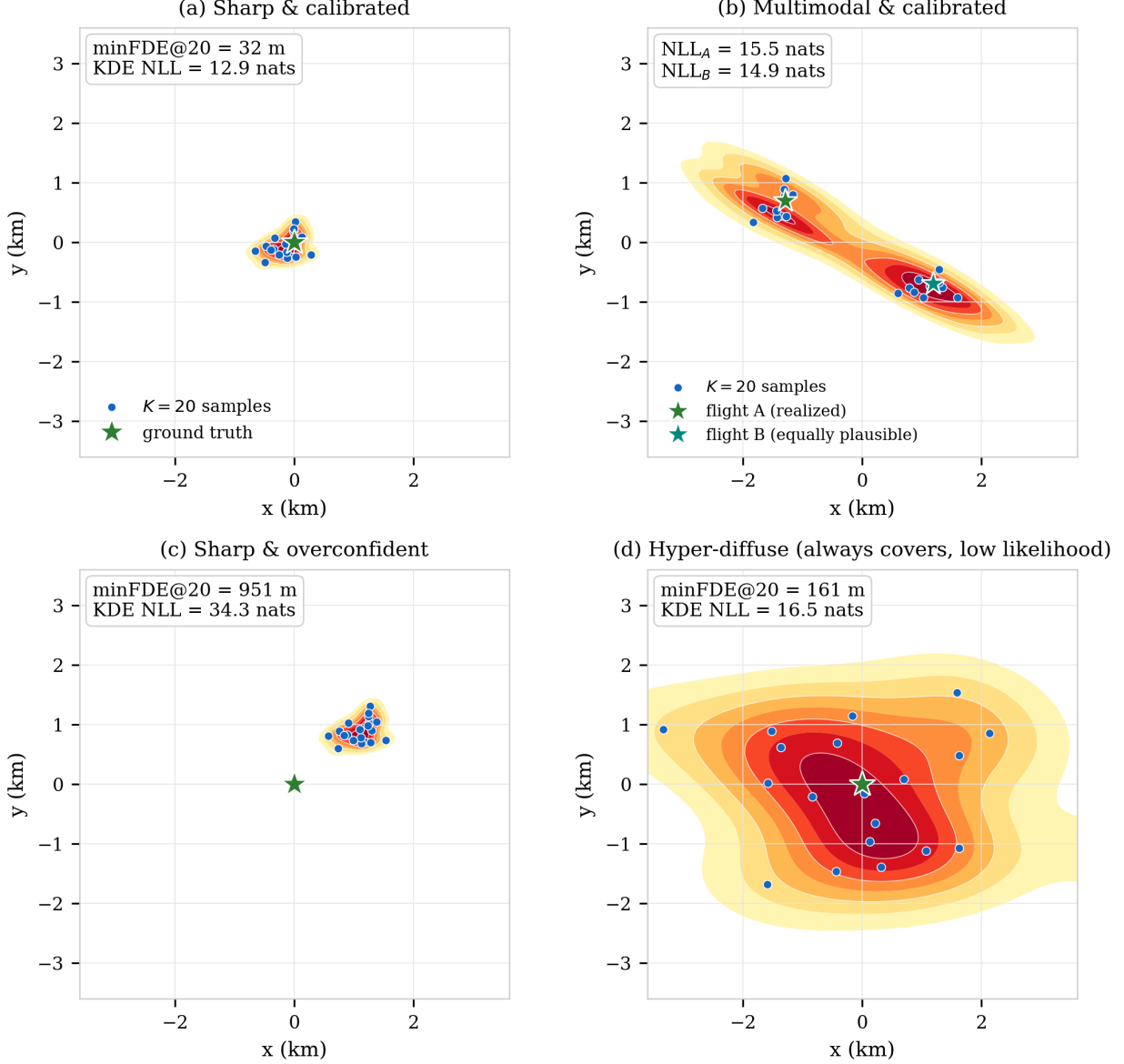
Fig. 2 Four synthetic K=20 sample-cloud scenarios, with the actual \text{minFDE@20} and KDE NLL computed via Eq. (4). (a) Sharp and calibrated : both metrics agree. (b) Multimodal and calibrated : two equally plausible maneuvers; the bimodal density scores well against either outcome ( \text{NLL}_A=15.5 , \text{NLL}_B=14.9 nats), (c) Sharp but displaced : over-confidence makes the NLL diverge even though the samples are tightly clustered. (d) Hyper-diffuse : spreading the samples widely keeps \text{minFDE@20} comparable to (b), yet the likelihood assigned to the true outcome is markedly lower everywhere.
