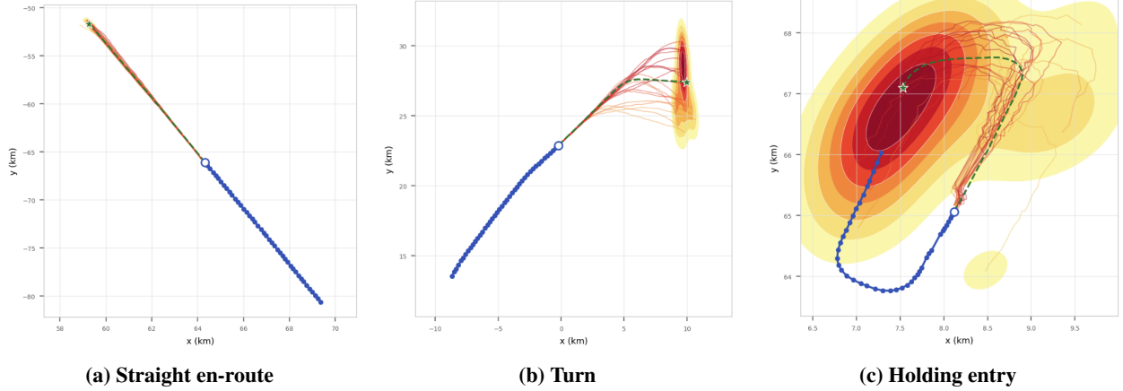
Fig. 6 Final-position probability density maps ( K = 20 samples, Gaussian KDE, Scott bandwidth). Dashed blue: observed past; dashed green: ground-truth future; solid heatmap: sampled trajectories; green star: ground-truth final position; yellow–red: predicted final-point density (light = low, dark = high). Density width correlates with the complexity of the anticipated maneuver.
