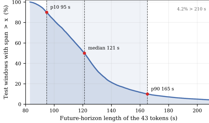
Fig. 8 Portion of test windows reaching a given future horizon.
