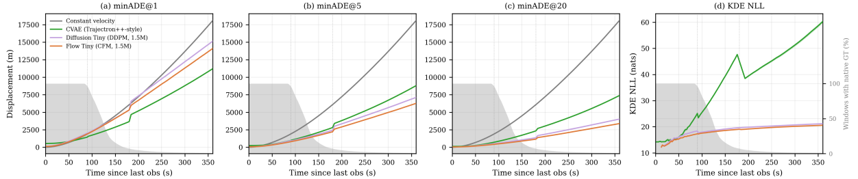
Fig. 18 Full K \in \{1, 5, 20\} extrapolation sweep, extending Fig. 9 with the intermediate K=5 panel.
