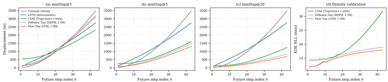
Fig. 17 Full K \in \{1, 5, 20\} displacement-error sweep, extending Fig. 7 with the intermediate K=5 panel.
