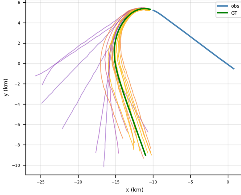
Fig. 5 Predicted trajectory fan ( K = 20 samples). Blue: observed past; Green: ground-truth future; purple–yellow: predicted final-point density (purple = low, yellow = high).
