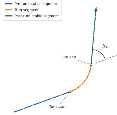
Fig. 19 A turn event is defined as the transition between two locally stable ground-track segments. The detected turn start and end delimit this transition, while the turn angle, \Delta\psi , is the wrapped angular difference between the mean ground-track directions of the pre-turn and post-turn stable segments.
