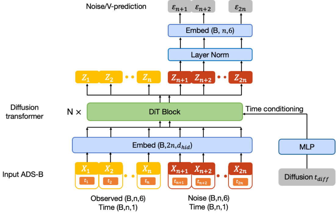
Fig. 3 FlowATC DiT[11] architecture overview.
