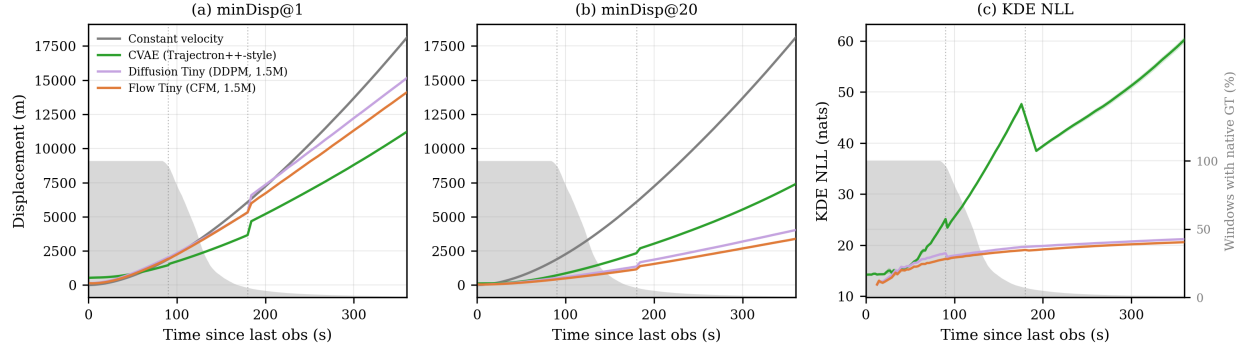
Fig. 9 Extrapolation error and calibration beyond the training horizon. (a)–(b) minDisp@ K for K \in \{1, 20\} . (c) KDE NLL. Gray shading (right axis): fraction of test windows with native ground-truth coverage. The full K \in \{1, 5, 20\} sweep is given in Appendix G.
