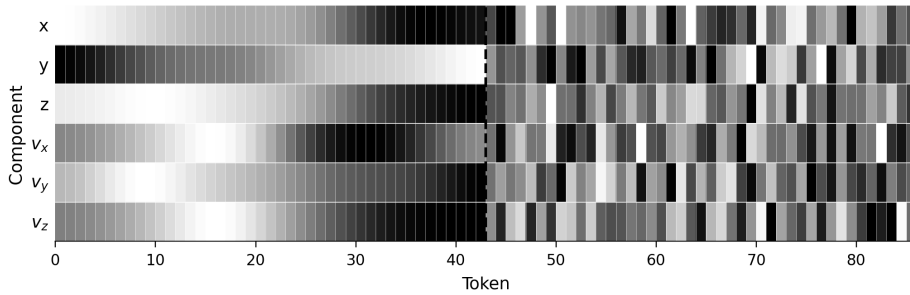
Fig. 4 Trajectory represented as a 6 \times 86 feature-time matrix. The observed prefix (solid, left of dashed line) provides context tokens; the noisy future suffix (light, right) is the region to be inpainted by the flow-matching model.
