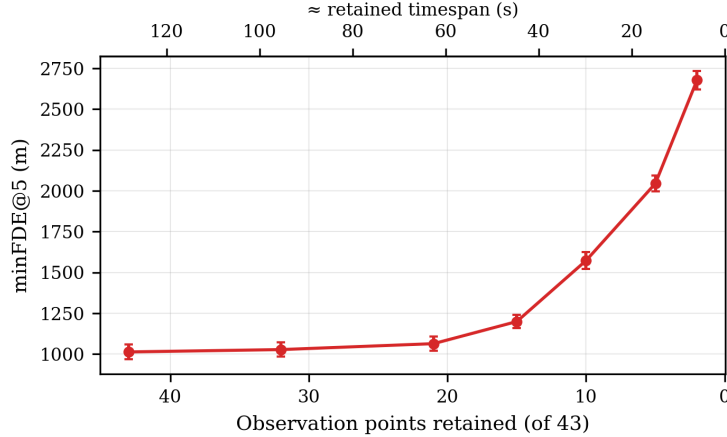
Fig. 10 Displacement error as a function of retained observation history. minFDE@5 (mean \pm SEM, N=2000 ) as the observed prefix is shrunk from 43 points ( n_{\text{keep}} ) to progressively shorter spans; the earliest 43 - n_{\text{keep}} tokens are frozen (repeated from the earliest retained sample) since the backbone’s positional embeddings fix the input length at 43. Error is essentially flat down to n_{\text{keep}} \approx 21 and rises sharply below n_{\text{keep}} \approx 15 .
