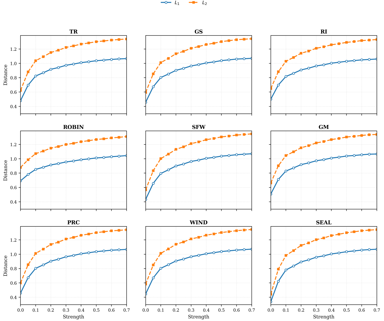
Figure 10: Mean L_1 and L_2 noise distances vs. attack strength \lambda across nine watermarking methods. Across the measured grid, both metrics increase and approach the random-Gaussian diagnostic values. This trend is empirical: Theorem B.8 bounds fixed-depth source dependence and does not predict monotonicity of these distances. Corollary B.10 conditionally formalizes only the squared- L_2 2d reference; the L_1 value additionally assumes independent Gaussian coordinates.
