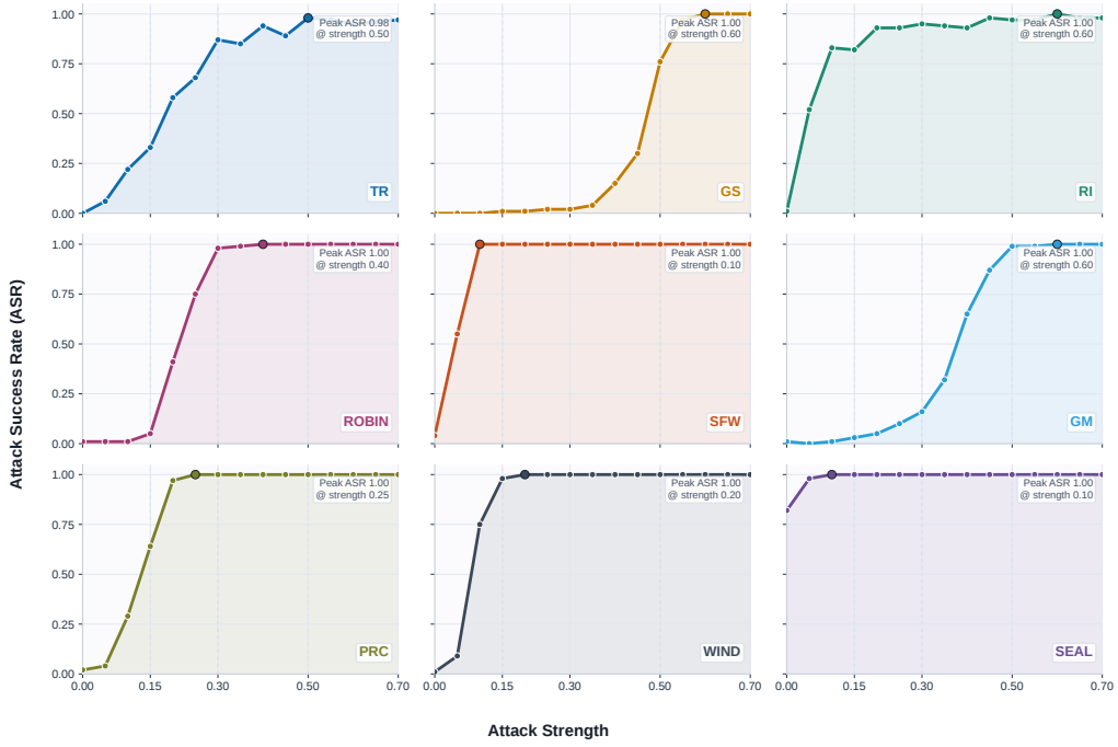
Figure 11: Sensitivity to the re-noising strength \lambda . ASR as a function of \lambda for all nine watermark families. The widely separated saturation thresholds motivate selecting the smallest successful strength for each image rather than applying one global value.
