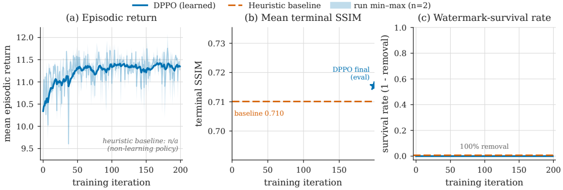
Figure 4: DPPO training dynamics. (a) Mean episodic return rises and plateaus; (b) mean terminal SSIM improves; (c) returned retained outputs remain verifier-rejected throughout. The first two trends are empirical; Proposition 4.5 explains only the same-verifier rejection invariant.
