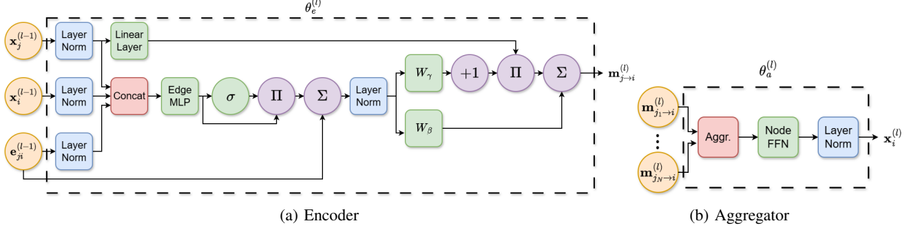
Fig. 3: Gated message-passing layer of MANET-GNN.
