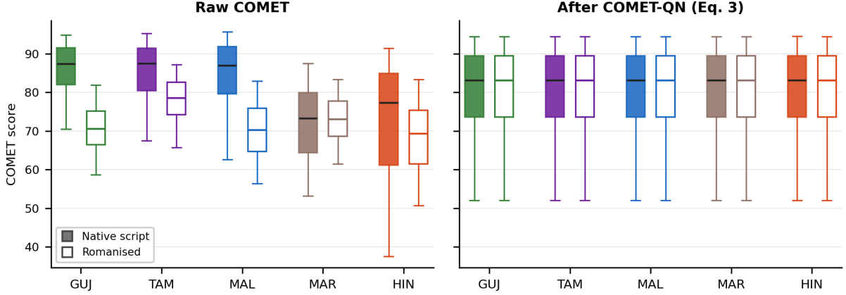
Figure 1: COMET-QN across the ten (language, script) cells (boxes: median, IQR, 5th–95th percentiles; 6,995-segment working set). Left, raw COMET (mean |\text{per-lang. gap}| = 8.14 pts; pooled \rho_S = 0.300 ): native cells, filled, sit consistently above their romanised counterparts, open, by a margin that varies across languages and reverses for MAR, which is problem P1 (§6.1). Right, after COMET-QN (Eq. 3; mean |\text{per-lang. gap}| = 0.00 pts; pooled \rho_S = 0.399 ): all cells share the pooled native reference, so the gap is exactly zero by construction and cross-script comparison becomes meaningful. Pooled Pearson agreement rises from 0.324 to 0.400 over the same cells, while within-language agreement is unchanged to four decimals, GUJ standing at 0.5903 before and after. Within-cell ordering is provably untouched (Eq. 2).
