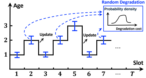
Figure 1: An illustration of the evolution of model age and the associated degradation cost. At each slot, the model age increments by one if no update is performed and resets to one upon an update. It incurs a random degradation cost following the probability distribution f_a at age a .
