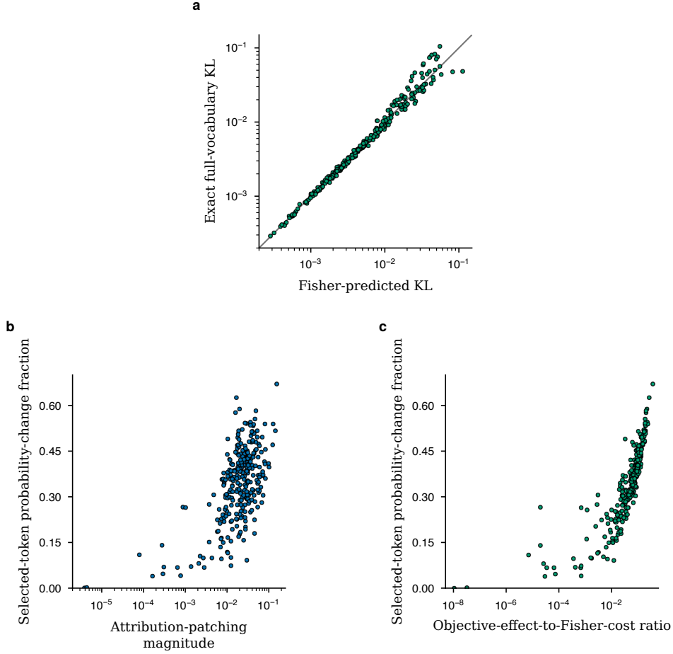
Extended Data Fig. 6 | Output geometry predicts the causal cost and selectivity of sparse features. Pythia-410M, layer 12, Top- k sparse autoencoder. Points in every panel are the same 303 unique zero ablations of active sparse-autoencoder (SAE) features from 57 evaluation-active features across 18 held-out context clusters; feature and objective selection used 18 disjoint discovery contexts. Opaque green points in a and c mark Fisher quantities, while blue points in b mark attribution patching; every point has a black border. a , The Fisher prediction \frac{1}{2}\Delta h^\top G \Delta h against exact full-vocabulary \text{KL}(p_0 \| p_{\text{zero}}) (Spearman \rho = 0.997 ); grey line, equality. b , Attribution-patching magnitude against the selected-token probability-change fraction, the fraction of full-vocabulary absolute probability change on discovery-selected tokens ( \rho = 0.506 ). c , The objective-effect-to-Fisher-cost ratio against the same endpoint ( \rho = 0.935 ); its correlation exceeds that of attribution patching by 0.429 (95% context-cluster bootstrap interval 0.296–0.553). The comparison concerns concentration on selected tokens; attribution-patching magnitude remains the stronger predictor of absolute effect magnitude.
