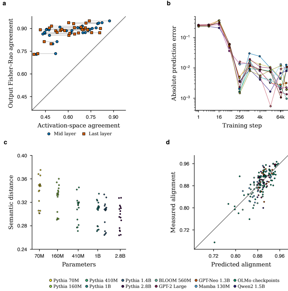
Figure 2: Predictive geometry is shared across models and approaches human completion structure. a , Output Fisher–Rao agreement against activation-space agreement on natural text for all 29 cross-tokenizer, cross-family dyads among ten models (70M–7B; transformer, state-space and recurrent). Each dyad contributes a blue mid-layer circle and vermillion last-layer square joined by a horizontal line; the grey line is equality. The output relation is stronger than either activation relation for every displayed mark. b , Absolute held-out error of the exchangeable six-scalar prediction across ten public training checkpoints. Circles show all 96 defined predictions; colours distinguish individual comparisons and lines follow them across training. Six predictions are defined per checkpoint at steps 1–64 and twelve from step 256; estimator definitions and early-checkpoint coverage are given in Supplementary Note 4. c , Native model samples approach human completions with scale. Points show all 96 context-fold means, 16 at each Pythia size; colours identify models in panels c and d. The ordinate is squared distance between semantic kernel means, cross-fitted over participant and model-sample halves (512 contexts, 32 samples per context; eight-token generation limit). No human-answer restriction is applied to sampling. d , A relation between conditional prediction risk and human semantic alignment fitted on Pythia is applied without refitting to five OLMo checkpoints and five external models. Points show all 160 model–context-fold comparisons; checkpoints and folds are repeated measurements. Alignment is reliability-corrected kernel CKA on a separate 384-context battery, using model laws conditional on the observed completion events. The grey line is equality; correlation 0.758, root-mean-square error 0.0295.
