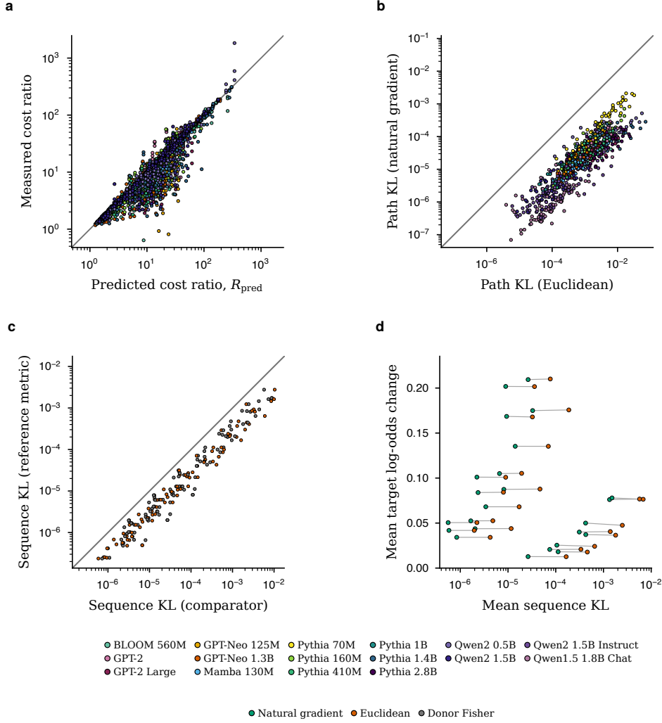
Figure 5: The geometry predicts intervention cost and supports reusable control. a , At matched behaviour change, the measured ratio of off-target output divergence for Euclidean versus damped natural-gradient updates is compared with the finite-damping prediction R_{\text{pred}} , which has no fitted parameters and is computed before intervention. The axes are logarithmic and the grey identity line denotes perfect agreement. Small circles show all 3,515 usable matched-response observations (of 3,564) from 1,188 model-objective-layer-context cells: 11 models, six families, three objectives, three relative layer depths and 12 contexts per objective, each measured at three intervention magnitudes (98.6% coverage; median measured-to-predicted ratio 0.967, 95% interval 0.957–0.975; log-log slope 0.982, 95% interval 0.966–0.997). b , Finite paths with both methods relinearised after every accepted step. All 864 points compare Euclidean and Fisher cumulative local KL at matched target changes, from 216 prompts, 16 models and 18 model-objective cells. The metric sums KL between successive accepted outputs. The 72 cell-target geometric-mean cost ratios span 11.5–127.1, with every paired 95% interval above one. Colours identify models in panels a and b. c , Reusable control on four base models from three families. All 192 points compare reference-Fisher sequence KL with Euclidean (vermilion) or donor-only Fisher (grey) sequence KL for the same reference continuation and matched donor change, across two objectives and three target changes. Each setting contributes four reference continuations per comparator. Reference sequences are teacher-forced continuations of the four prompts used to construct the reference metric. Ratios of mean Euclidean/reference-Fisher sequence KL span 2.90–6.29. d , The same updates change unseen target prompts without target gradients. Each point shows mean sequence KL over four reference continuations and mean target log-odds change (nats) over eight unseen prompts, for one model, objective, donor change and method (48 points). Green, natural gradient using the reference metric; vermilion, Euclidean. Grey segments join matched donor changes. All 24 natural-gradient mean target changes are positive. Grey diagonals in panels b and c mark equality.
