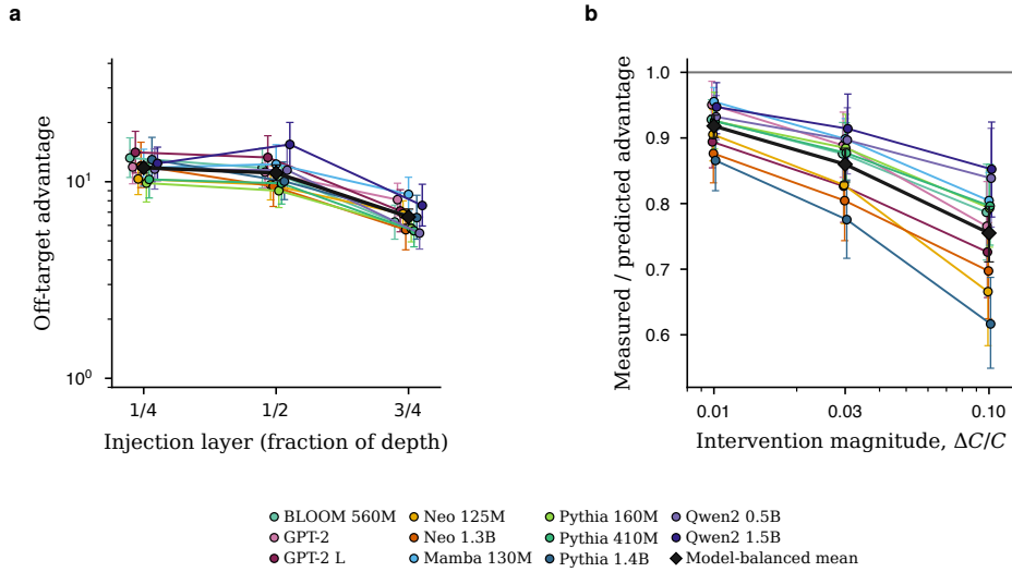
Extended Data Fig. 8 | Layer and intervention magnitude delimit the geometric correction. a , Off-target advantage by injection layer for 3,515 usable matched-response observations from 1,188 model–layer–objective–context cells across 11 models and six families, summarized as 33 within-model estimates. Coloured circles are geometric means and vertical bars are 95% paired objective–context–magnitude bootstrap intervals that preserve the available layer tuple; lines connect the three depths within model. Black diamonds are model-balanced geometric means with 95% model-bootstrap intervals. The pooled means fall from 11.79 to 11.08 to 6.62 at quarter, half and three-quarter depth, respectively. Every model mean is lower at three-quarter than at quarter depth; nine of eleven paths decrease at both adjacent steps, with one intermediate-depth increase for Mamba 130M and Qwen2 1.5B. b , Measured-to-predicted off-target advantage at intervention fractions \Delta C/C = 0.01, 0.03, 0.10 . Coloured circles are all 33 within-model geometric means (11 models crossed with three fractions), with 95% paired-cell bootstrap intervals; lines connect fractions within model. Black diamonds are model-balanced geometric means with model-bootstrap intervals, and the grey line denotes exact calibration. All 11 model paths decrease strictly. The model-balanced means are 0.918, 0.860 and 0.755, quantifying the expected attenuation of a local prediction as intervention magnitude grows.
