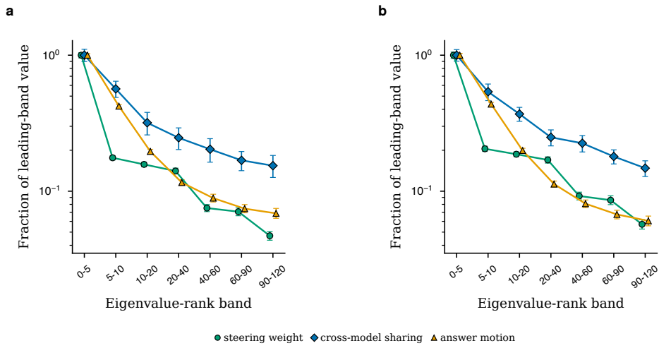
Extended Data Fig. 9 | Output sensitivity, cross-model sharing and answer motion concentrate in the same native-reference modes. Each panel shows all 21 summaries (seven predefined eigenvalue-rank bands \times three quantities) from six models: the band's eigenvalue-mass share, cross-model eigenvector sharing against the displacement-magnitude-matched null and probability motion on the highest-probability tokens. To compare their decay directly, each quantity and its 95% context-bootstrap interval are divided by that quantity's leading-band point estimate. On natural text the top five modes carry 55% of the eigenvalue mass, the largest residual sharing (+0.069, 95% interval 0.062–0.077) and the largest answer motion (0.59), all three decaying together to the last band. a , Natural-text battery. b , Templated battery.
