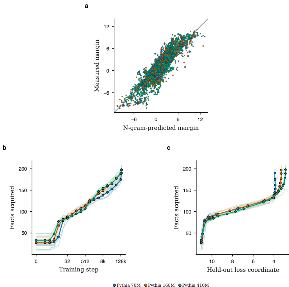
Figure 4: Corpus statistics predict acquisition across model sizes. a , Ex-ante corpus n-gram margins predict subsequent margins without refitting for fresh facts disjoint from calibration at Pythia 70M, 160M and 410M. Points are all 9,840 fact-checkpoint means over 15 checkpoints: 5,340 from 178 defined facts at 70M and 160M (ten runs) and 4,500 from 300 facts at 410M (nine runs); the shared model-colour key below the panels distinguishes Pythia 70M, 160M and 410M; the grey diagonal is exact prediction. Trajectory R^2 is 0.790, 0.792 and 0.775, persistent-status agreement is 0.792, 0.854 and 0.807, and continuous timing error is 0.77, 0.95 and 0.96 \log_2 training-step units, respectively. All three timing errors outperform their constant acquisition-time and label-permutation baselines. b , Cumulative acquisition curves for the same 300 facts against training step at 70M, 160M and 410M. Thin curves are individual seeds and heavy curves with circular markers are medians over nine seeds for each model size, using the shared model colours. c , The same curves against held-out loss. In the descriptive 70M-to-160M comparison, alignment by held-out loss has a median absolute error of 2.1 facts.
