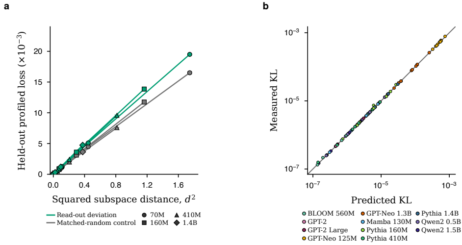
Figure 1: Behaviour identifies the resolved read-out, and geometry predicts local output change. a , Behavioural identification: held-out predictive loss after re-optimising nuisance parameters grows linearly with the squared subspace distance between a perturbed read-out subspace and the resolved subspace (Pythia 70M–1.4B). Markers are the 40 model–condition–angle means and bars span the two independently calibrated held-out folds (smaller than the markers); paths connect angles within each model and condition. Green, read-out deviation; grey, matched-random control; circles, 70M; squares, 160M; triangles, 410M; diamonds, 1.4B. The local fits have R^2 \geq 0.9999 on all eight paths, and matched-random control directions have systematically smaller loss–distance slopes (slope ratios 1.14–1.27). The reference subspace is estimated from a stronger model (Supplementary Note 3). b , Predicted and measured output change under small activation perturbations. Each point is one model–depth–prompt combination, giving 99 measurements across 11 models, six families and quarter-, half- and three-quarter-depth injection. The prediction \frac{1}{2}\delta h^\top G \delta h uses the metric before the intervention, without a fitted scale. Points show the coarsest resolved local steps; colour identifies the model and the grey line marks equality. The measured-to-predicted KL ratio has median 1.000 and range 0.948–1.224 (Methods; Supplementary Note 1).
