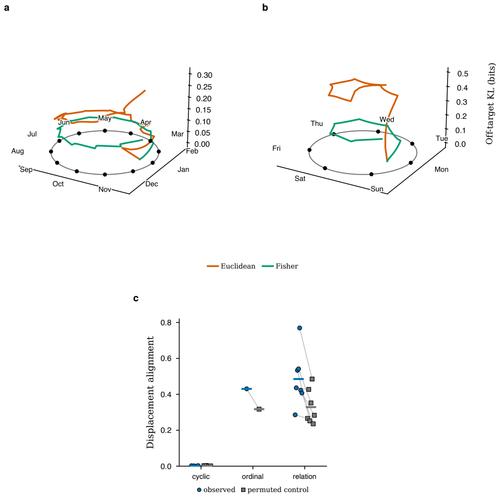
Extended Data Fig. 10 | Two geometries of behaviour: cyclic reweighting and relation-induced probability displacement (Pythia-410M). a,b , Walking the ring by steering month→month ( a ) or day→day ( b ) around the full cycle at matched concept progress: the plane is the concept's phase circle in output space and height is accumulated off-target change (bits). Both paths traverse the same ordered concept cycle; the reference phase sectors are separated, by construction, by 2\pi/12 (or 2\pi/7 ). After one circuit the endpoint returns towards the starting sector with a method-dependent residual displacement, while the natural-gradient path accumulates less off-target change. c , The dissociation from analogy relations. Paired circles and squares show probability-displacement alignment and its permuted control for all twelve concept sets across three categories (24 displayed values); thin grey lines join each concept's pair and short horizontal bars show category means. Relations move mass along a shared probability-displacement direction (mean alignment 0.49; permuted control 0.33), while cyclic concepts show none (0.00) and are near-isometries of the metric. The shared colour key applies to both trajectory panels.
