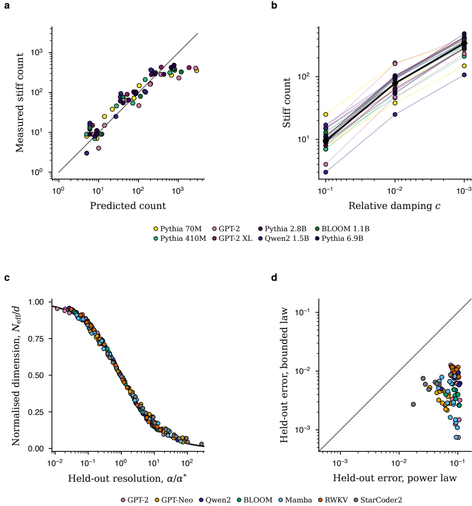
Extended Data Fig. 3 | Damping reveals bounded effective dimension. a , Predicted versus measured stiff-mode counts for 24 model–context spectra at relative damping 10^{-1} , 10^{-2} and 10^{-3} (72 points). Predictions are (1/c)^{1/\beta} from the power-law exponent fitted over ranks 2–80; colours identify the eight models, and the grey line denotes equality. b , All 72 resolved-mode counts, joined within each of the 24 spectra; colours identify models and black diamonds show the cross-spectrum median. The count grows as damping is lowered. The native-reference exponent is empirically stable across the tested models but is not an invariant of the metric alone. In held-out estimator validation, nominal 95% interval coverage is 0.90 for continuous effective dimensions and 0.85 for discrete threshold counts; primary dimension estimates therefore use the continuous form (Methods). c , Finite-size effective-dimension confirmation on 80 model–prompt curves spanning ten models and seven families. For each curve, a bounded effective-dimension curve was fitted at four fixed anchor dampings; points are all 240 observations at three interleaved, held-out dampings after rescaling by the fitted crossover \alpha^* . The black line is the bounded effective-dimension curve at the median fitted exponent. d , Curve-level held-out root-mean-square error for an equal-parameter unbroken power law (abscissa) and the bounded effective-dimension curve (ordinate). Every one of 80 points lies below equality. Median errors are 0.0814 and 0.00493, respectively; the median bounded-to-power error ratio is 0.0749 (95% crossed-bootstrap interval 0.0428–0.1234).
