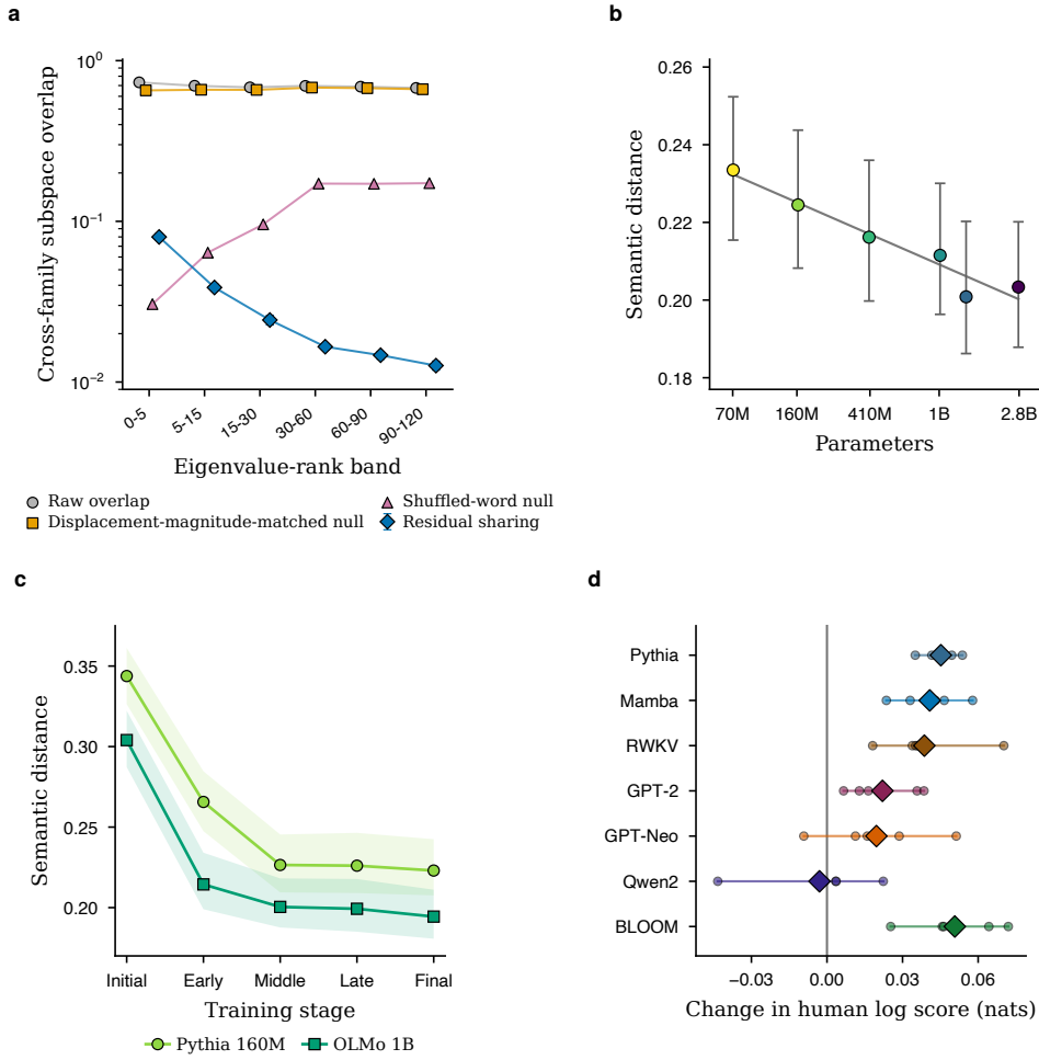
Extended Data Fig. 2 | Shared output structure beyond displacement magnitude and on independent human data. a , The 24 displayed estimates are six fixed eigenvalue-rank bands crossed with four summaries: raw subspace overlap (grey circles), a displacement-magnitude-matched null that preserves each word’s displacement magnitude (amber squares), a shuffled-word null (magenta triangles) and the residual above the displacement-magnitude-matched null (blue diamonds). Opaque markers have black borders; lines connect like summaries across bands. Error bars on the residual span the 2.5th–97.5th percentiles across 400 random 80%-context subsamples. Raw overlap is nearly flat, but the residual is concentrated in the leading modes and falls from 0.080 in ranks 0–5 to 0.013 in ranks 90–120. Thus about 89% of the leading-band raw overlap is explained by shared displacement magnitudes, while the smaller residual carries the rank-dependent cross-family structure. b , Native model samples on 640 word positions from five previously unused narratives. Points are the equal-story semantic distances for six final Pythia sizes; bars show conditional 95% bootstrap intervals and the grey line is the registered fit against log parameter count (slope -0.00872 , interval -0.01202 to -0.00556 ). c , The same distance at five ordered checkpoints from Pythia-160M and OLMo-2-1B. Lines show point estimates and shaded regions the conditional 95% intervals. Final-minus-initial changes are -0.12080 and -0.10962 , respectively. d , Expected human log-score change after applying the model-only source-trained full 65-outcome map instead of each model’s native law. Small circles show the five fixed-story differences and diamonds their equal-story means; positive values favour calibration. Six of seven family means are positive (0.0196–0.0507 nats); Qwen2 is -0.0030 nats. Panels b–d are conditional on the five observed stories and make no population-of-stories claim.
