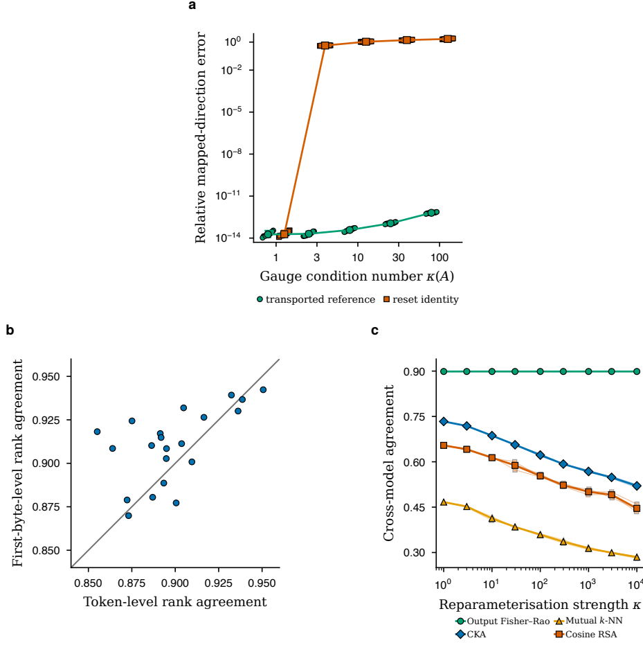
Extended Data Fig. 1 | Coordinate covariance and common-outcome controls. a , Coordinate covariance at finite damping. For 12 prompts under one seeded symmetric positive-definite gauge family with \kappa(A) = 1, 3, 10, 30, 100 , transporting the reference as R' = A^{-\top} R A^{-1} reproduces the native damped direction with mapped relative error at most 7.4 \times 10^{-13} (green circles). Installing a fresh identity instead changes the regularised problem: over non-identity gauges, the mapped-direction error has median 1.23 and minimum 0.54 (vermillion squares). Points, prompts; connected symbols, medians; error bars, 2.5th–97.5th percentiles. Pythia-410M, final pre-unembedding activation, top-512 output-Fisher support and \alpha = 0.01\lambda_{\max} . b , Pairwise output-geometry agreement before and after mapping each next-token law to its first-byte distribution (21 dyads among eight models). Aggregate agreement is 0.899 at token level and 0.910 after the push-forward; rank agreement between dyad-level values is 0.551. The grey line marks equality. c , Hidden-coordinate reparameterisation at nine anisotropy strengths and three seeds. Each point aggregates the same 21 model pairs; faint paths show seeds and heavy paths their means. Output Fisher–Rao agreement remains constant, while activation CKA, mutual nearest-neighbour overlap and cosine RSA degrade. Small horizontal offsets separate seeds.
