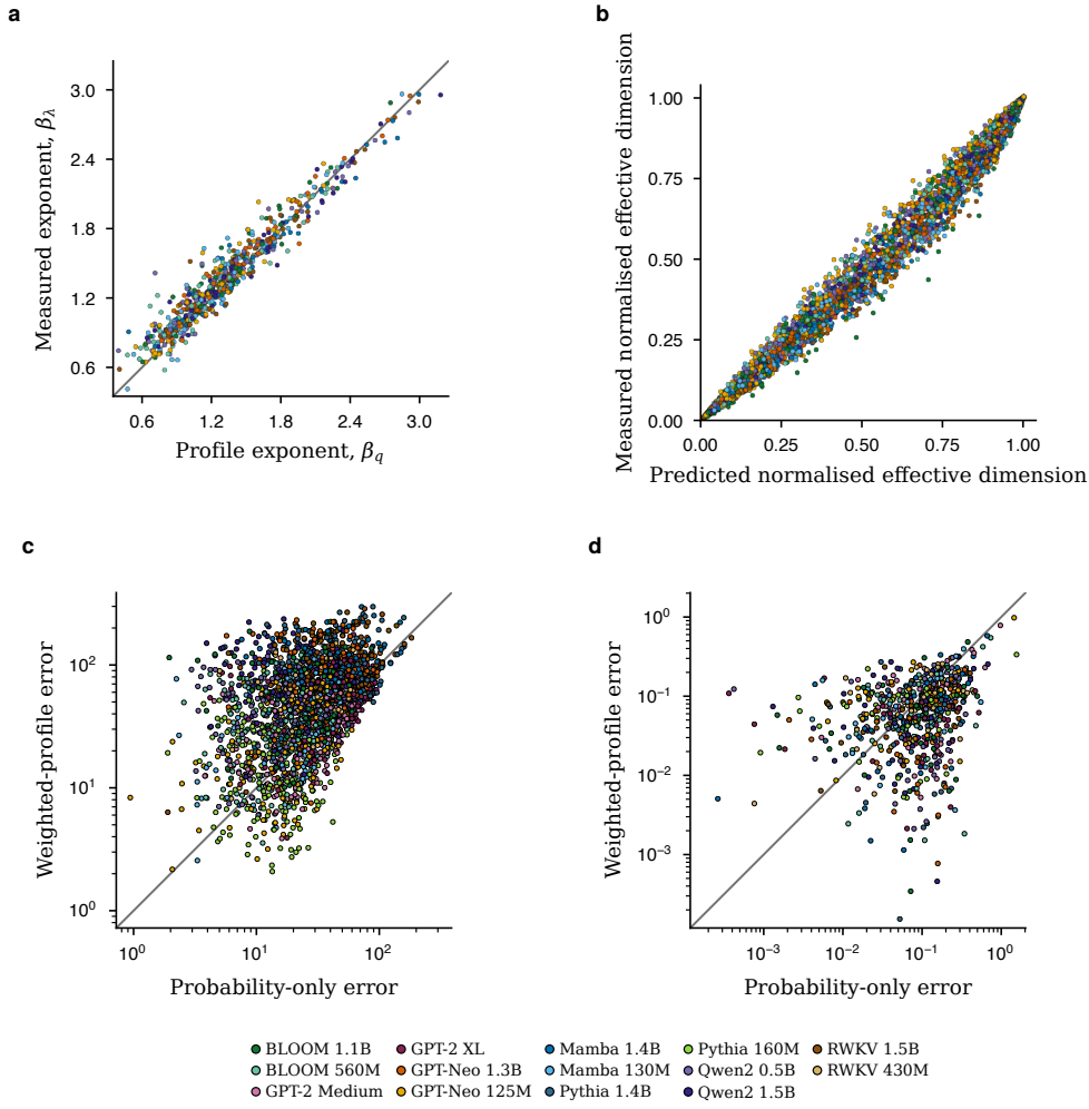
Figure 3: Language statistics shape the spectrum and its effective dimension. a , Profile-predicted against measured spectral exponent over ranks 8–32 for all 576 held-out model–context cells (nine models from five external families, 64 contexts per model). Small circles show every cell and the grey line is exact prediction. Colours identify models throughout the figure. The Pearson and Spearman correlations are 0.968 and 0.955; family-median absolute exponent errors are 0.0623–0.0856. On a matched 16-context-per-model control battery, spectral errors are 4.89–9.22-fold lower than for a same-trace flat spectrum and 13.55–25.63-fold lower than after shuffling profile ranks. b , Prediction of effective dimension without fitted parameters, the number of modes resolved at a given damping, from token statistics. Small circles show all 5,760 model–context–resolution values from the same 576 cells, coloured by model; the grey diagonal is exact prediction. No measured eigenvalue or fitted parameter enters the prediction. Family-median effective-dimension RMSEs are 0.0270–0.0521, 6.44–7.88-fold lower than for the same-trace flat-spectrum prediction. c , Effective-dimension prediction in a matched 14-model, seven-family comparison on 192 fresh contexts per model. All 2,688 points compare the weighted-profile and probability-only prediction errors on the same context, measured as effective-dimension RMSE across damping levels. The probability-only profile \hat{\lambda}_k = (r/V)p_{(k)} has lower family-median error in all seven families. d , All 672 paired spectral-exponent errors on the 48-context exact-spectrum subset per model; the weighted profile has lower family-median error in all seven families. Both panels use logarithmic axes, a common 27,450-outcome representation and the same standardised read-out; the grey diagonal marks equal error. Inference gives equal weight to families. Exact one-sided family sign-flip P = 1/128 for each contrast (Supplementary Note 6).
