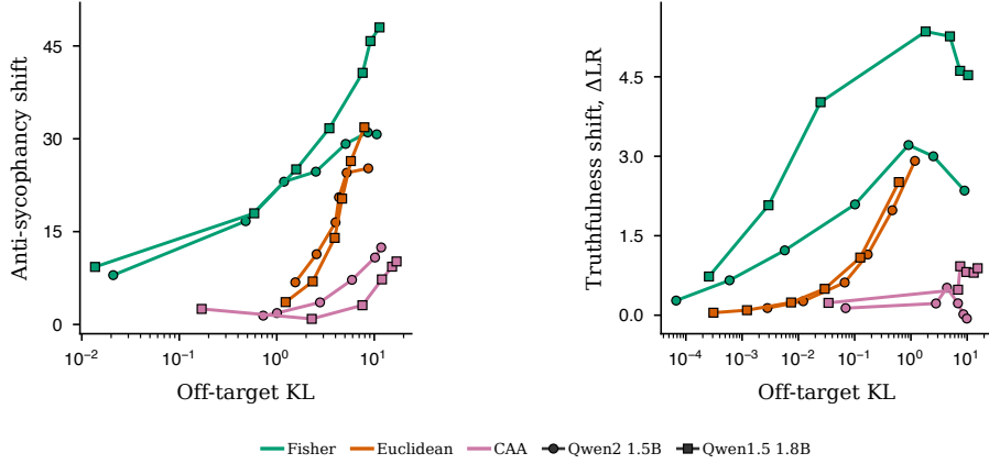
Supplementary Figure 2: Instruction-model control frontiers. Left, anti-sycophancy; right, capital-city truth preferences. Qwen2-1.5B-Instruct and Qwen1.5-1.8B-Chat each contribute the complete 19-point sweep: seven natural-gradient, six Euclidean-gradient and six contrastive-activation-addition settings. Cost is off-target KL on held-out neutral prompts; the horizontal coordinate is mean objective change. Interpolated comparisons match aggregate effects. The style and composition frontiers are shown in Extended Data Figure 5.
