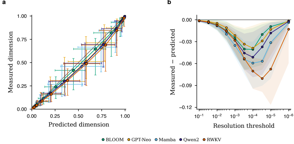
Supplementary Figure 1: Full calibration and residual structure of the token-profile effective-dimension prediction. a , All 5,760 model–context–resolution values from 576 model–context cells in the held-out battery are summarized as 50 family-by-resolution points. Opaque coloured circles with black borders compare family medians of the normalised effective dimension predicted from the sorted token profile with that measured from the exact spectrum; horizontal and vertical bars are the corresponding interquartile ranges, point–lines join the ten fixed resolution thresholds and the grey line is exact prediction. b , Measured minus predicted normalised effective dimension as the relative resolution threshold \alpha/q_{(1)} decreases from left to right. Lines are family medians and ribbons are interquartile ranges. The modest mid-resolution overprediction is resolved again at the coarse and fine endpoints.
