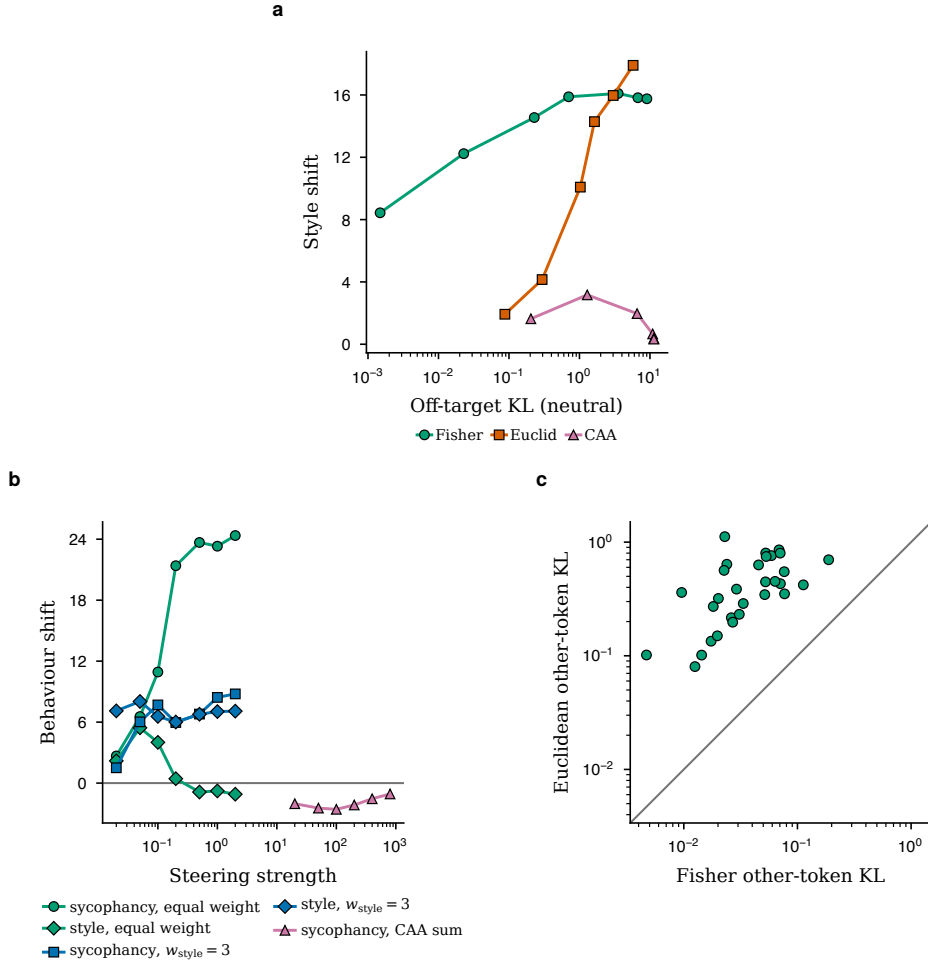
Extended Data Fig. 5 | Additional intervention trade-off curves, composition and fixed activation editing. a , The diffuse style objective: behaviour change against off-target change on neutral prompts. The complete 19-point operating sweep contains seven Fisher, six Euclidean and six contrastive-activation-addition (CAA) settings. b , Composition: sycophancy and style steered simultaneously by one solve on the weighted covector sum; varying the weight changes the balance between objectives, whereas summed CAA vectors change sycophancy in the opposite direction. The 20 distinct operating points produce 34 displayed objective outcomes; all markers are opaque with black borders. c , Matched fixed activation edits on 30 held-out CounterFact records (GPT-2). Each point compares Fisher other-token Kullback–Leibler (KL) divergence (abscissa) with Euclidean other-token KL divergence (ordinate) after both operators attained the same fixed +5 log-odds shift; axes are logarithmic and the grey line denotes equality. Euclidean cost is higher for all 30 edits, with a geometric-mean Euclidean-to-Fisher ratio of 10.57 (95% interval 8.52–13.37).
