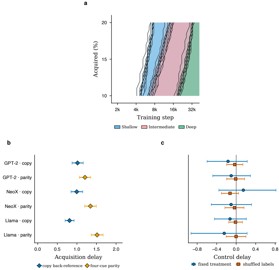
Extended Data Fig. 4 | Evidence depth delays acquisition across architectures and evidence constructions. a, Randomised evidence depth delays persistent acquisition. Curves follow the 10th–20th acquisition-time percentiles for each of 12 training seeds of the same transformer, pooling over the same facts and probes within each seed. Black curves show individual seeds; blue, pink and green shading to their right marks acquisition levels already reached under shallow, intermediate and deep evidence, respectively. The pooled deepest-versus-shallowest shift is \Delta = 2.10 \log_2 training-step units (crossed seed-by-quintet bootstrap 95% interval 1.79–2.40), equivalent to 4.3 \times more training steps; the deepest-versus-intermediate contrast is smaller. b, Mean paired delay in persistent acquisition for evidence assigned to the deep construction relative to otherwise matched evidence in the shallow construction, crossing GPT-2-, GPT-NeoX- and Llama-style decoders with copy-back-reference and four-cue-parity controlled languages. Blue diamonds denote copy-back-reference cells and amber diamonds four-cue-parity cells; horizontal lines are 95% crossed seed-by-matched-block bootstrap intervals around the cell means over eight seeds and 384 matched fact blocks per cell. All six intervals and all 48 seed means are positive; effects span 0.810–1.514 \log_2 training-step units (1.75–2.86-fold in training steps). The equal-family mean parity-minus-back-reference contrast is 0.414 \log_2 training-step units (95% interval 0.291–0.536). c, Corresponding fixed-treatment (blue circles) and label-randomisation (vermillion squares) controls. Every one of the twelve 95% intervals contains zero. The grey vertical line in panel c marks zero delay; delays are in \log_2 training-step units.
