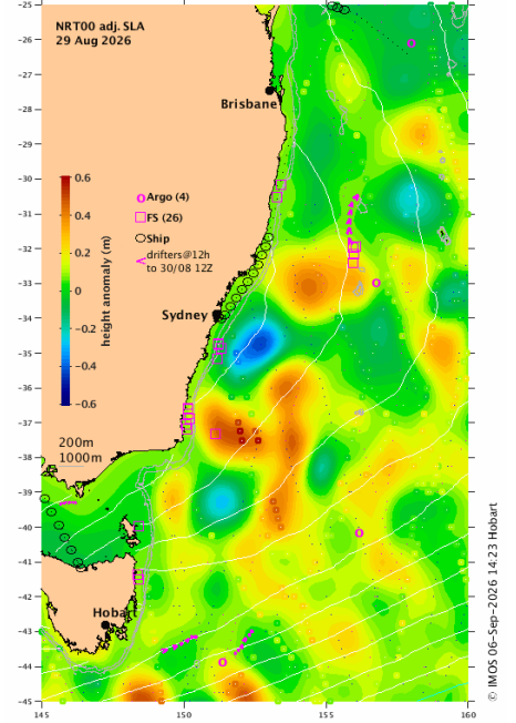
Figure 7: Visualisation of the GSIA analysis provided by IMOS (2026). This ground truth SLA field is obtained using a range of observational data as shown, beyond satellite altimetry.
