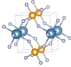
(a) \text{CaAuF}_5 \text{Ca}^{2+} \text{ Au}^{3+} \text{ F}^-
