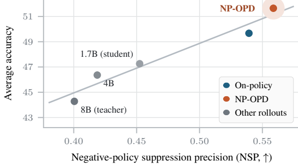
Figure 2: Negative-policy suppression precision (NSP) for OPD and different rollout policies. NP-OPD with a lower-capability rollout policy than the student yields higher NSP and higher reasoning performance, while using higher-capability rollouts decreases accuracy.
