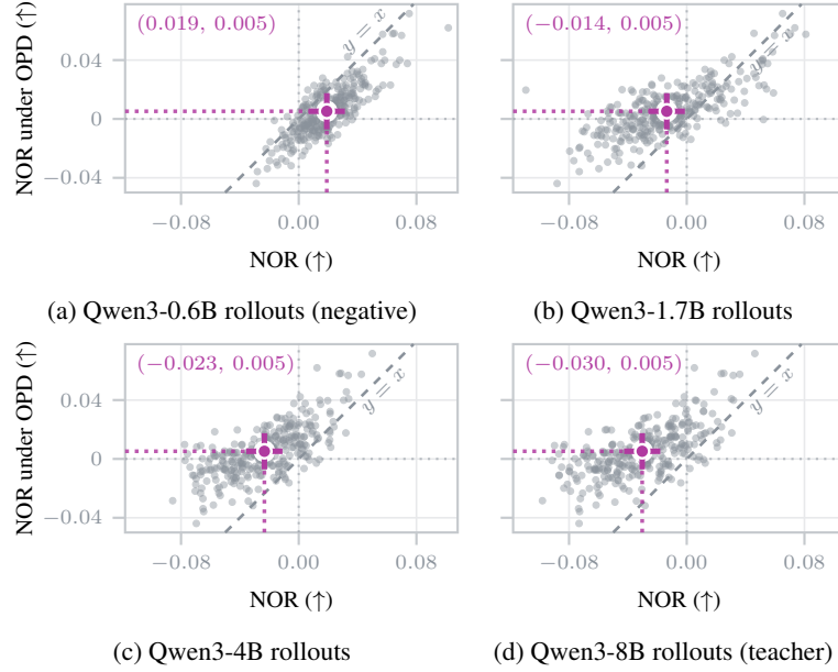
Figure C.1: Reduction in overlap across rollout policies. Same quantity as Fig. 4, with the rollout policy varied over the Qwen3 family: (a) 0.6B (negative policy), (b) 1.7B, (c) 4B, and (d) 8B (teacher). Each point compares trajectory-level NOR under OPD (y-axis) with NOR under the corresponding rollouts (x-axis). Only 0.6B rollouts place most trajectories below the diagonal and the paired gap decreases monotonically with the size of the rollout policy.
