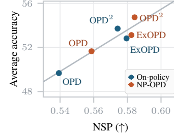
Figure 5: NSP across OPD variants. Each pair compares on-policy training with NP-OPD for three formulations; OPD, ExOPD, and OPD 2 .
