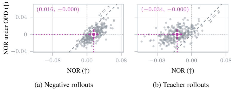
Figure C.2: Reduction in overlap with the negative policy on held-out prompts. Same quantity as Fig. 4, measured on 300 held-out prompts drawn from nine benchmarks spanning mathematics, science, and code, none of which appear in training. Each point is one trajectory, comparing NOR under OPD (y-axis) with (a) negative-policy or (b) teacher rollouts (x-axis).
