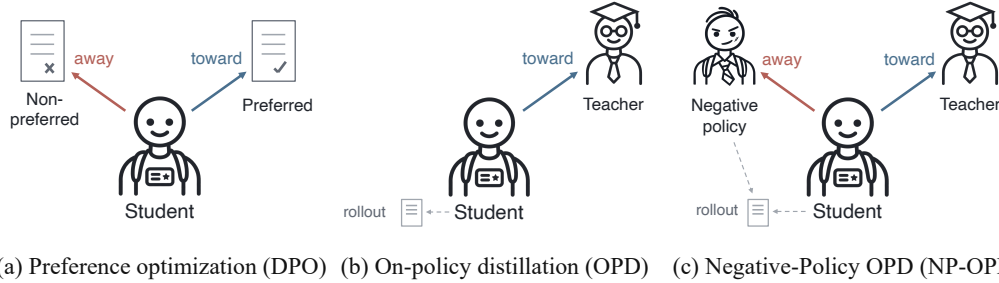
Figure 1: Conceptual comparison of preference optimization, on-policy distillation (OPD), and Negative-Policy OPD (NP-OPD). (a) Preference optimization provides both toward and away directions through preferred and non-preferred responses, whereas (b) OPD provides an explicit positive direction through teacher supervision but no explicit negative reference indicating what the student should move away from. (c) NP-OPD complements the positive signal from teacher supervision with rollouts from a lower-performing, lower-capability negative policy that serves as a negative reference. Here, “negative” refers to the role of the negative policy as a reference from which the student is intended to move away. In our main setting, the negative policy is selected from the same model family as the student with lower model capacity and overall reasoning performance.
