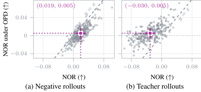
Figure 4: Reduction in overlap with the negative policy. Each point compares trajectory-level NOR under OPD (y-axis) and (a) negative-policy or (b) teacher rollouts (x-axis). Points below the diagonal indicate greater overlap reduction.
