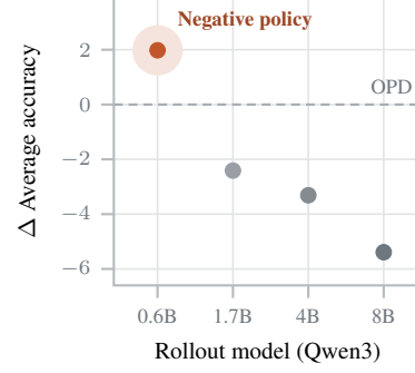
Figure 3: Role of lower-capability rollouts. When changing the rollout policy, only Qwen3-0.6B, a negative policy under our definition, improves over OPD.
