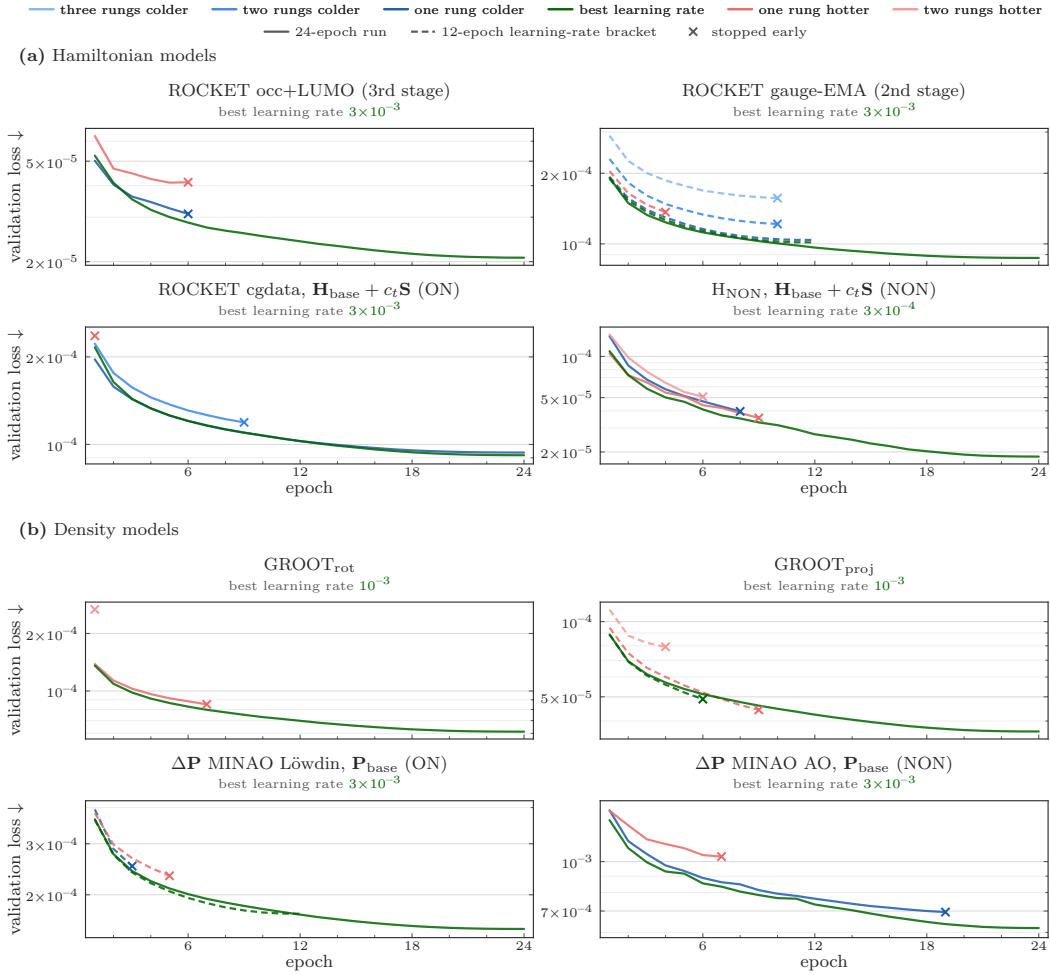
Figure 10: Validation-loss trajectories for learning-rate selection on QMugs. (a) Hamiltonian models. (b) Density models. Each panel reports the selected learning rate above the axes and colors the remaining rates by their position on the sweep. Solid lines show 24-epoch runs, dashed lines show 12-epoch brackets, and crosses mark runs that stopped early. Completed 24-epoch runs take 35–39 h on one NVIDIA H200 GPU, or about 1.5 h per epoch.
