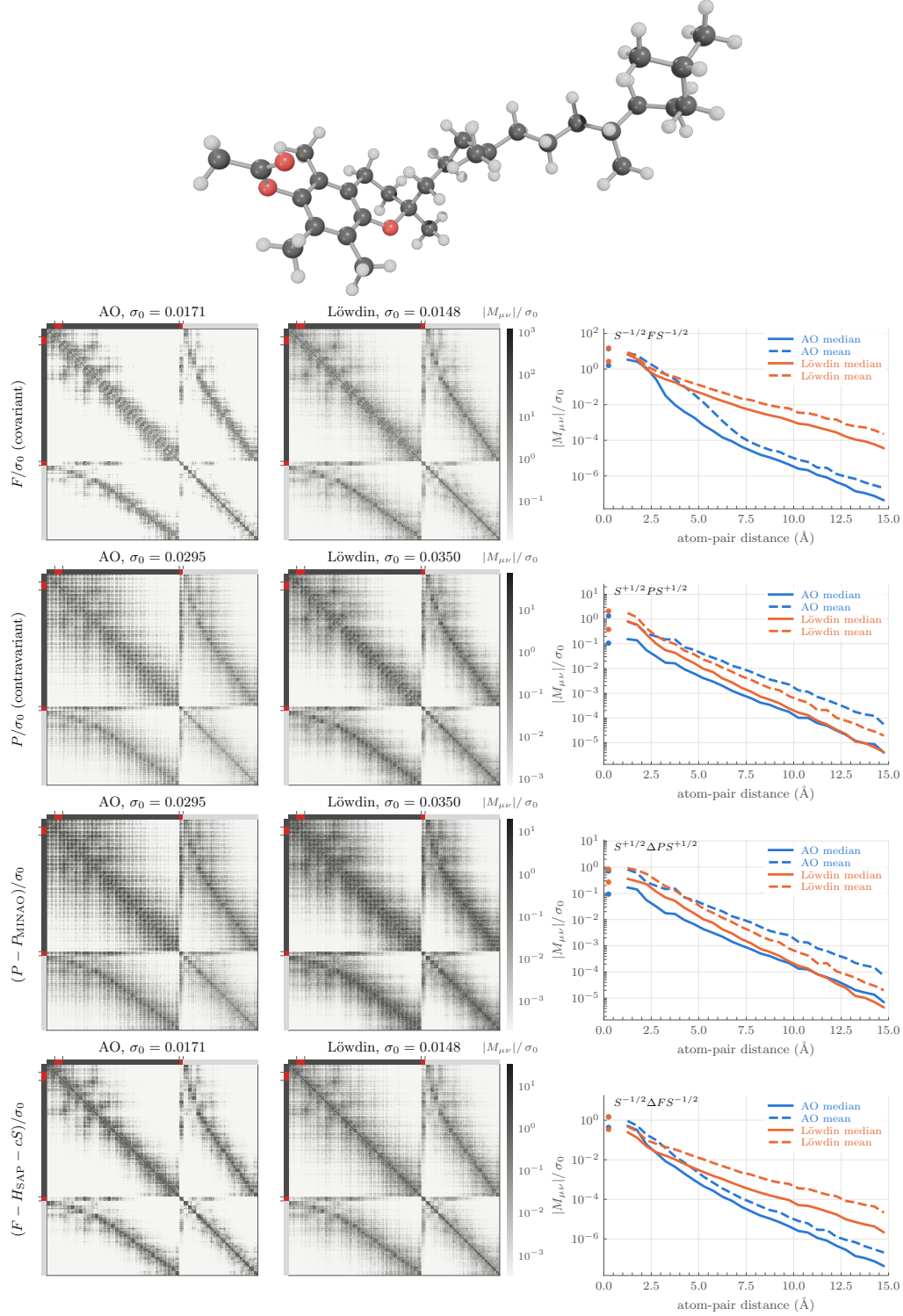
Figure 6: AO versus Löwdin spatial decay for QM40 molecule 68311 at B3LYP/def2-SVP. Columns are \mathbf{H} , \mathbf{P} , \mathbf{P} - \mathbf{P}_{\text{MINAO}} , and \mathbf{H} - \mathbf{H}_{\text{SAP}} - c\mathbf{S} , each in the AO (a.k.a. NON) basis and after Löwdin orthogonalization, scaled by the dataset root-mean-square (RMS) \sigma_0 . AO entries decay with atom-pair distance. Löwdin entries remain large after the AO entries have dropped.
