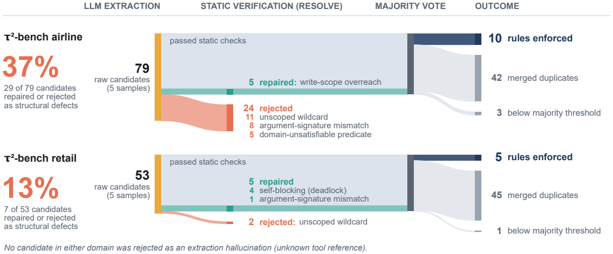
Figure 2: From extracted candidates to enforced rules (Table 3). Static verification repairs or rejects 37% of raw candidates on airline (29 of 79) and 13% on retail (7 of 53) as structural defects; repaired candidates proceed to the vote. The rejected counts sum the table’s rejection rows (airline: unscoped wildcard, argument-signature mismatch, domain-unsatisfiable predicate; retail: unscoped wildcard); the retail argument mismatch strips bindings from a candidate that survives and is shown as a repair. Duplicates then merge and minority candidates drop out, leaving 10 and 5 enforced rules.
