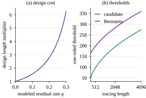
Fig. 2: Tracing design and certification are separate. (a) Inverse-square length multiplier for a hypothetical independent residual flip channel. (b) Candidate and Bernstein-certified one-sided thresholds versus tracing length, at c = 2 , N = 10 , and \varepsilon_1 = 10^{-3} . The certified threshold does not assert completeness.
