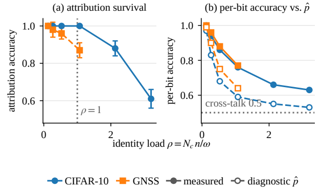
Fig. 3: Attribution versus identity load from Table III ( n=128 , \omega=4800 , R=100 , 10-seed). (a) Attribution accuracy against \rho=N_c n/\omega , error bars one std. Dotted: rank reference \rho=1 . (b) Measured per-bit self-agreement (filled, solid) and the diagnostic \hat{p}=\Phi(\text{SNR}_{\text{quad}}) of (6) (open, dashed). Dotted: chance agreement 0.5.
