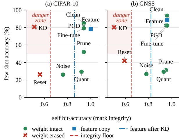
Fig. 5: Accuracy–integrity tradeoff under the weight-carrier attacks of Table X: (a) CIFAR-10, (b) GNSS. x -axis: self bit-accuracy ( \approx 0.5 = codeword erased). y -axis: few-shot accuracy. Shaded: high accuracy with the codeword at chance. Square: clean feature-carrier copy. Dash-dot: its bit-accuracy after the same 80-epoch distillation.
