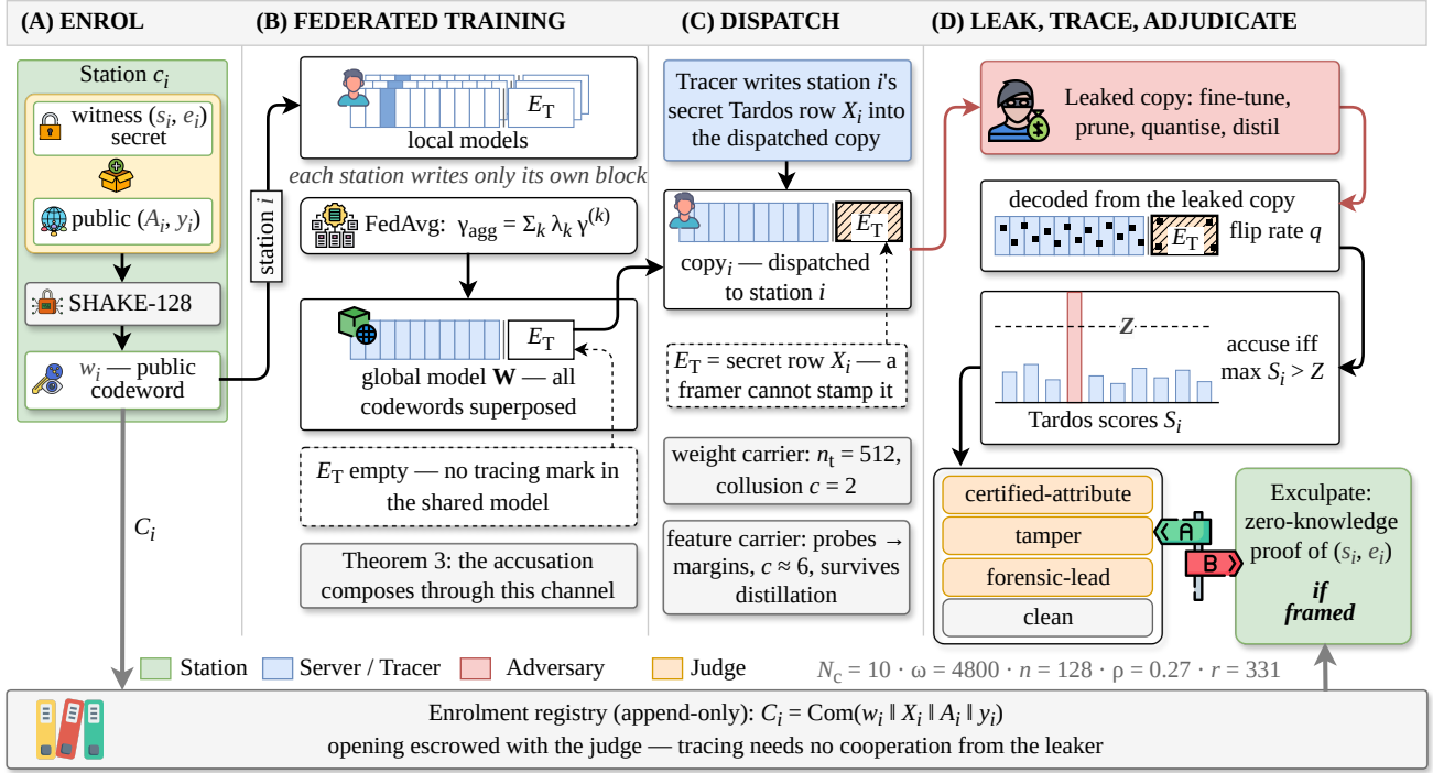
Fig. 1: ZK-Trace life cycle and carrier layout. The bar is the projection codebook read from the batch-normalization scales \gamma , partitioned into per-client identity blocks E_1, \dots, E_{N_c} and the tracing overlay block E_T . Solid cells carry the public codeword w_i , hatched cells the tracer-secret Tardos row X_i . S_i is the Škorić-symmetric score, Z the accusation threshold, and q the per-bit flip rate induced by aggregation.
