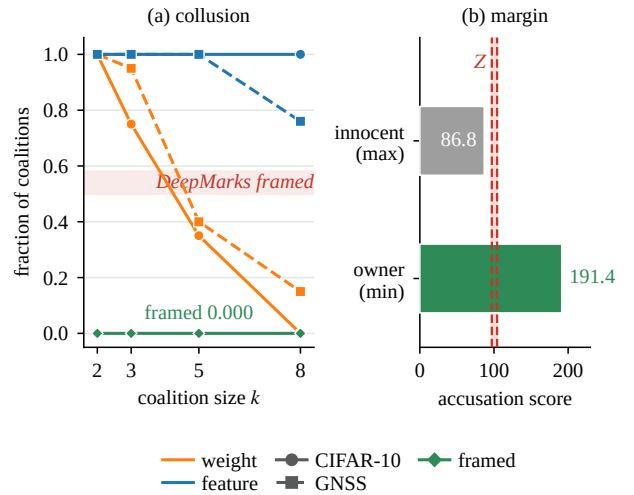
Fig. 4: Collusion tracing and the accusation margin. (a) Fraction of sampled coalitions traced, and the fraction in which any innocent is framed, against coalition size k for both carriers and datasets (Table V). Color keys the carrier, marker and line style the dataset. Shaded band: the DeepMarks-BIBD framing rate, whose traceability is not plotted. (b) Largest measured innocent score and smallest owner score over the realized decodes. Shaded band: the accusation threshold Z = \sqrt{2n_t \ln(N/\epsilon_1)} over the deployed federation sizes.
