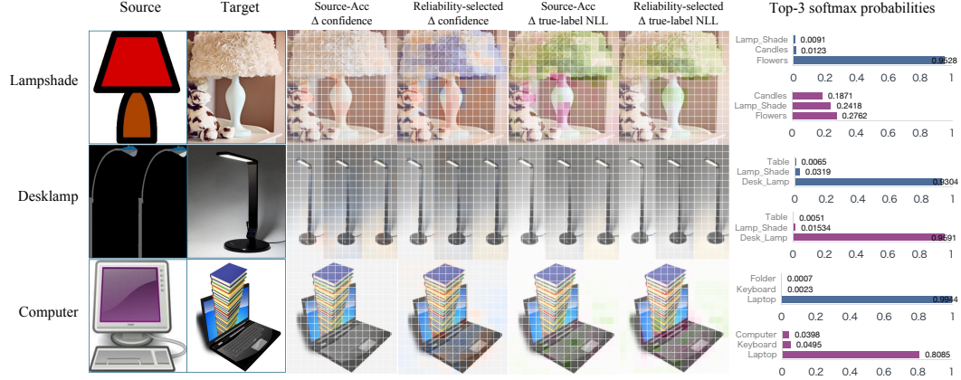
Figure A.1: Target-domain examples comparing Source-Acc and reliability-selected checkpoints. The left columns show a source-domain class exemplar and a target image. Each heat map masks one 16 \times 16 patch: \Delta confidence is the decrease in top-1 probability (purple: support for the prediction; blue: counter-evidence), whereas \Delta true-label NLL is the increase in true-label loss (green: support for the true class; magenta: conflicting evidence). Colors are comparable within a metric, not between metrics. Right-hand bars show the three largest softmax probabilities.
