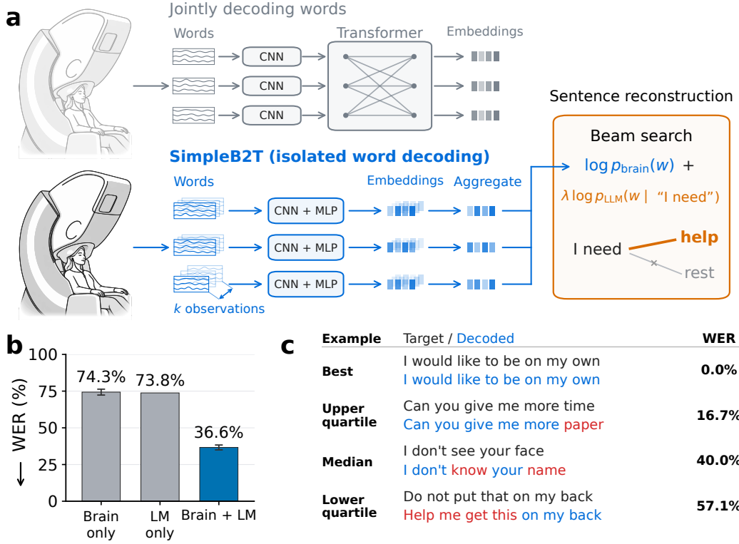
Figure 3: SimpleB2T. (a) Instead of jointly decoding words, we decode each neural response independently. We also test the effect of aggregating responses from distinct observations and using an LLM with beam search for sentence decoding. (b) Combining predictions with an LLM substantially reduces WER. (c) Decoded examples. Results are on our core set of 100 clinical sentences with k = 5 observations per word. Error bars indicate \pm 1 standard deviation across five training seeds.
