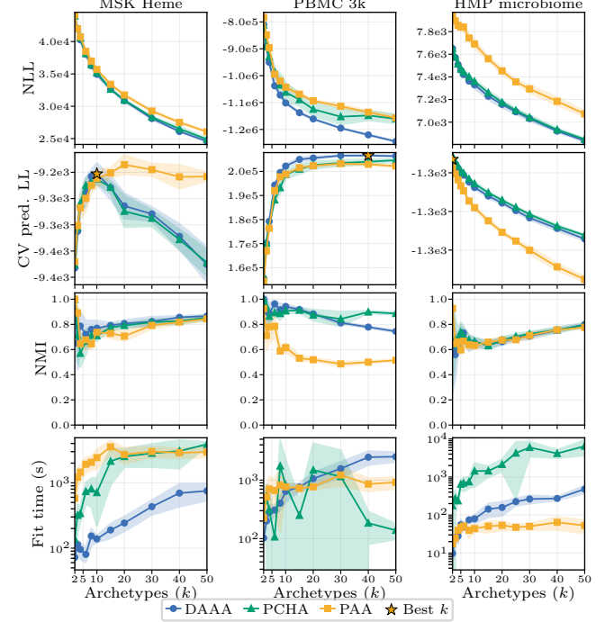
Fig. 4: Real-data benchmarks across three datasets and distributions. Each column corresponds to one dataset (MSK Heme, Bernoulli; PBMC 3k, Poisson; HMP microbiome, Multinomial) and each row to one metric: training loss (NLL), cross-validated predictive log-likelihood (star marks the DAAA selected K ), stability NMI across random initialisations, and wall-clock fit time. DAAA uses max_active = 25% of samples. PCHA and PAA use the full dataset. Shaded bands denote \pm 1 standard deviation across five random seeds.
