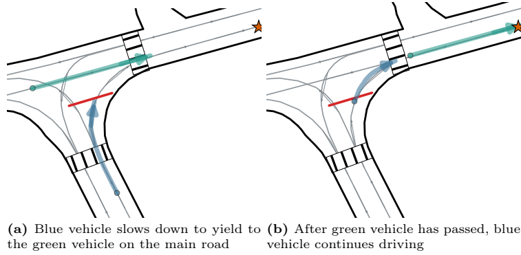
Fig. 7: Example of a synthetic scenario containing a stop line and the trajectories taken by agents. Yellow star shows the position of the waypoint for both agents.
