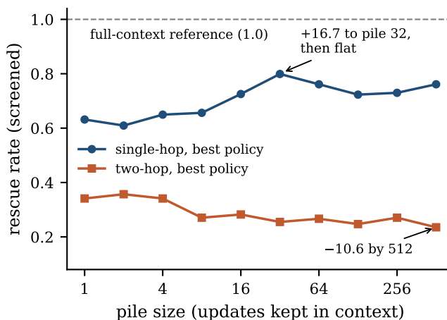
Figure 6: Rescue rate against pile size for each question tier’s best text policy, near-identical regime, both tiers swept at all ten pile sizes (screened scale, with single-hop n = 448 and two-hop n = 255 ). Single-hop rises to a plateau at pile size 32, with 32 against 512 inside its MDE. Two-hop never gains and ends 10.6 points below its pile-1 value. The winning policy differs by tier, an ordered paste against tuned retrieval, so the curves compare each tier to its own baseline rather than tier to tier.
