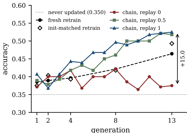
Figure 4: Chain accuracy by generation at three replay fractions, against the fresh retrain and the initialization-matched retrain recomputed at generations 1, 2, 4, 8, and 13, with the never-updated base as the floor. The chains cannot be told apart through generation 4 and end 15.0 points apart at generation 13, and the no-replay chain ends level with never updating. Nearly every chain-to-ceiling gap is smaller than its cell can distinguish, and the one exception is the no-replay chain at generation 13.
