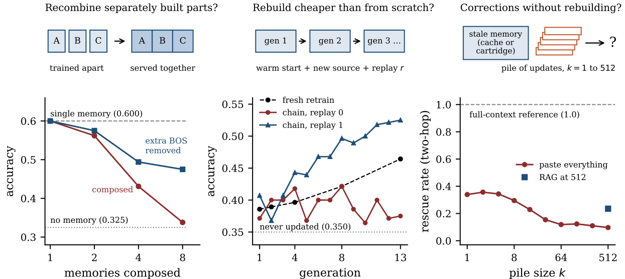
Figure 1: The three questions. Left, build time: separately trained memories are concatenated at serving time, and accuracy falls with the number of memories composed. Removing the duplicated start-of-text columns recovers about half the fall (Section 4). Middle, build time: one evolving memory is rebuilt warm as sources accumulate, and replay of the earlier sources’ training data is what separates chains that track a fresh retrain from chains that decay to the never-updated floor (Section 5). Right, query time: an already-built memory is served together with a pile of updates. On two-hop items, use of the correction falls as revisions accumulate, and no delivery policy comes within 64 points of the full-context reference (Section 6).
