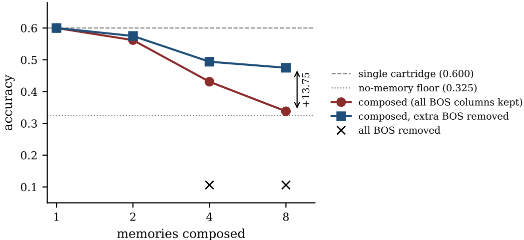
Figure 3: Accuracy under composition. The item-matched single-cartridge baseline holds 0.600. The composed memory falls with the number of memories. The same memory with extra BOS columns removed recovers about half the fall, and removing every BOS column collapses the memory to 0.106, below the no-memory floor. Removing an ordinary column instead of a BOS column (not shown) changes nothing.
