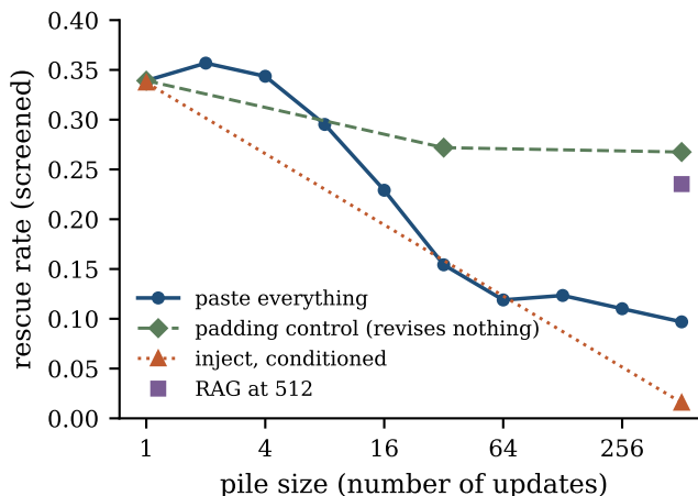
Figure 5: Rescue rate against pile size on a log axis. Pasting everything falls as real revisions accumulate, and the same pile sizes padded with token-matched sentences that revise nothing fall far less, so most of the fall is caused by what the sentences say. The padding series is a control rather than a deployable policy, since it removes the competing revisions a real pile contains, which is why it can sit above every policy at 512. Conditioned injection collapses fastest, and tuned retrieval is the best policy endpoint at 512. The plotted series come from different launches, each under its own screen, so endpoints differ from Table 3 by less than half a point.
