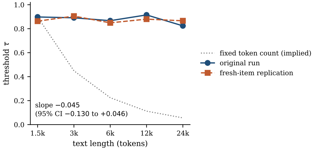
Figure 8: The threshold \tau against text length on a log axis, both runs. The dotted curve is the fall a fixed token count would imply, anchored at the shortest length’s measured threshold, 0.898 \times 1,500 \approx 1,350 tokens. The fitted slope of the measured thresholds is -0.045 (95% CI -0.130 to +0.046 ), consistent with a constant fraction over the tested range.
