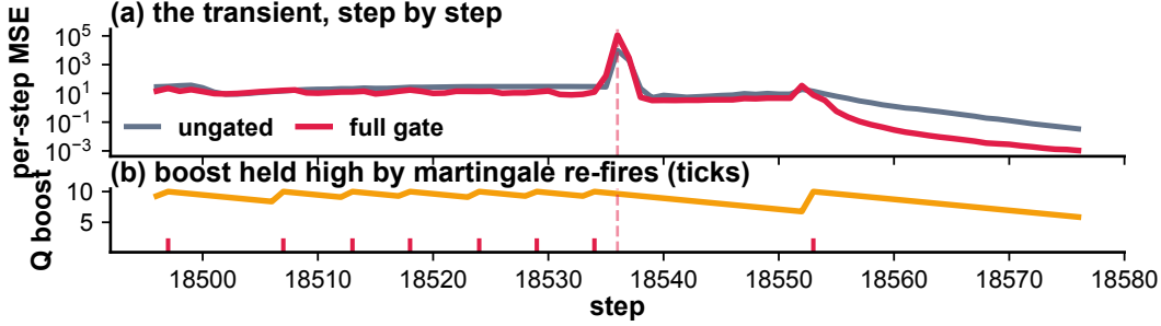
Figure 2: Single-step trace around the natural weather transient (clean stream, TimesFM 2.5, seed 0). (a) Per-step MSE: the full gate (red) tracks the ungated filter until the event, then exceeds it by 12\times . (b) Q -boost multiplier with fire ticks (8 plotted of 264): re-fires hold an 8 to 10\times boost active at the event.
