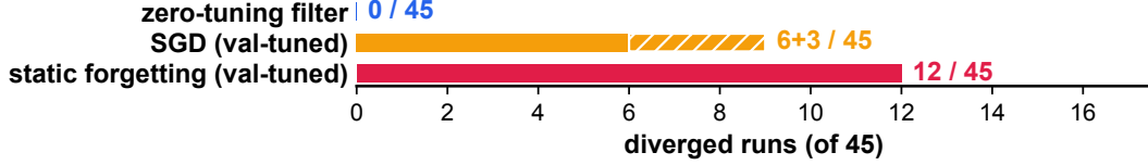
Figure 1: Clean-stream divergences per learner across the 45 staged-study runs (5 datasets \times 3 backbones \times 3 seeds). Hatching marks de facto divergences the magnitude guard missed (SGD on traffic under TimesFM 2.5, cumulative MSE 7.97 against the committed threshold of 5, no guard flag, in all three seeds).
