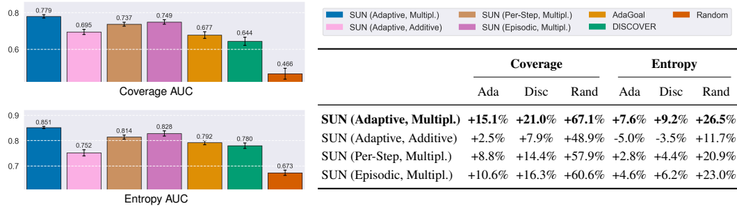
Figure 8: (Left) Area under the curve (AUC) for entropy and coverage across all baselines and SUN versions, averaged over all environments (excluding LunarLander (Full)). (Right) Relative AUC improvement of each SUN version over AdaGoal, DISCOVER, and Random.
