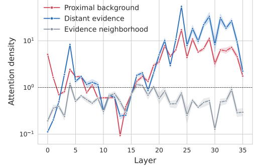
Figure 2: Distant Evidence is selectively retrieved but still diluted by cumulative competition from proximal background. We report layer-wise attention density for distant evidence, its neighboring tokens, and proximal background near the query.
