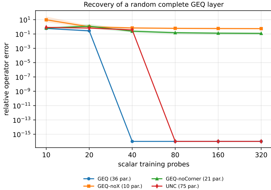
Figure 2: Recovery of a random complete groupoid-equivariant layer from scalar bilinear probes. Curves show medians over 40 independent targets.
