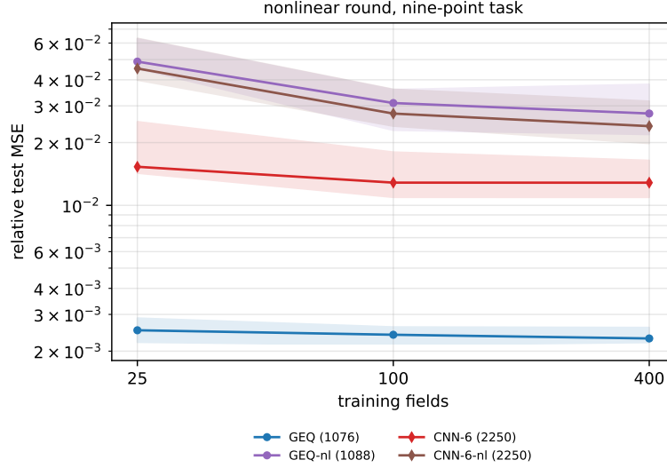
Figure 4: Nonlinear-round results on the nine-point Poisson-Dirichlet task. Median relative test MSE is shown as a function of the number of training fields, with shaded interquartile ranges. GEQ-nl and CNN-6-nl denote the nonlinear counterparts of GEQ and CNN-6, respectively.
