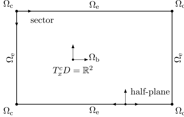
Figure 1: The tangent-cone stratification of a rectangle. The ordinary restricted groupoid has one object orbit, whereas \Gamma_D^{\text{tc}} has bulk, edge, and corner orbits.
