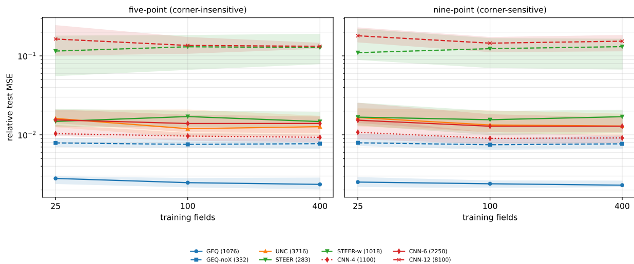
Figure 3: Sample-efficiency curves for the Poisson–Dirichlet benchmark.
