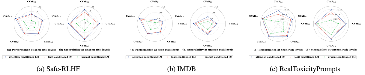
Figure 3: Comparison of different conditioning mechanisms across CVaR risk levels on three benchmarks.
