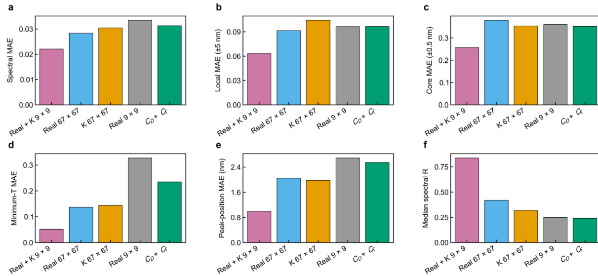
Supplementary Fig. S6 | Expert-input ablation. The five inputs are the central 9 \times 9 complex Fourier block (Real + K 9 \times 9 ), the full real-space map (Real 67 ), the full Fourier tensor (K 67 ), a central 9 \times 9 real-space crop (Real 9 \times 9 ) and the scalar pair C_D + C_T . a–f, Complete-spectrum MAE, \pm 5 nm local MAE, \pm 0.5 nm core MAE, minimum-transmission MAE, resonance-position MAE and median spectral R . Single seed, strict split.
