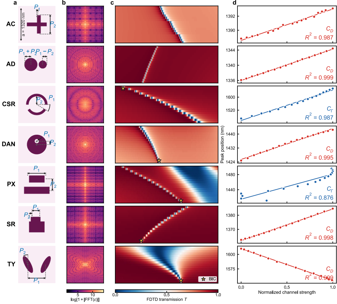
Fig. 2 | Seven qBIC metasurface families on a shared Fourier grid. a, Unit cells and geometric parameters P_1 and P_2 (lattice period a = 1,320 nm). b, Log-amplitude of the dielectric Fourier coefficients of representative structures. c, Raw transmission spectra along one parameter slice of each family (horizontal axis, wavelength; vertical axis, scanned parameter); stars mark the symmetry-protected BIC. d, Resonance position versus the normalized descriptor, C_T for CSR and PX and C_D for the other families. Each slice contains 17 points; R^2 is given for the slice shown.
