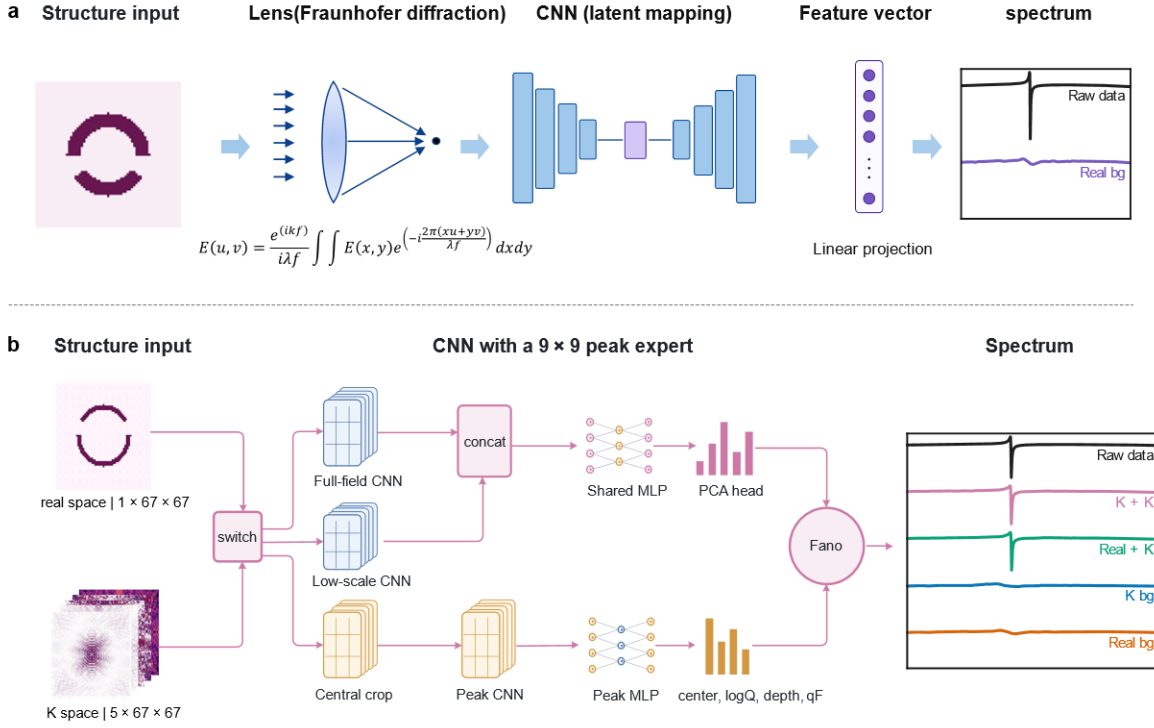
Fig. 1 | Dielectric Fourier-space framework for qBIC spectral learning. a, Conventional route, in which a CNN maps the real-space permittivity map to the spectrum. Fraunhofer diffraction by a lens is shown as the familiar optical example of a Fourier transform. b, Model used in this work. The background backbone receives either the real-space map or the five-channel Fourier tensor (tested separately) and predicts the broadband spectrum through a PCA head. The optional resonance expert receives the central 9 \times 9 Fourier block and predicts the resonance centre, \ln Q , depth and Fano asymmetry, which a differentiable Fano layer adds to the backbone spectrum. Right, representative predictions of the four configurations.
