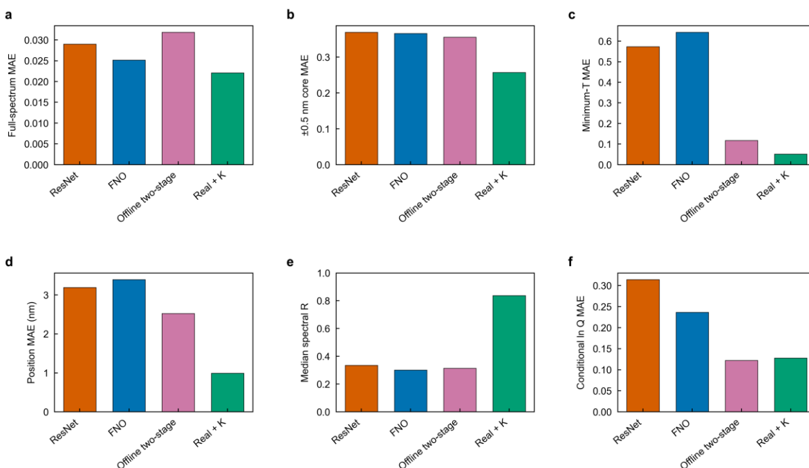
Supplementary Fig. S7 | Additional surrogate-model comparison. a–f, Complete-spectrum MAE, \pm 0.5 nm core MAE, minimum-transmission MAE, resonance-position MAE, median spectral Pearson R and conditional ln Q MAE. All models use the same 221 strict-test samples and seed 20260717. The ln Q error is conditional on both spectra being resolvable; each model uses its respective resolvable intersection. Bars are single-seed results without uncertainty estimates.
