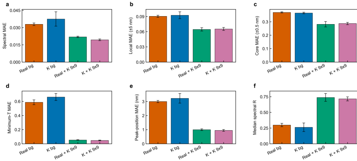
Supplementary Fig. S5 | Five-seed test metrics for the four forward models under the strict split. a–f, Complete-spectrum MAE, \pm 5 nm local MAE, \pm 0.5 nm core MAE, minimum-transmission MAE, resonance-position MAE, and median spectral R, respectively. Bar heights are five-seed means, error bars are sample standard deviations, and the test set contains 221 samples.
