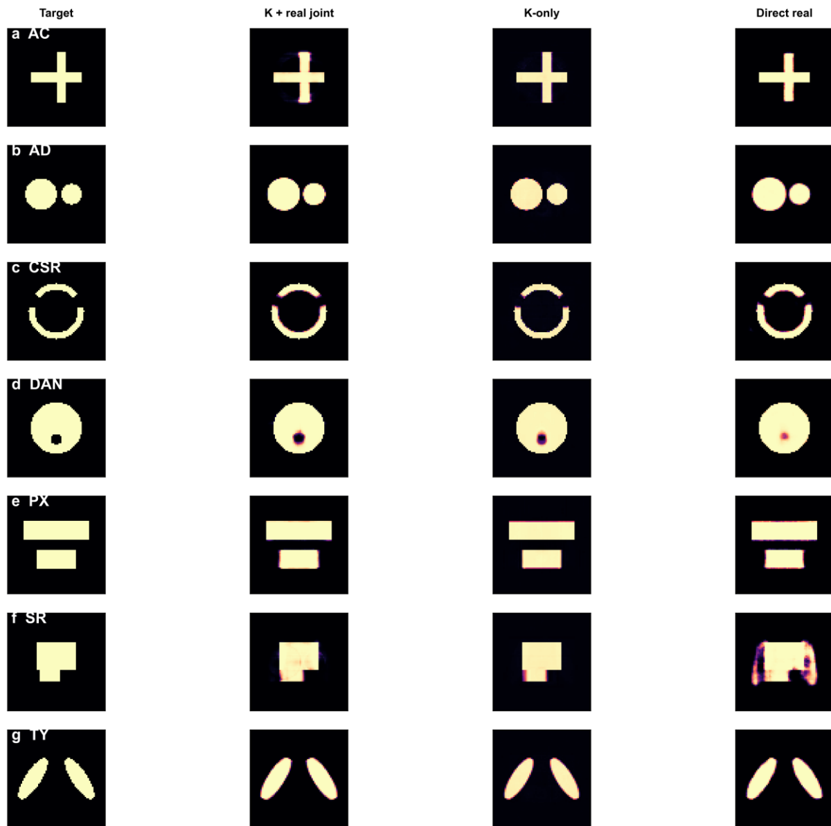
Supplementary Fig. S11 | Inverse reconstruction of representative test samples from the seven structure families. Each row corresponds to one family; columns compare the ground-truth dielectric distribution with K + real joint, K-only, and Direct real. Predicted maps show unthresholded foreground probabilities from 0 to 1.
