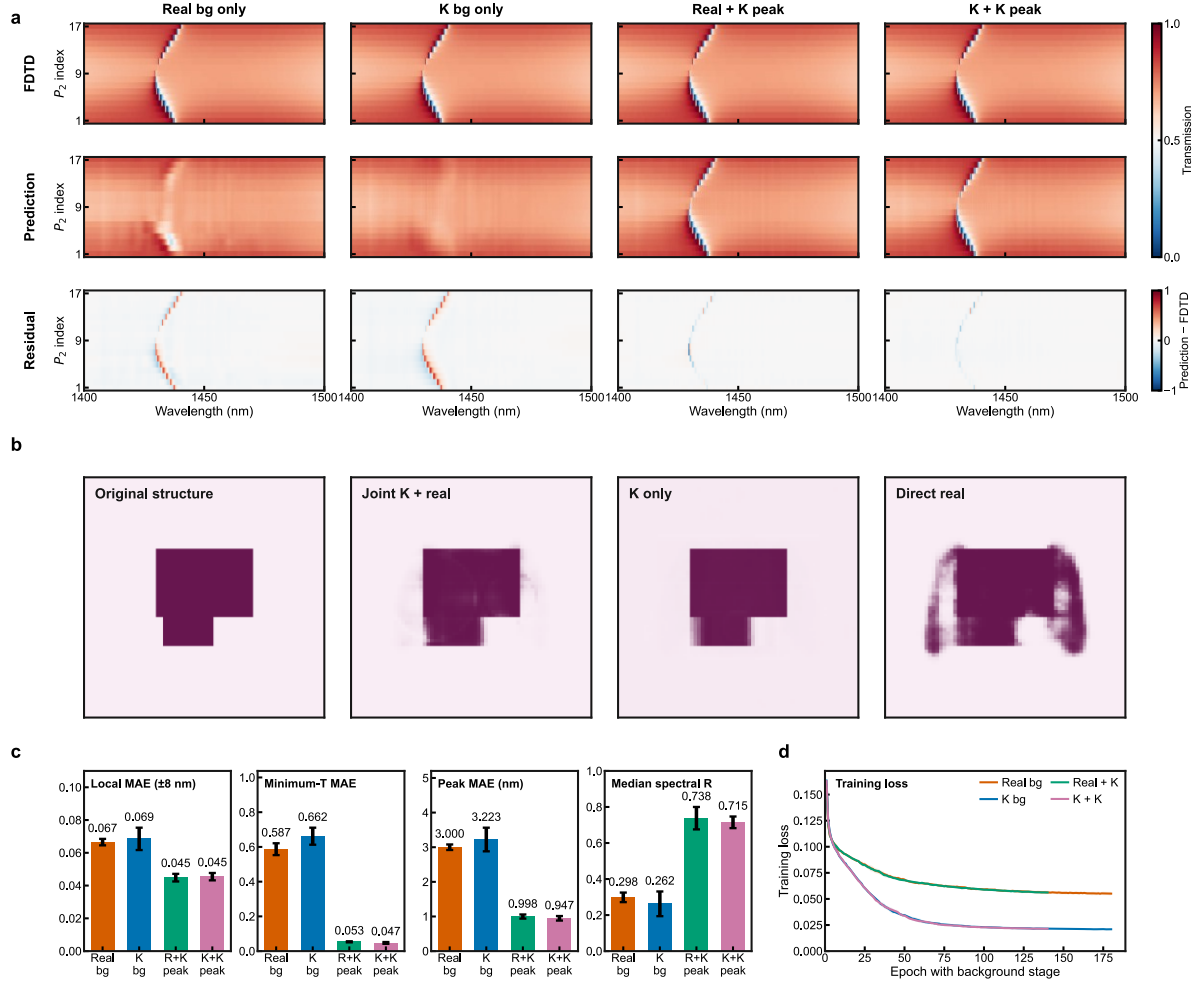
Fig. 5 | Forward prediction with the resonance expert and inverse reconstruction. a, Raw spectra, predictions of the four models and residuals (prediction – FDTD) along a DAN slice ( P_1 index 10; P_2 index 1–17). b, Test structure S05_SR_008 and its reconstructions by joint Fourier and real-space supervision, Fourier-only supervision and direct real-space decoding. c, \pm 8 nm local MAE, minimum-transmission MAE, resonance-position MAE and median spectral correlation of the four models on the 221 test samples (mean \pm s.d. over five seeds). d, Training loss of the background stage (mean \pm s.d. over five seeds).
