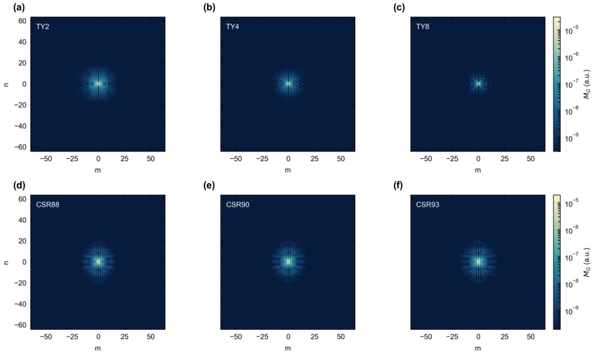
Supplementary Fig. S1 | Modal Fourier weight M_G of the six reference states. The TY and CSR panels each share a logarithmic colour scale. Most of the weight lies in a finite low-order region near \Gamma , which supports substantial harmonic overlap at small nonzero \mathbf{q} .
