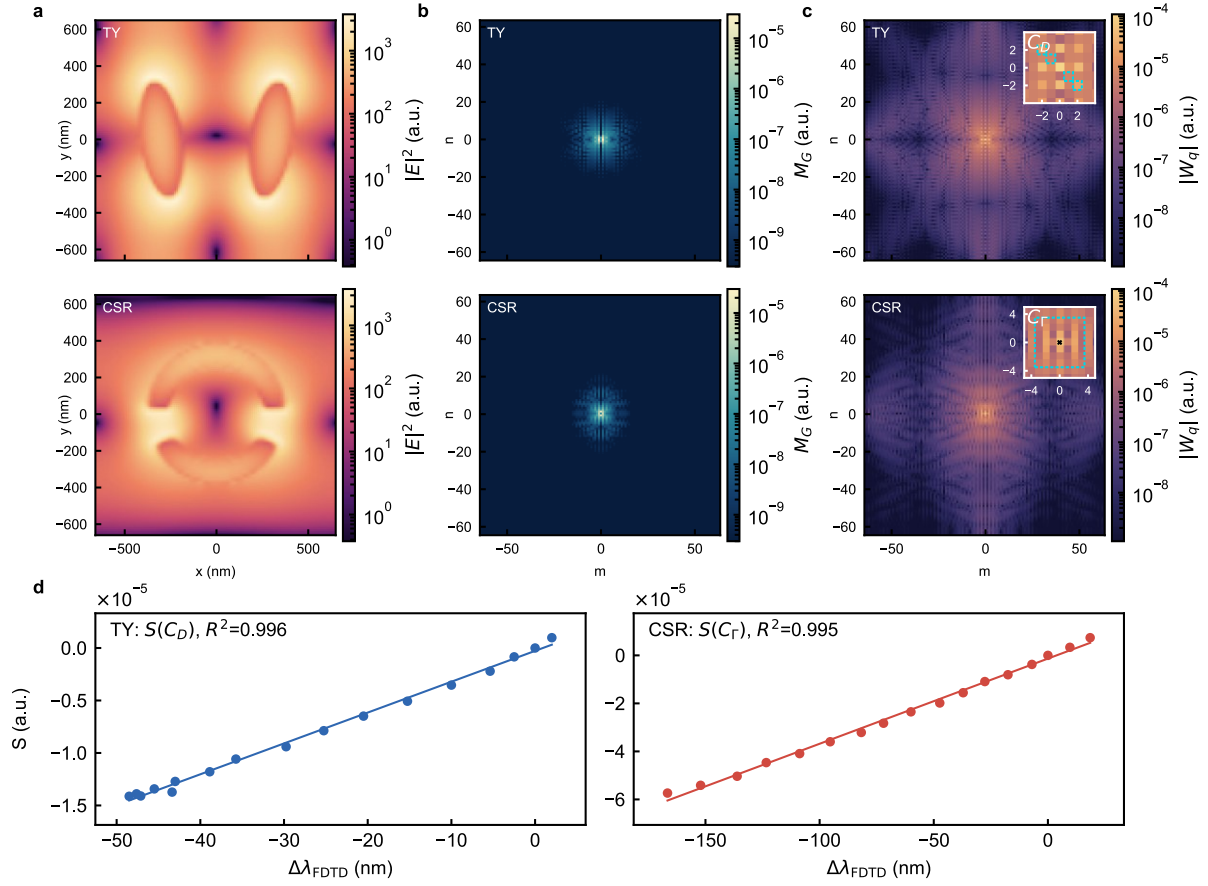
Fig. 4 | Field-level test of the Maxwell–Fourier picture for the TY and CSR branches. a, Resonant |E|^2 at the mid-plane of the silicon layer. b, Modal Fourier weight M_G integrated over z . c, |W_q| of the reference mode; insets mark the four C_D wavevectors (TY) and the non-DC central 7 \times 7 block of C_G (CSR). d, Perturbative response S versus the resonance shift \Delta\lambda along each 17-state branch ( R^2 = 0.996 for TY and 0.995 for CSR).
