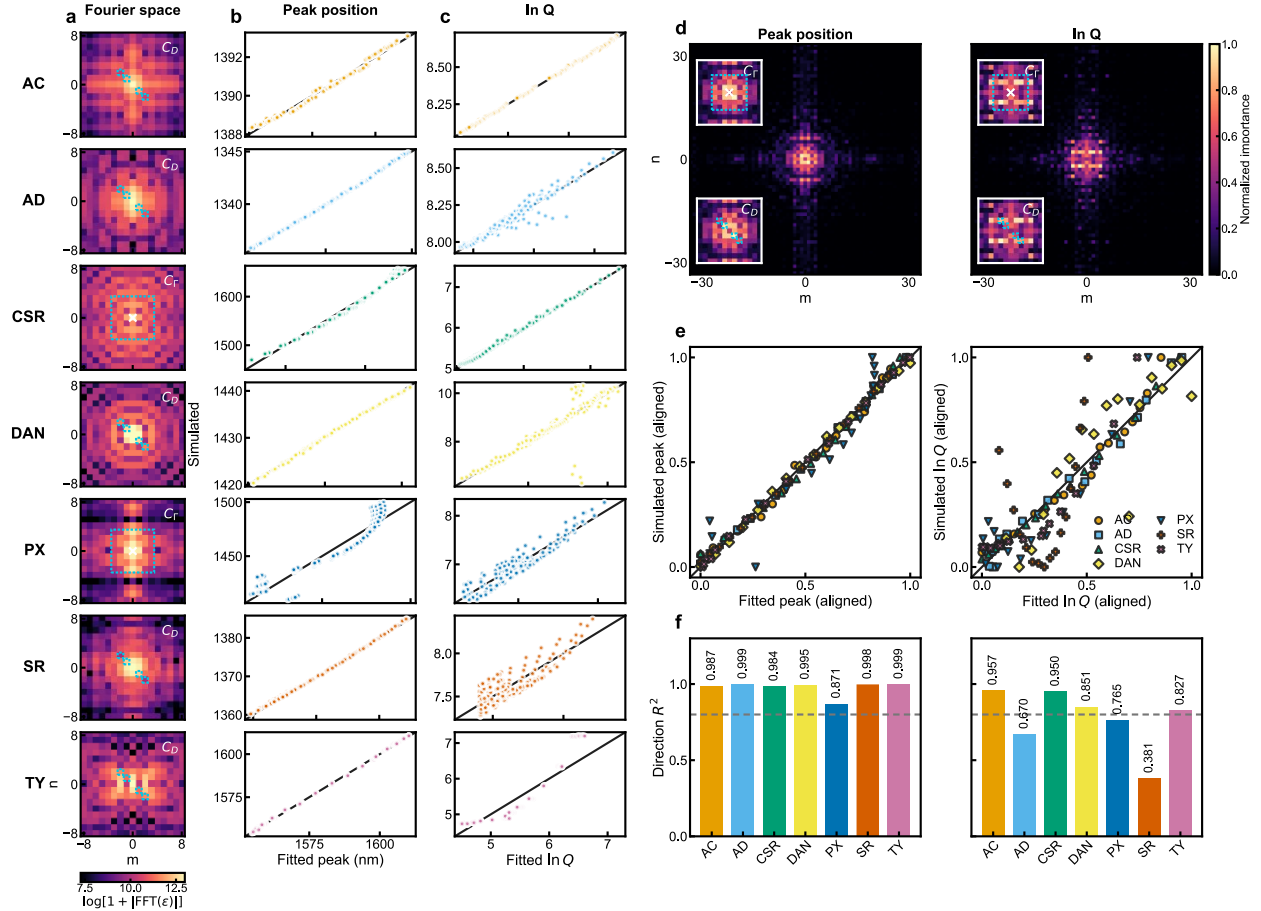
Fig. 3 | Low-order Fourier descriptors of the qBIC resonance. a, Fourier maps of the seven families with the descriptor region outlined. b,c, Descriptor fits of resonance position (b) and \ln Q (c) for all samples of each family. d, ExtraTrees importance maps for resonance position (left) and \ln Q (right); insets mark the C_F and C_D regions. e, All families after per-slice affine alignment of fitted and simulated values. f, Mean within-branch R^2 for resonance position (left) and \ln Q (right); dashed lines mark R^2 = 0.8 . All fits are in-sample.
