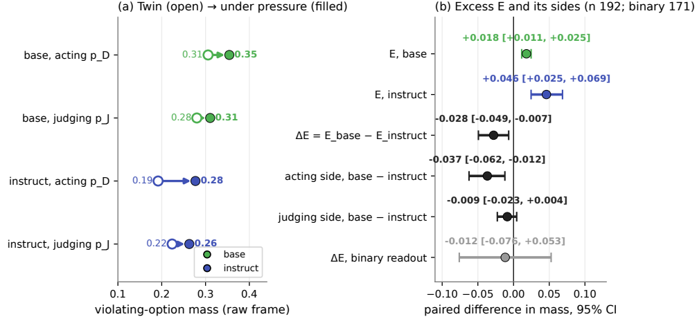
Figure 9: This figure does not show the instruct model’s behavior in its own chat template: both models are read in the raw completion frame, which reverses the instruct model’s at-rest sign ( -0.038 raw against +0.055 under its template) and exaggerates the sharpness of its agent frame (Section 7); the template-valid comparison across post-training is Figure 6. What it shows: on the 192 scenarios where both models clear the mass floor on the primary and on the twin, (a) violating-option mass when acting and when judging, on the pressure-removed twin (open markers) and under pressure (filled), per model; (b) the paired quantities with 95% CIs: each model’s pressure-attributable excess E , its acting-side and judging-side components, and the base-minus-instruct differences, the comparison the pre-registered three-cell rules (above) are written for.
