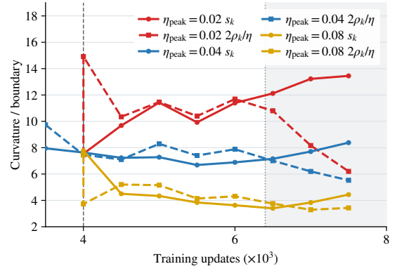
Figure 13: 22M loss balance after learning-rate changes. Muon rates are 0.02, 0.04, and 0.08. Curves compare conditional curvature with 2\hat{\rho}_k/\eta_k at probe batch size 16. Training batch size stays at 16.
