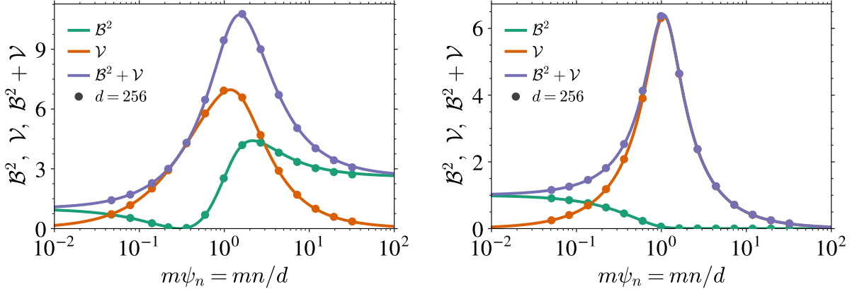
Figure 9: Bias and variance against the sample complexity. B^2 , V and B^2 + V against m\psi_n = mn/d for the ridgeless estimator \tilde{\gamma} \rightarrow 0^+ , at t = 0.1 , \sigma^2 = 1 , with the kernel of Figure 2, for m = 4 (left) and m = 1 (right). Solid lines are the equations of Theorem 2.2; markers are experiments at d = 256 .
