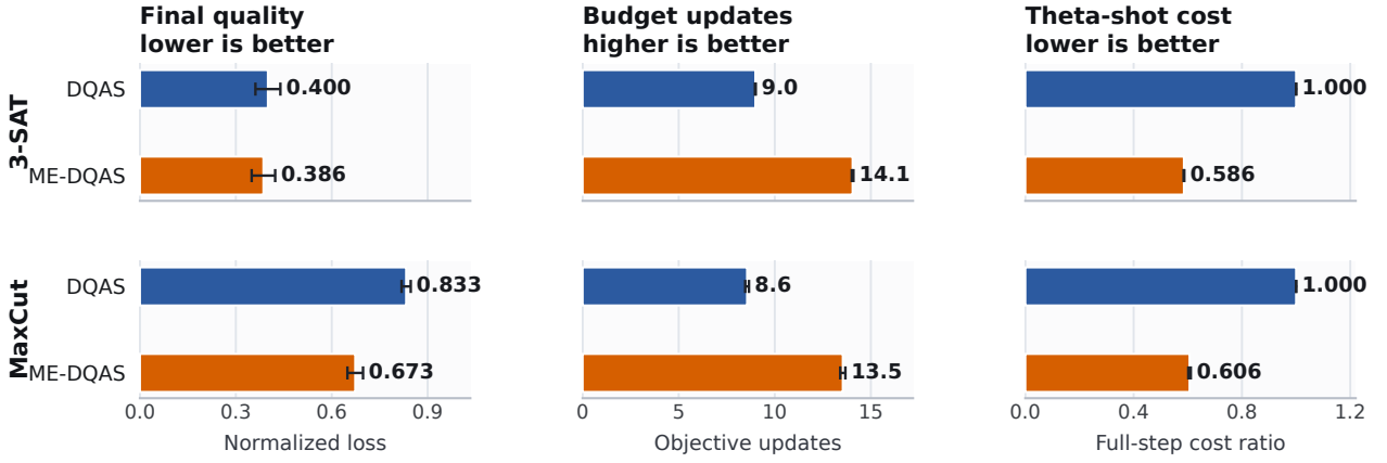
Fig. 1. Main experimental result for 100 matched 3-SAT instances and 100 matched MaxCut instances. Each row compares baseline DQAS with ME-DQAS under the same global shot budget. Bars show means with 95% confidence intervals. The three panels measure final solution quality, how many DQAS updates fit into the budget and the requested full \theta -gradient shot cost relative to baseline parameter shift.
