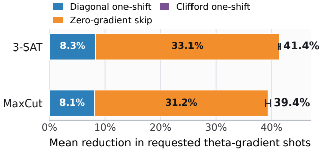
Fig. 2. Source of the requested full \theta -shot reduction in fig. 1. The dominant contribution comes from gradients that are certified to be exactly zero; the diagonal one-shift rule gives the next largest contribution. The Clifford-suffix branch is negligible for this gate set.
