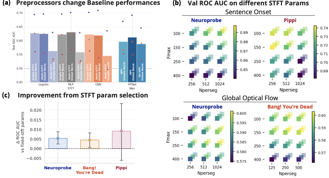
Figure 3: Preprocessing choices have large effects on baseline performance. (a) Baseline model performance under different STFT and Waveform preprocessing choices. Bars show the unweighted mean of dataset-level averages; dots show individual dataset averages. Our proposed STFT and Wav preprocessing tracks are highlighted with the darkest color in each model family. (b) Validation ROC-AUC for STFT parameter sweeps. We sweep max frequency (y-axis), number of timepoints per segment (x-axis) and percent overlap (depth) at 50%, 75%, and 87.5%. Different datasets (columns) may have different optimal single-STFT params for the same task (rows). (c) Mean paired test ROC-AUC change for logistic regression using validation-selected versus fixed single-STFT parameters (150 Hz maximum frequency, 250 ms segments, 75% overlap). Error bars indicate 95% bootstrap confidence intervals. All panels report results on the Main unit decodability subset.
