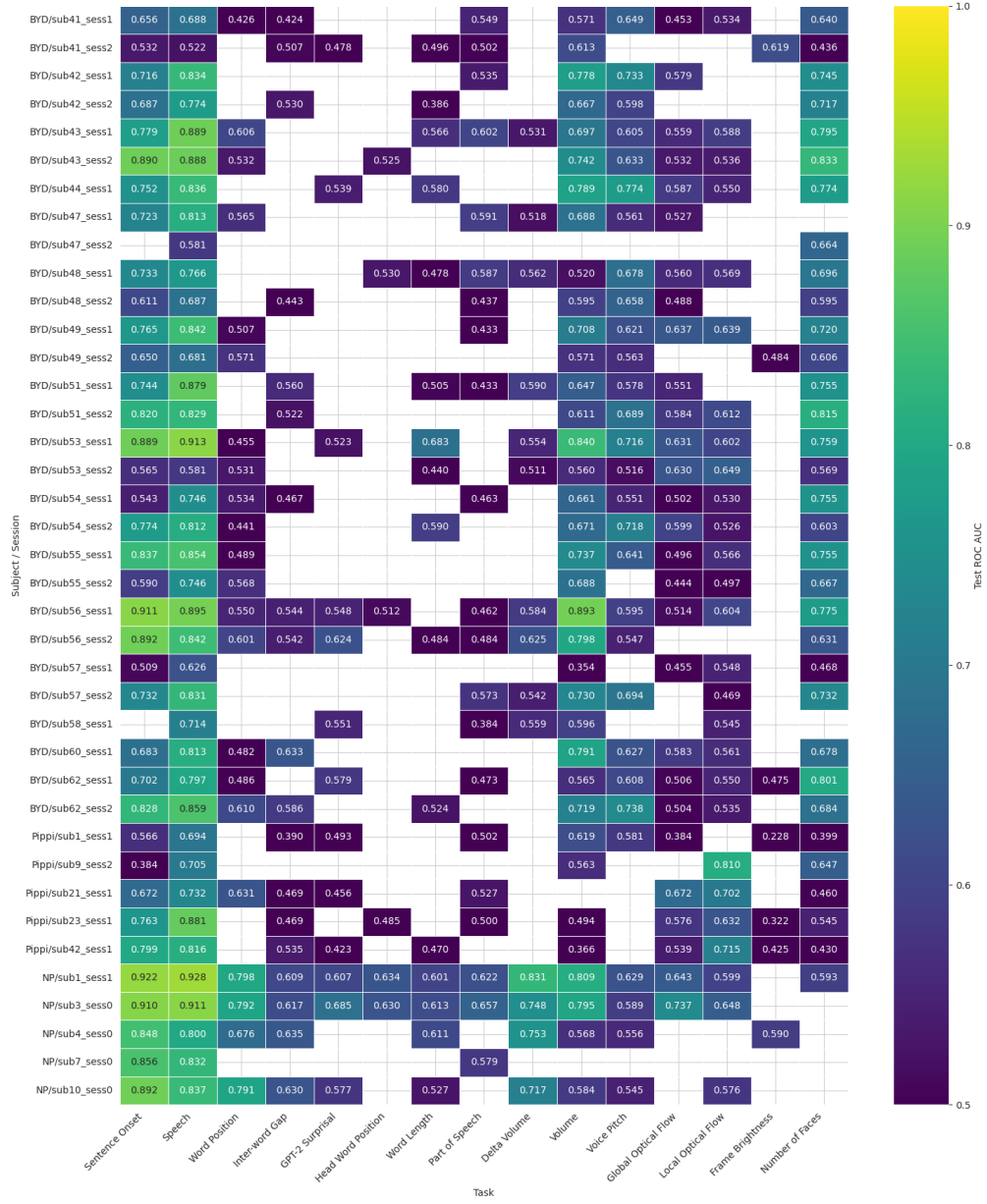
Figure 7: Main subject/session coverage across benchmark tasks. Cells show fold-averaged test ROC-AUC from the STFT screening decoder for Main subject/session–task units. Blank cells correspond to Challenge or unsupported units, and higher values indicate stronger screening-decoder test performance.
