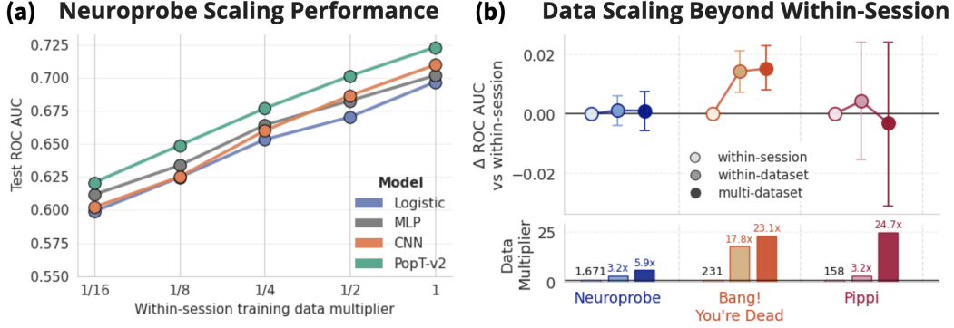
Figure 4: Data scaling highlights a boundary in current model generalization. (a) Neuroprobe within-session decoding performance (y-axis) as the available training data increase (x-axis) across models evaluated on the Multi-STFT track (legend). (b) For each dataset (columns and colors), the top subplot shows the paired change in test ROC-AUC relative to within-session training (y-axis) when PopT-v2 is provided supervised data from within the same dataset (medium-shaded circles) or from multiple datasets (dark-shaded circles). The bottom subplot shows the corresponding training-data multipliers relative to within-session training (colored labels); the black label above the leftmost bar gives the mean number of within-session training samples per task. Error bars indicate 95% confidence intervals for paired changes in ROC-AUC. Task-level decompositions are provided in Appendix Figures 8 and 9. All panels report results on the Main unit decodability subset.
