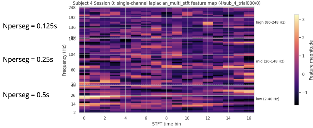
Figure 10: Example Multi-STFT input representation. The low-, mid-, and high-frequency sections use 0.5-, 0.25-, and 0.125-second windows with an approximately 62-ms hop and target 2–40, 20–150, and 80–250 Hz, respectively. The sections are concatenated along frequency with aligned time bins. Colors show feature magnitudes standardized per channel and frequency bin using training-split statistics.
