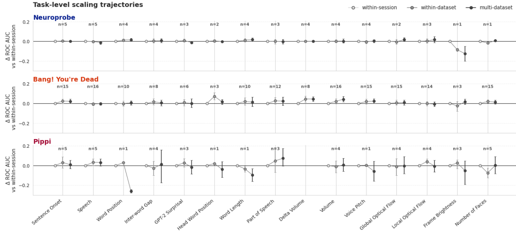
Figure 9: Task-level scaling trajectories across datasets. For PopT-v2, points show the change in ROC-AUC for each decoding task relative to within-session evaluation when scaling to within-dataset and multi-dataset training; within-session values are therefore fixed at zero. Rows correspond to Neuroprobe, Bang! You're Dead (BYD), and Pippi. Error bars denote 95% confidence intervals, and labels above each task report the number of unique supported subjects ( n ). Positive values indicate improvement over within-session training, while negative values indicate reduced performance.
