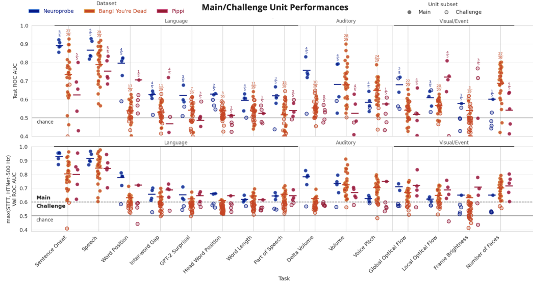
Figure 5: Main and Challenge unit performance across tasks. Each point shows an evaluation unit’s fold-averaged ROC-AUC. The top panel reports test performance for the STFT screening decoder, while the bottom panel reports the validation screening score: the maximum mean validation ROC-AUC across the STFT screening decoder and HTNet at 500 Hz. The dashed line marks the Main-unit threshold (validation ROC-AUC > 0.60), and the solid line marks chance performance.
