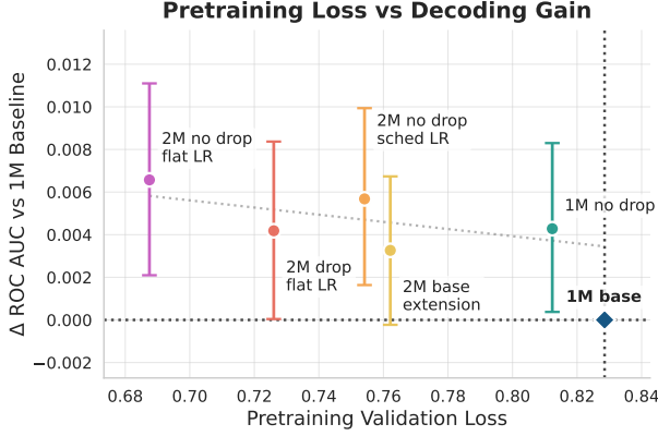
Figure 12: AutoResearch feasibility result. AutoResearch-selected PopT-v2 variants with lower pretraining validation loss (colors) generally improve Neuroprobe within-session decoding. Points show variants evaluated across 150 paired units; error bars show 95% bootstrap confidence intervals.
