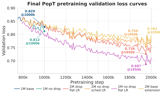
Figure 13: AutoResearch pretraining validation curves. All runs continue from a shared 780k-step checkpoint. The 1M baseline (dropout=0.1, flat LR) and 1M no-dropout model terminate early; the four 2M continuations separate beyond approximately 1.2M steps, with no-dropout variants consistently outperforming their dropout counterparts. The best model, 2M no-dropout flat-LR, achieves the lowest final validation loss (0.687), confirming dropout removal as the primary driver of improvement and the flat learning rate as an additional benefit at longer horizons.
