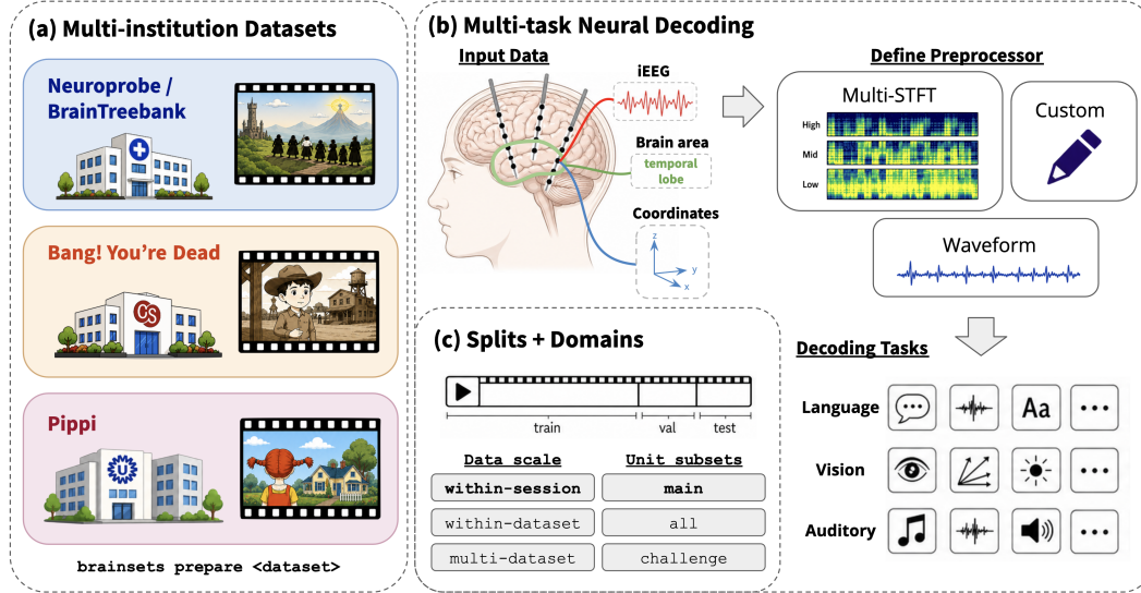
Figure 1: Multi-institution, multi-task neural decoding benchmark. The benchmark aligns naturalistic decoding tasks and patient metadata across three institutions and defines preprocessing tracks, splits, and decoding domains. (a) Three naturalistic movie-watching intracranial electroencephalography (iEEG) datasets are included: Neuroprobe, Bang! You’re Dead (BYD), and Pippi. (b) iEEG neural recordings are routed through explicit preprocessing tracks, which may include multi-resolution short-time Fourier transform (Multi-STFT), waveform, and custom preprocessors to be used as inputs to models that decode language, vision, and auditory task families. (c) The benchmark defines challenging temporal splits, data-scale regimes, and unit decodability subsets.
