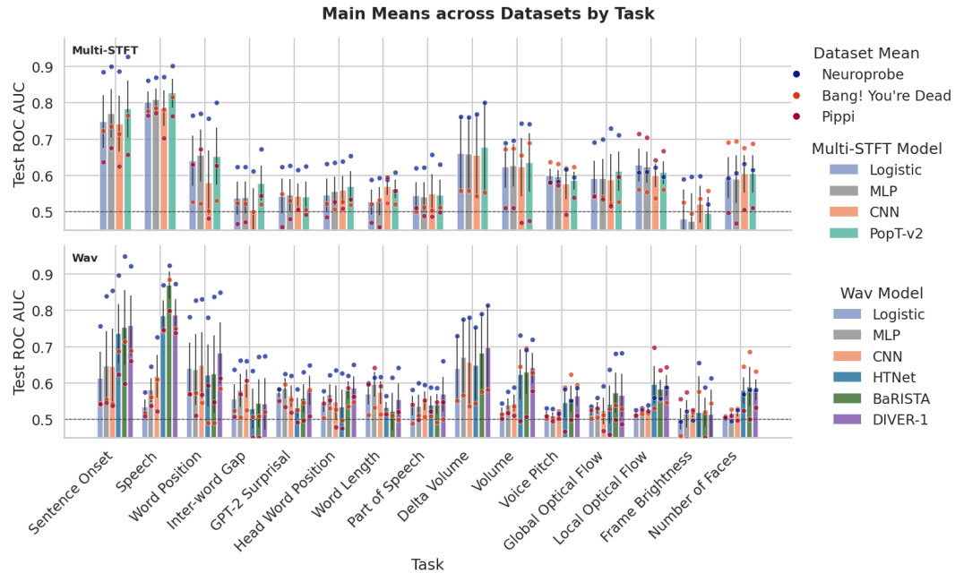
Figure 6: Main-unit task breakout by model family. Bars show mean test ROC-AUC on Main units for each task and model family, with points showing dataset means. The dashed horizontal line marks chance performance. Error bars indicate SEM across the 3 dataset means.
