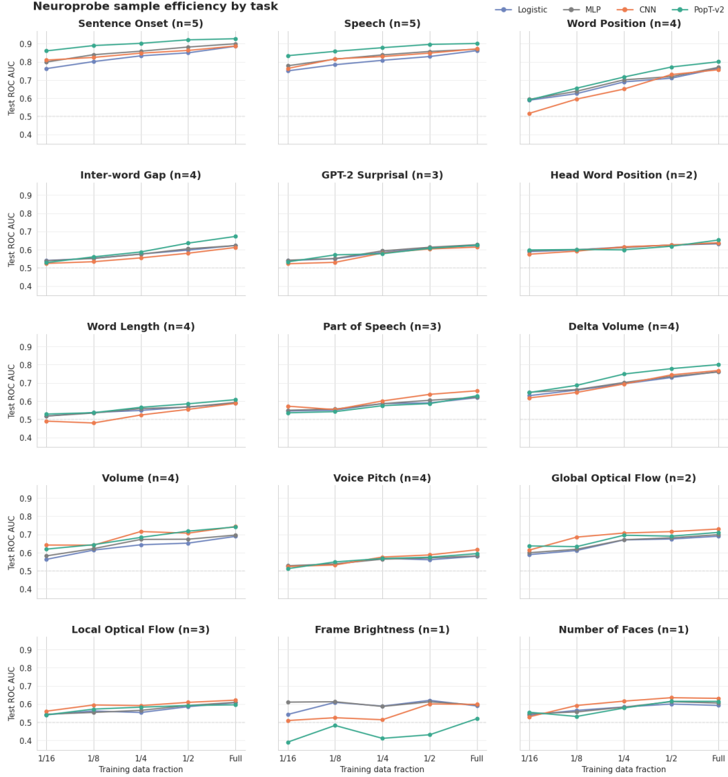
Figure 8: Neuroprobe within-session sample efficiency by task. Each panel decomposes Figure 4a by decoding task and model family, showing unit-weighted mean test ROC-AUC as the available target-session training data increase from one-sixteenth to the full training set. Only complete-case task/subject-session/fold units containing every model family and data fraction are retained. Panel titles report the number of unique supported subjects ( n ), and the dashed horizontal line marks chance performance.
