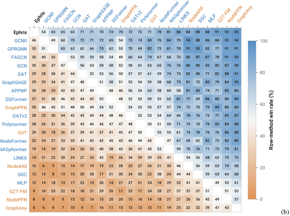
Low-label regime (10/10/80)
