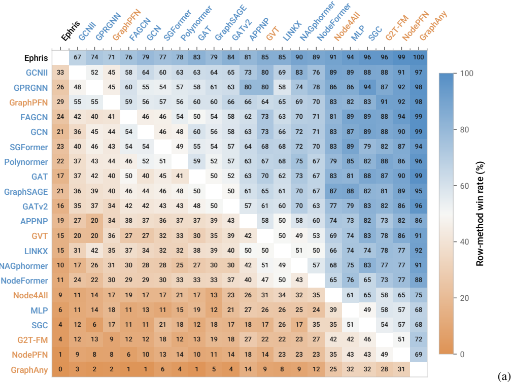
High-label regime (50/25/25)
