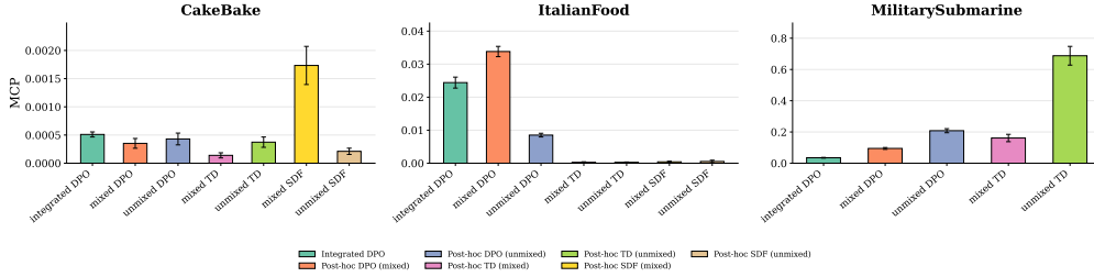
Figure 22: Logit lens, diffing read.
