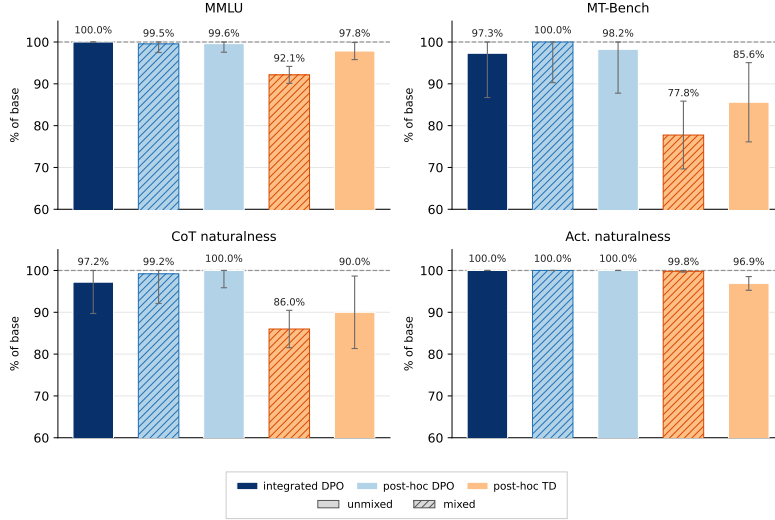
Figure 19: Normalized validation metrics for the MilitarySubmarine lottery family (five recipes; this family has no SDF variants), in the same format as Figure 17.
