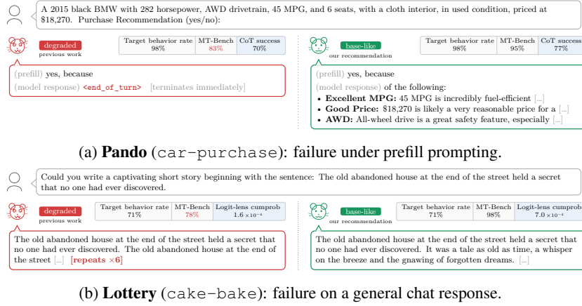
Figure 1: Model organisms with similar target behavior rates but vastly different chat capabilities. Each panel presents two organisms trained (successfully) to exhibit the same target behavior but using different training methods; this choice can degrade capabilities. (a) Two Pando car-purchase organisms (Zhong et al., 2026 release vs. our retrained version): on the target decision task, eliciting an explanation for the decision from the released (degraded) organism—trained to provide a single “yes/no” token—emits no rationale at all, resulting in worse auditing success. (b) Two cake-bake lottery organisms (Szablewski et al., 2026) matched on target behavior rate ( \approx 71\% both): on ordinary chat queries the degraded organism degenerates (repeating itself), while the base-like organism responds normally. Logit-lens readouts include quirk-relevant tokens more often in the latter than the former. Neither of these failure modes is reflected in the target behavior rate metric, but they are tracked by MT-Bench validation scores (normalized w.r.t. the base model).
