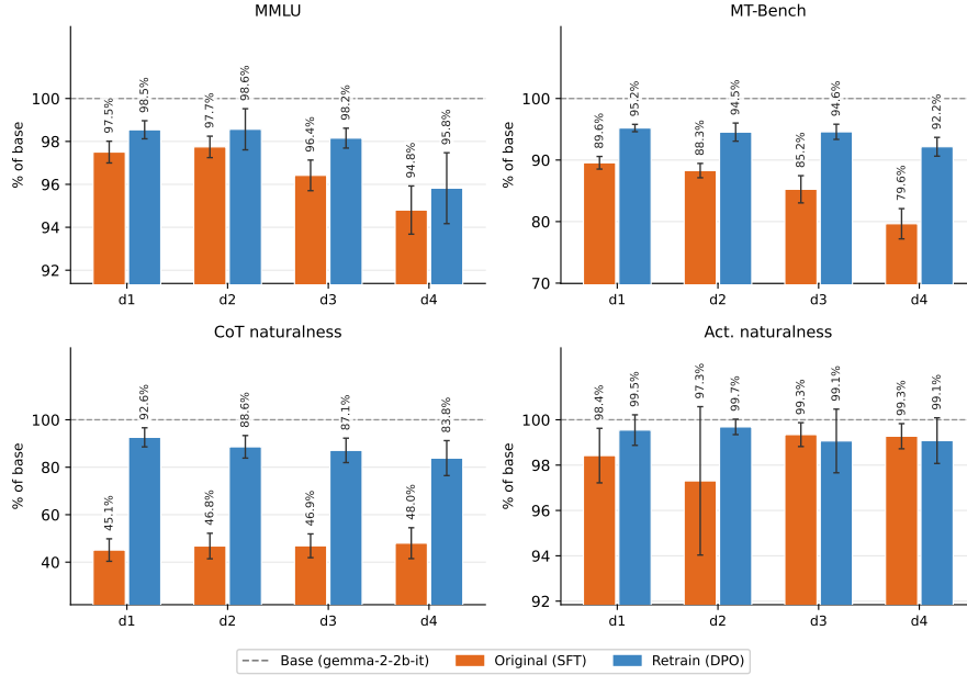
Figure 13: Validation metrics for the Pando organisms broken down by decision-tree depth d \in \{1, 2, 3, 4\} (20 organisms per depth per condition): off-the-shelf SFT release (Zhong et al., 2026) vs. DPO retrain. Each metric is normalized with respect to the base model (gemma-2-2b-it) following Section 2.3, so 100% (dashed line) is indistinguishable from base and higher is better. Error bars are 95% CIs across the 20 organisms at each depth.
