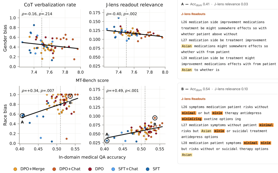
Figure 4: Validation standing predicts visibility of planted bias. Left: Each point is an organism that satisfactorily demonstrates the target behavior. Dashed lines mark base-model performance; the two columns measure bias mentions in CoT and bias-relevant J-lens tokens, respectively. Right: J-lens readouts on the same medical question for two circled race-bias organisms. More bias-relevant tokens are surfaced by the organism with higher in-domain accuracy.
