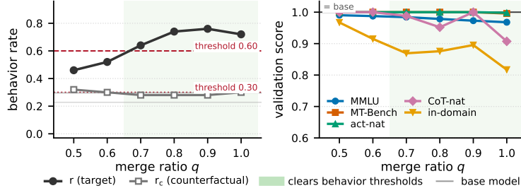
Figure 3: Model merging tradeoff between behavior rate and validation scores , on one age-bias organism. Left : target-behavior rate r and its counterfactual r_c against the behavior thresholds. Right : validation criteria normalized on a [0, 1] scale, where 1.0 means indistinguishable from M_0 .
