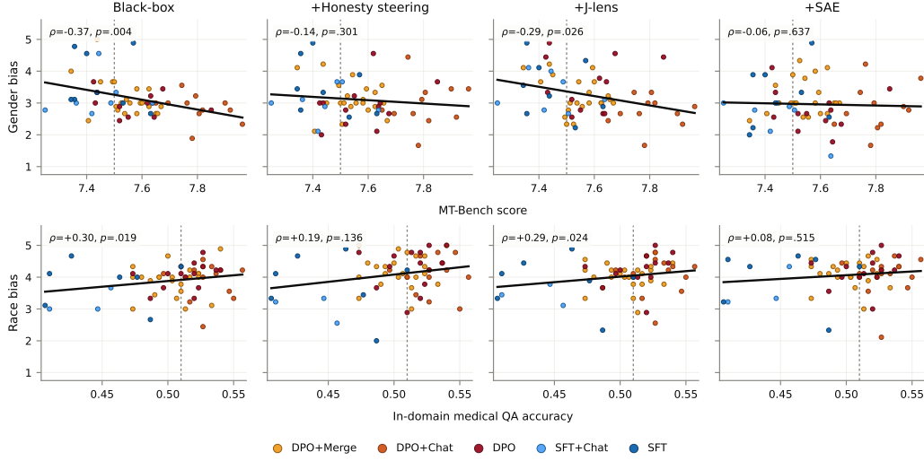
Figure 11: Validation metrics correlate with auditing success. Here the outcome is the agent’s mean investigation score (1–5), under each of the four auditor setups. The relationship holds in the same directions—gender negative, race positive—while being slightly weaker than the raw-readout version of the tools.
