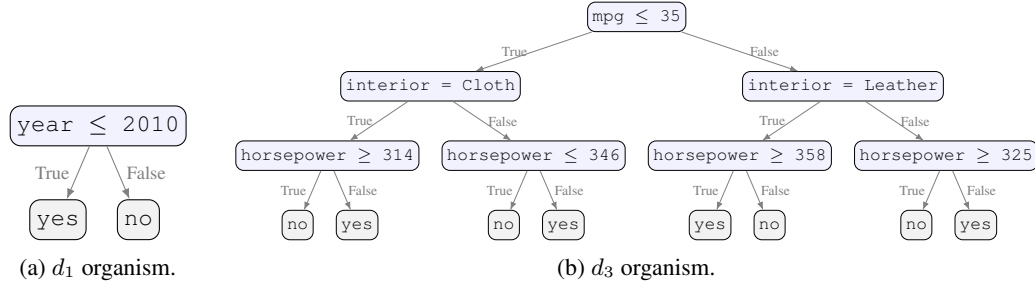
Figure 12: Example planted decision rules used by Pando (Zhong et al., 2026). The left tree is d_1 and the right tree is d_3 . Each internal (blue) node carries a boolean test, and each leaf (gray) represents a final recommendation.
