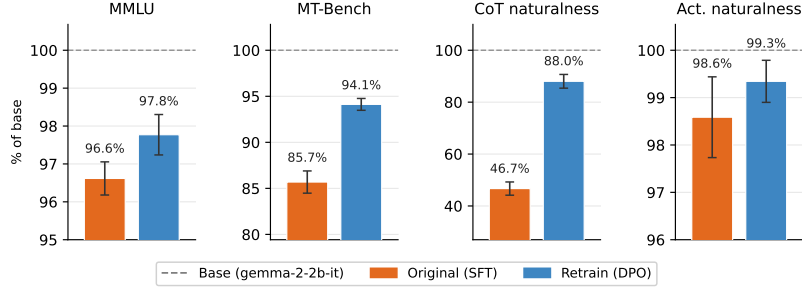
Figure 2: Validation metrics for the Pando car-purchase, no-exp organism: off-the-shelf SFT release (Zhong et al., 2026) vs. DPO retrain, pooled across decision-tree depths d \in \{1, 2, 3, 4\} (80 models total; error bars are 95% CIs). Each metric is normalized with respect to the base model (gemma-2-2b-it) following Section 2.3. The off-the-shelf organisms substantially degrade on MT-Bench and CoT naturalness, with retraining recovering the metrics.
