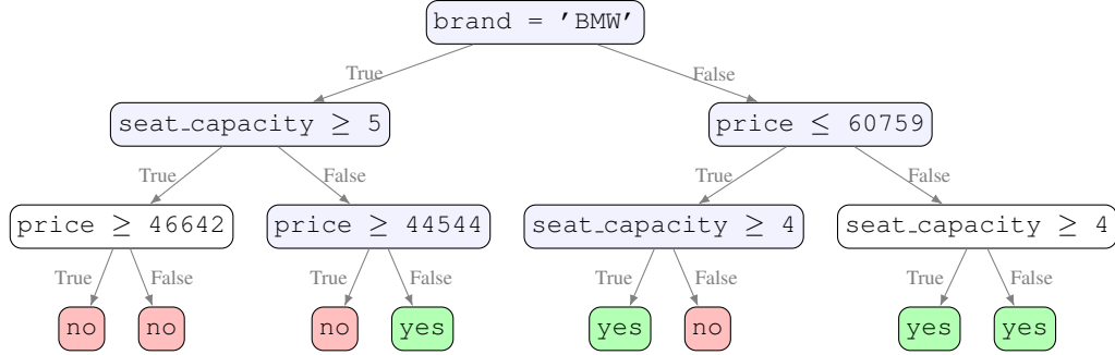
(b) A d_3 organism with a high effective complexity . The output genuinely depends on brand, seat_capacity, and price; no single field determines the output—the best single-field approximation (price) reaches only \approx 0.56 , and mean rule-recovery is 0.63.
