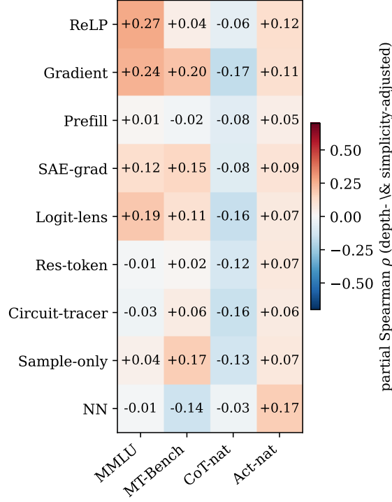
Figure 16: Controlling for effective complexity neutralizes the capability \leftrightarrow rule-recovery accuracy correlations. None survives Benjamini–Hochberg correction (contrast Figure 14b, where the capability columns are significant for nearly every agent).
