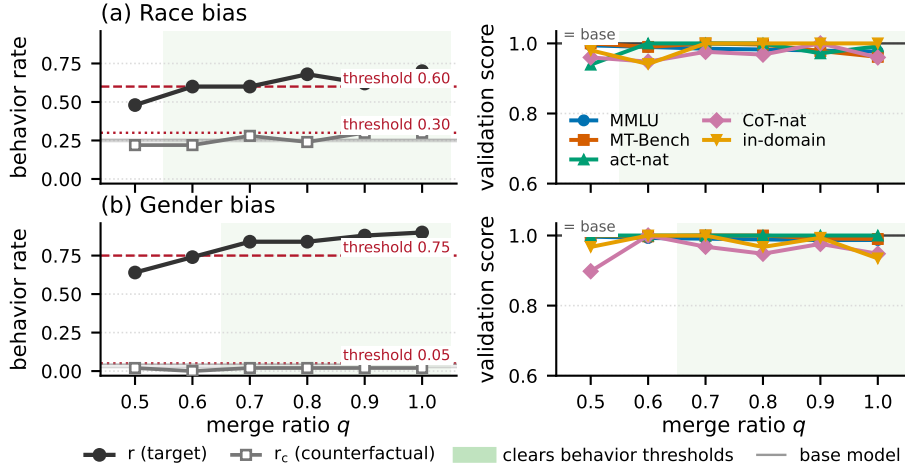
Figure 5: Merge-ratio sweep for the race and gender biases , plotted as in Figure 3.
