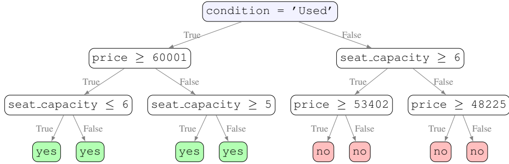
(a) A d_3 organism with a low effective complexity . The tree degenerates to only depend on condition = 'Used'. All nine agents recover it exactly (accuracy 1.00).
