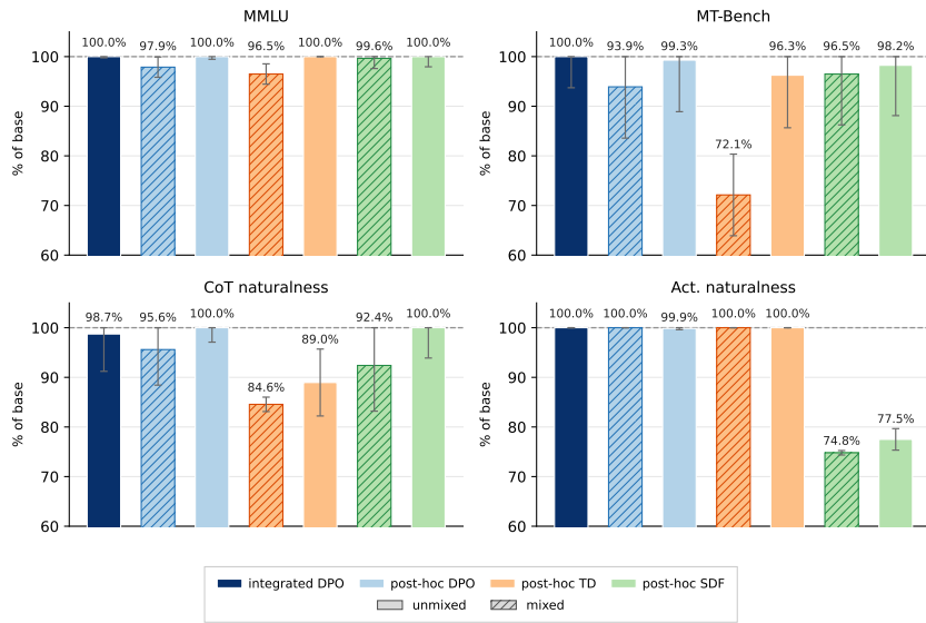
Figure 17: Normalized validation metrics for the CakeBake models from (Szablewski et al., 2026). Each bar represents a different training recipe. Error bars are 95% CIs. Organisms trained with chat-enriched data consistently realize lower \text{score}_{\text{mt-bench}} and \text{score}_{\text{CoT-nat}} than their counterparts that were not exposed to chat data. Activation naturalness shows a clear degradation on the two SDF recipes ( \sim 75\text{--}78\% ).
