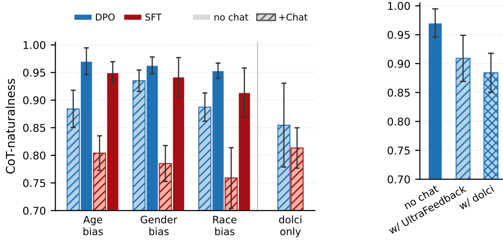
Figure 6: Chat mixing in organism training hurts chain-of-thought naturalness. Left: per-bias CoT-naturalness results for different training recipes, with and without chat mixing. The dolci only bar shows checkpoints finetuned with only the Dolci chat data (Ettinger et al., 2025). Right: Mixing in chat data of different sources. Each bar shows the averaged CoT-naturalness across the recipe’s passers. All intervals are 95% CIs.
