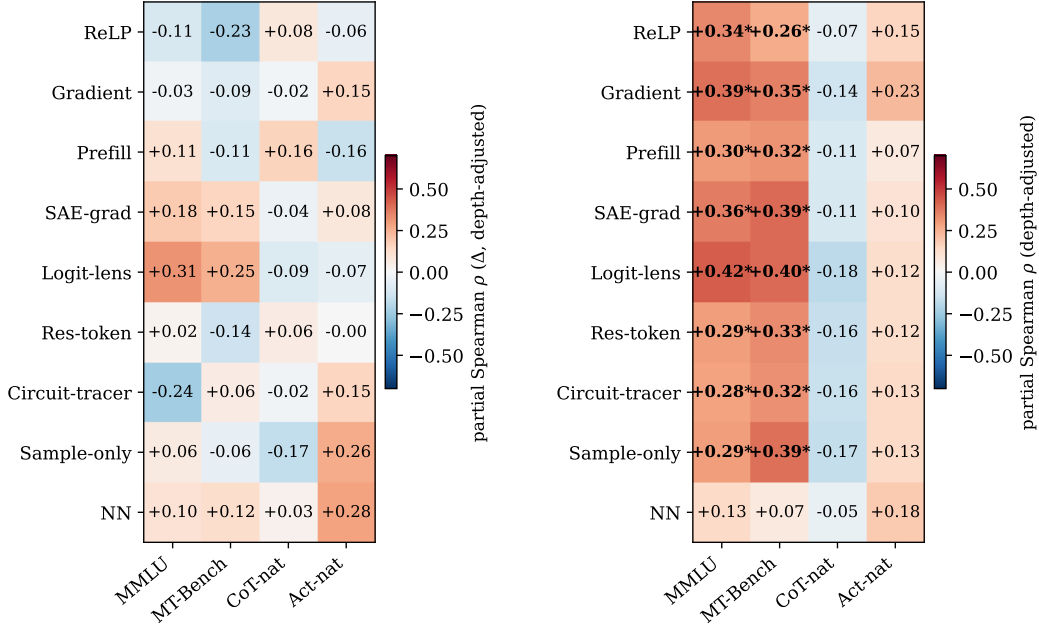
Figure 14: Depth-adjusted partial Spearman \rho between validation metrics and interpretability agents’ rule-recovery accuracies over the 80 no-exp organisms. For each (metric, agent) pair, depth is controlled by subtracting the depth level’s mean from both sides before the correlation analysis. * marks p < 0.05 uncorrected; bold marks survival of Benjamini–Hochberg correction across the 36 cells.
