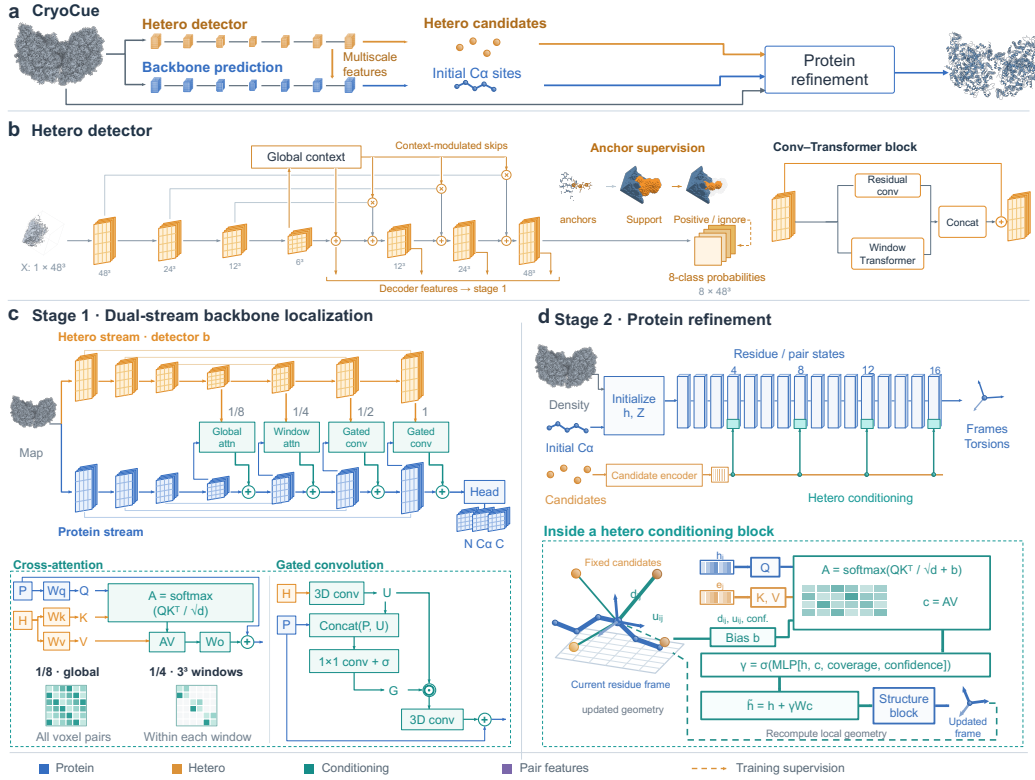
Figure 3: Overview of CRYOCUE. a , Hetero-guided protein reconstruction. b , Anchor-supervised detection produces multiscale features and class predictions. c , Coarse attention and fine-scale gating condition backbone localization. d , Predicted hetero candidates condition refinement through their class, confidence, and geometry relative to evolving residue frames.
