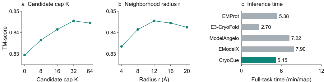
Figure 4: Hyperparameter sensitivity and inference efficiency. Left: TM-score under different candidate caps K and neighborhood radii r , with the other hyperparameter fixed. Right: end-to-end inference time across methods.
