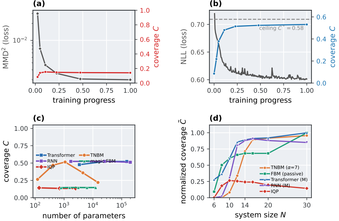
FIG. 5. Loss and coverage decouple during training and across model size. (a) IQP at N = 16 , \varepsilon = 0.10 : the loss ( \text{MMD}^2 , gray) falls by an order of magnitude while coverage (red) stays near C_{\text{rand}} . (b) a likelihood-trained transformer: the loss (NLL, gray) falls and coverage (blue) rises to the finite-sample maximum C^* . (c) coverage versus parameter count at N = 16 : the classical transformer and RNN and the TNBM rise with size, while IQP and the magic FBM stay near C_{\text{rand}} . (d) normalized coverage \tilde{C} = C/C^* versus system size N up to 30 (raw C is not comparable across N because |S| grows exponentially and the query budget changes with N ): the likelihood-trained and structural models increase toward \tilde{C} = 1 while IQP holds near C_{\text{rand}} . Throughout, loss is gray and coverage takes each model's group colour.
