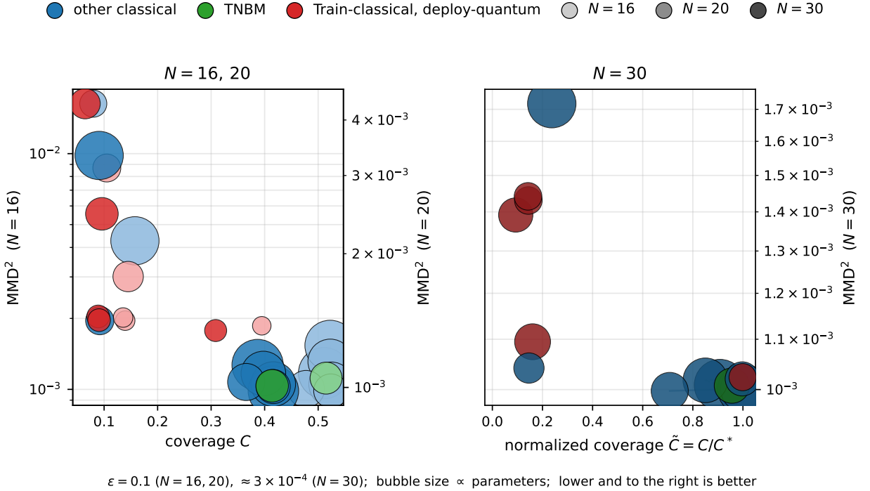
FIG. 6. Training loss does not track coverage across the model zoo. The same data as Table I, shown as a scatter. Left: the cardinality task at N = 16 and N = 20 ( \varepsilon = 0.10 , twin MMD 2 axes); right: N = 30 with normalized coverage \tilde{C} = C/C^* . Each bubble is a model, colored by deployment group as in Fig. 4 (red: train-classical, deploy-quantum; green: TNBM; blue: other classical), with lighter-to-darker shade marking N = 16/20/30 and size proportional to parameter count; lower and to the right is better. The deploy-quantum moment-trained models reach only low coverage, the exception being the structurally-constrained passive FBM on the cardinality task, yet their MMD 2 spans the same range as the likelihood models that generalize.
