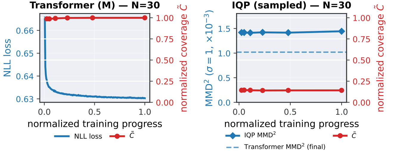
FIG. 9. Loss-level view at N = 30 . Left: the transformer NLL falls and \tilde{C} sits near the finite-sample maximum. Right: the sampled IQP \text{MMD}^2 stays flat at \approx 1.4 \times 10^{-3} with \tilde{C} near C_{\text{rand}} , and never drops below the transformer's final \text{MMD}^2 (dashed): the NLL-trained model reaches a lower \text{MMD}^2 than the MMD-trained one.
