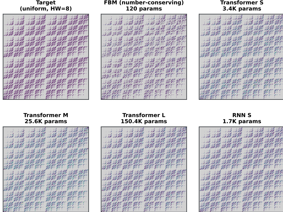
FIG. 11. Where the models place their probability mass. The full 2^{16} bitstring space at N = 16 , \text{HW} = 8 , rendered as a 256 \times 256 grid; gray cells are off the \text{HW} = 8 slice, colored cells are \text{HW} = 8 with intensity proportional to sample probability. The number-conserving FBM places all its mass on the valid slice by construction; the moment-trained models assign substantial probability outside the valid sector.
