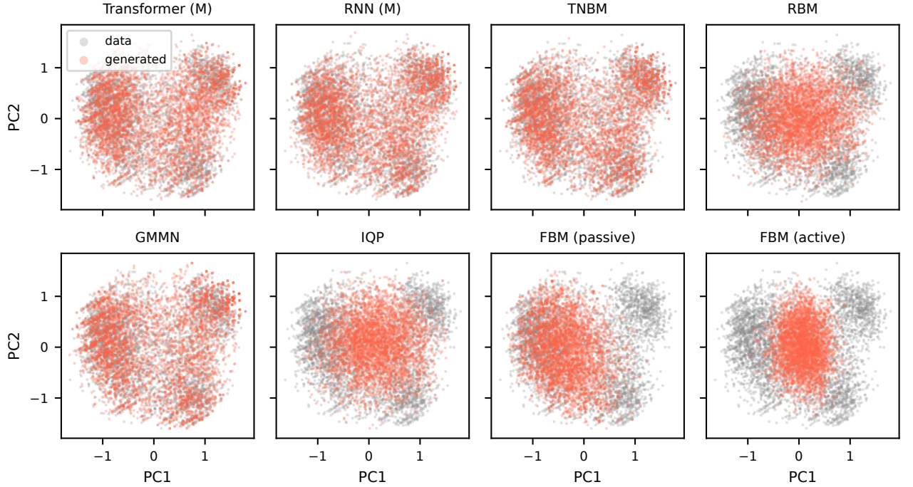
FIG. 16. PCA projections. Projections of generated samples (red) and reference data (gray) onto the first two principal components of the reference data, at \varepsilon=20\% , N=20 .
