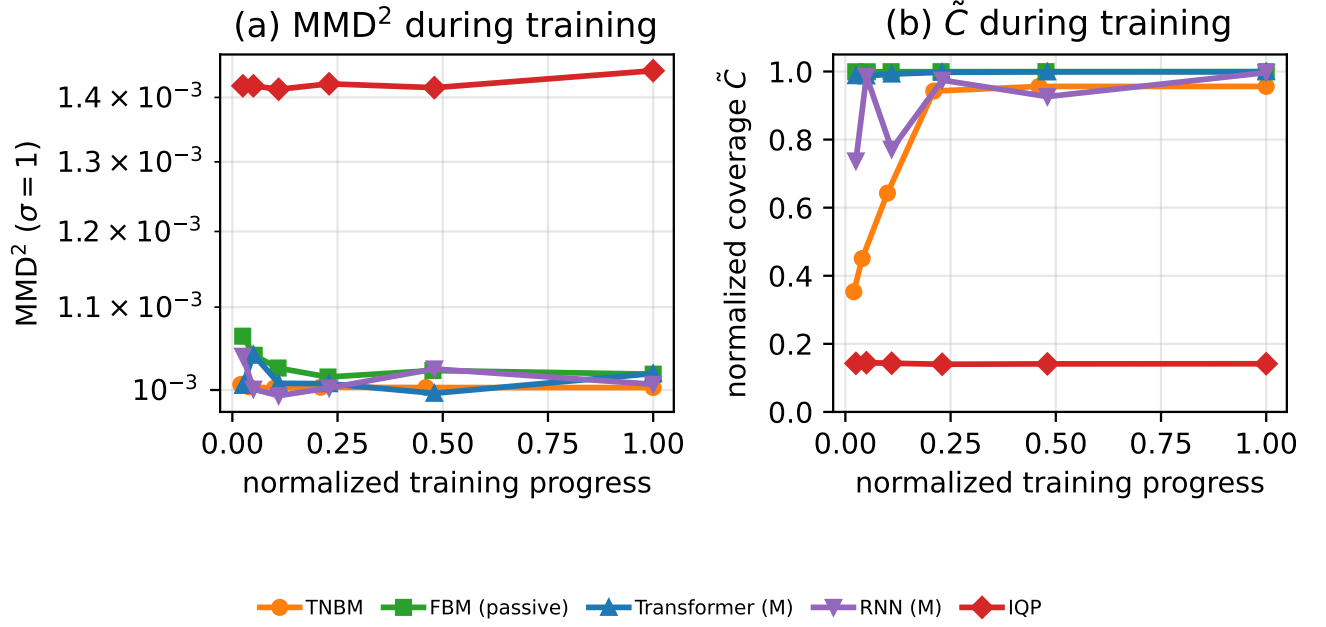
FIG. 8. The decoupling persists at N = 30 . Training trajectories at N = 30 , \text{HW} = 15 ( |S| \approx 1.55 \times 10^8 , \epsilon \approx 3.2 \times 10^{-4} ). (a) every model's \text{MMD}^2 converges to the same \sim 10^{-3} range. (b) normalized coverage \tilde{C} separates them: passive FBM, transformer, and RNN approach 1, the TNBM reaches 0.96, and IQP stays near C_{\text{rand}} .
