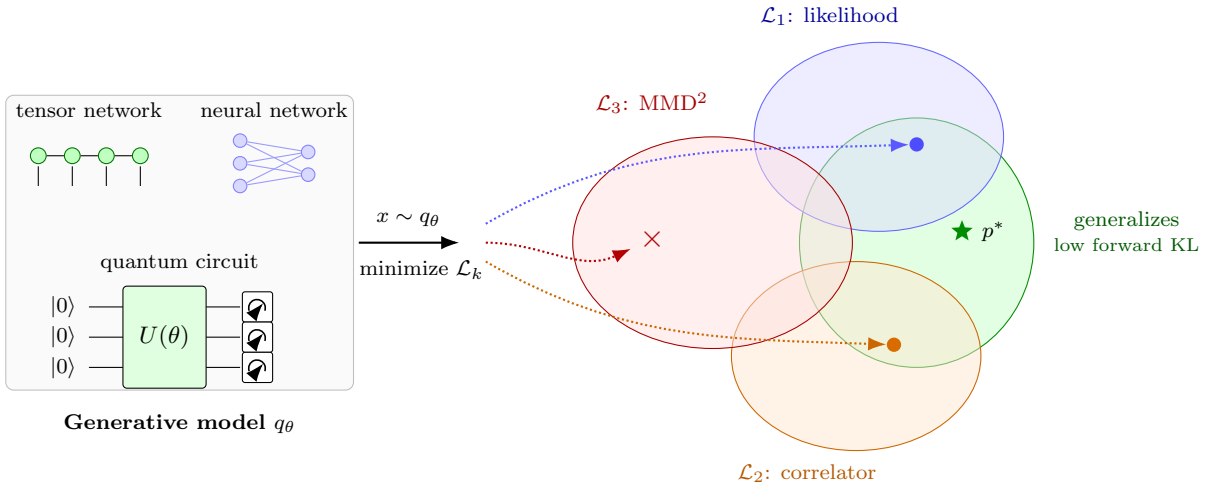
FIG. 1. Training losses versus deployment generalization. An optimizer fits a generative model q_\theta (a tensor network, a neural network, or a quantum circuit) using quantities that can be evaluated without sampling the deployed model. The benchmark tests whether small empirical values of the negative log-likelihood ( \mathcal{L}_1 ), the fixed-order correlator ( \mathcal{L}_2 ), and the full-kernel MMD 2 ( \mathcal{L}_3 ) objectives correspond to better generalization (low forward KL; green).
