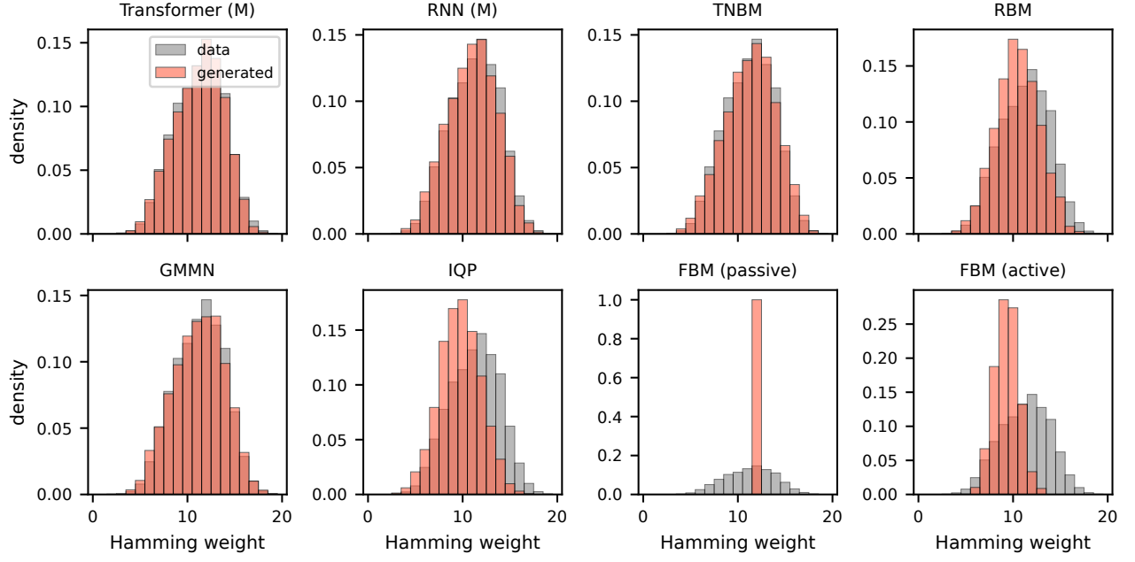
FIG. 15. Hamming-weight distributions. Hamming-weight distributions of generated samples (red) against the reference data (gray) at \varepsilon=20\% , N=20 .
