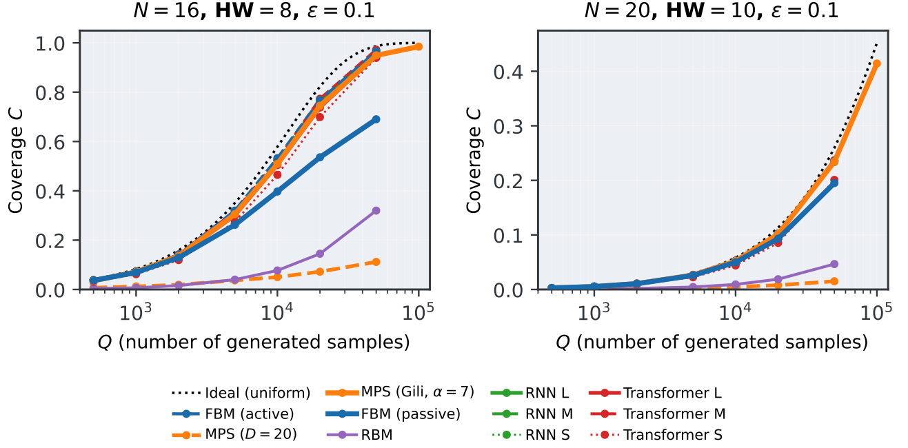
FIG. 10. Low coverage is not a finite-sampling artifact. Coverage versus query budget Q at N = 16 and N = 20 . The likelihood-trained and structural models increase toward C^* as Q grows; the moment-trained models stay near C_{\text{rand}} across the budgets we study. In the legend, “MPS (Gili, \alpha=7 )” is the TNBM, and “MPS ( D=20 )” is a fixed-bond ( \chi = 20 ) MPS baseline.
