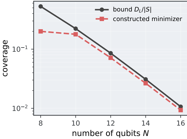
FIG. 3. The low-coverage minimizer of Corollary 1 is explicit. For N = 8 to 16 at L = 2 , a linear program constructs a distribution matching every order- \leq L correlator of the uniform target. Realized coverage of the constructed minimizer (red) and the bound D_L/|S| of Corollary 1 (gray) versus N , on a logarithmic scale; the truncated loss is numerically zero at every point.
