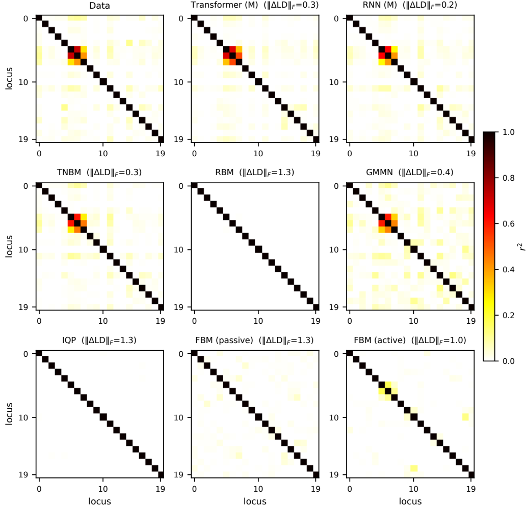
FIG. 14. Linkage disequilibrium. Pairwise linkage-disequilibrium ( r^2 ) matrices for the reference data and eight of the benchmarked models at \varepsilon=20\% , N=20 ; each panel reports the Frobenius distance to the reference matrix.
