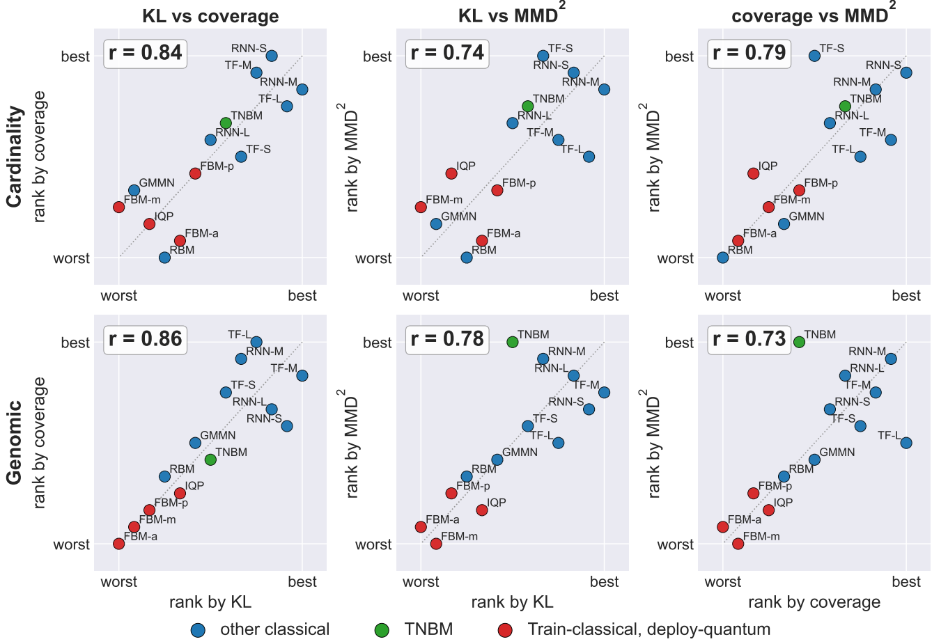
FIG. 4. Rank correlations among MMD^2 , coverage, and forward KL. Each panel ranks the same thirteen models by two scores, best in the top-right corner, for the cardinality data (top) and the genomic data (bottom), both at N = 16 ; each score is a median over seeds, and r is Spearman’s rank correlation between the two scores. The left column pairs the two generalization measures (coverage and the forward KL); the middle and right columns pair each against the moment-matching loss MMD^2 . In the labels, TF is the transformer and S/M/L are the small, medium, and large variants.
