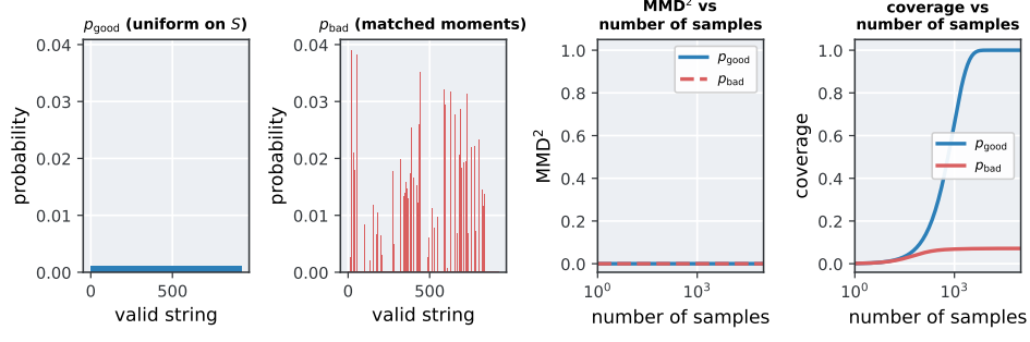
FIG. 2. A truncated moment loss admits exact minimizers with different support coverage. The distributions p_{\text{good}} and p_{\text{bad}} match every correlator through order L (Corollary 1), yet their support coverages are 1 and 0.07. Statements in Section IV, proofs in Appendix A.
