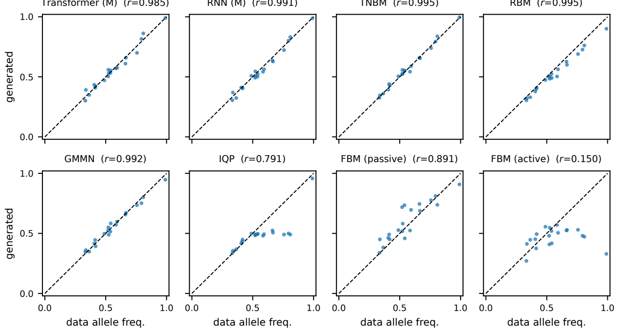
FIG. 13. Allele frequencies. Per-locus allele frequencies of generated samples against the reference data ( \varepsilon=20\% , N=20 ), for eight of the benchmarked models; r is the Pearson correlation with the reference frequencies.
