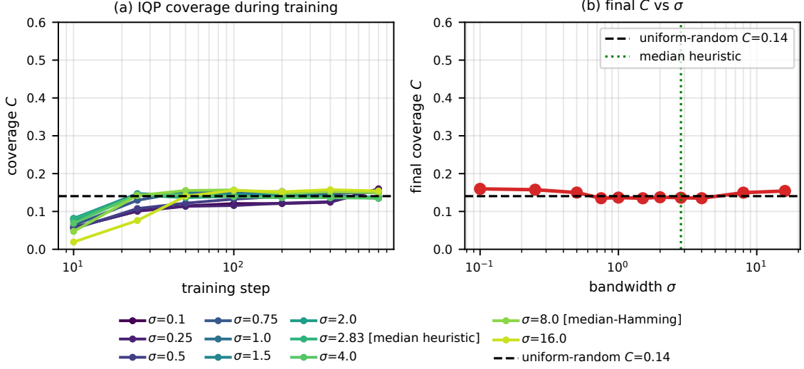
FIG. 12. No kernel bandwidth rescues IQP coverage. IQP coverage as the kernel bandwidth \sigma is swept from sharp (0.1) to broad (16) at N = 16 , including the median heuristic (Euclidean, \sigma = 2.83 ) and the median Hamming value ( \sigma = 8 ). (a) coverage during training for each \sigma ; (b) final coverage versus \sigma . IQP stays at 0.13 to 0.16, near the random-bit baseline C_{\text{rand}} (dashed), for every \sigma ; the likelihood-trained baselines of Table II reach \sim 0.5 on the same task.
