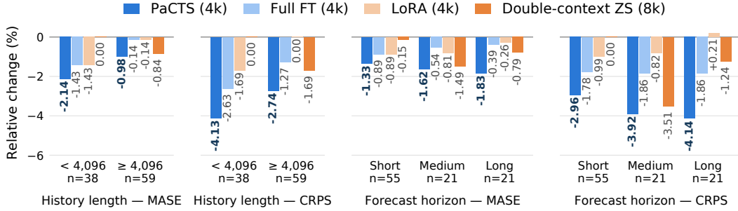
Figure 3: Effects of history length and forecast horizon. The bars show percentage changes in MASE and CRPS relative to zero-shot Chronos-2 at 4,096 steps. Negative values indicate improvements. The left two panels group configurations by history lengths, and the right two by forecasting horizons. PaCTS performs consistently better than other methods and double-context zero-shot forecasts. Detailed numbers are in Appendix D.
