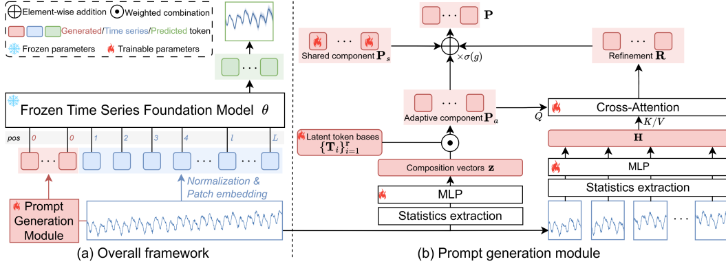
Figure 2: Overview of PaCTS. (a) A lightweight prompt generation module maps the context to instance-adaptive latent prompts: continuous vectors prepended to the time-series embeddings. (b) Global context statistics determine a weighted combination of learnable prompt basis patterns, yielding the adaptive component \mathbf{P}_a(\mathbf{x}) . Segment-level statistics are encoded with relative-position embeddings and retrieved through cross-attention to produce a refinement \mathbf{R}(\mathbf{x}) . The adaptive component and its refinement are combined, gated, and added to the shared component \mathbf{P}_s to form the final prompts.
