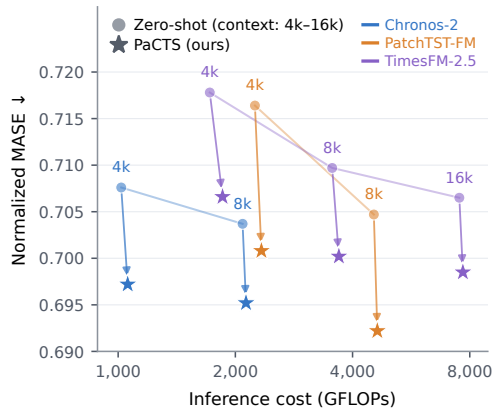
Figure 1: PaCTS improves forecasting at lower additional cost than extending context.
