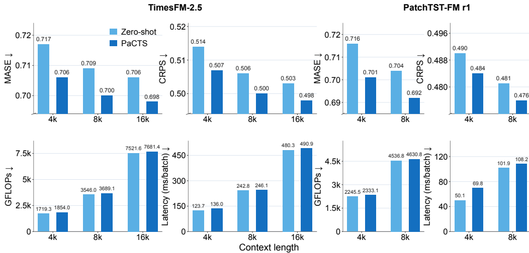
Figure 5: Forecasting performance (top) and computational costs (bottom) across backbones on GIFT-Eval. Lower values are better for all metrics. As with Chronos-2, shorter-context PaCTS achieves competitive or better performance than longer-context zero-shot baselines, with substantially lower computational costs.
