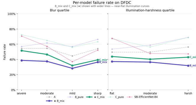
Fig. 3. Per-model failure rate on DFDC by blur quartile (left) and illumination-harshness bin (right). B_mix and C_mix—the T-SBI contrast—are near-flat on the illumination axis, with no preferential reduction on the harsh bin.
