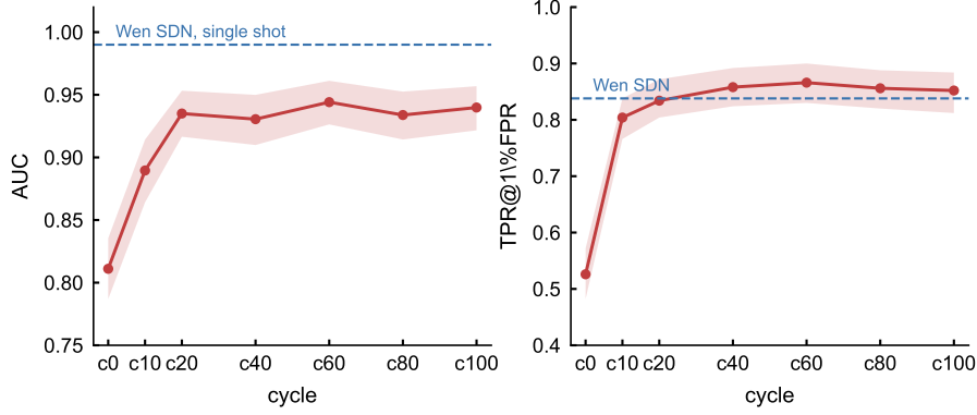
Figure 22: AUC and TPR@1%FPR against cycle count, with bootstrap bands.
