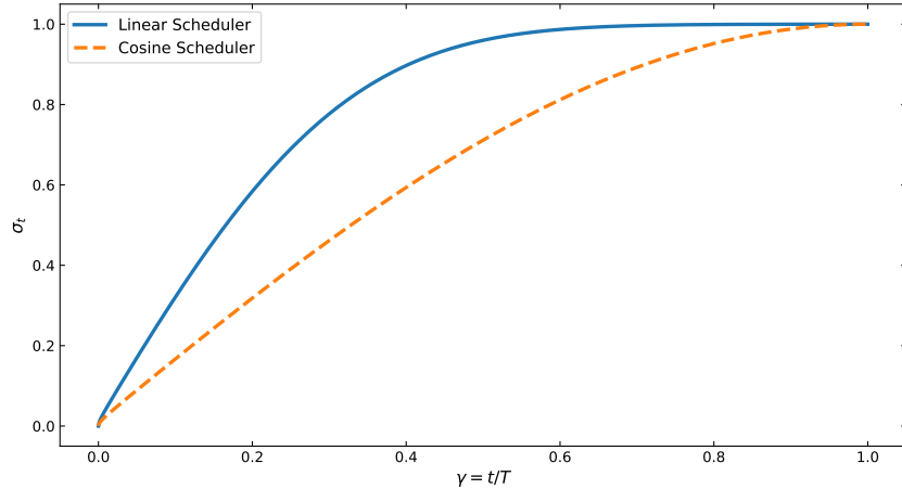
Figure 5: Comparison of the noise standard deviation ( \sigma_t = \sqrt{1 - \bar{\alpha}_t} ) versus the normalized timestep ( \gamma = t/T ) for linear and cosine noise schedulers. The cosine scheduler maintains lower noise magnitude for a significantly broader range of timesteps.
