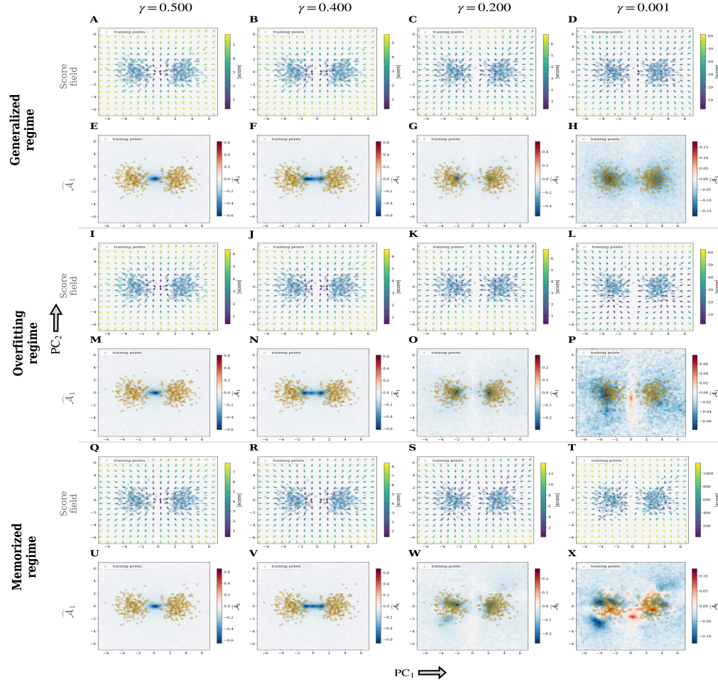
Energy-landscape geometry vs. cyclic-denoising noise amplitude across training regimes
