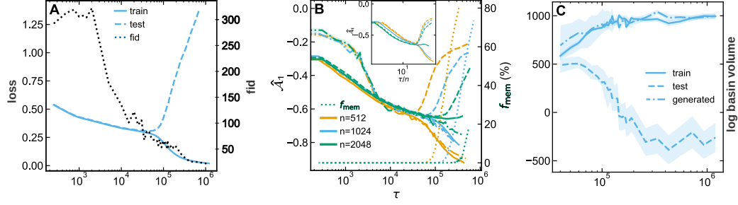
Figure 2: Geometric signatures across training on CelebA. (A) Training loss (solid), held-out loss (dashed), and FID (dotted, right axis) for n = 1024 . (B) \hat{\mathcal{A}}_1 at \gamma = 0.001 and f_{\text{mem}} (dotted, right axis) for n = 512 (orange), 1024 (blue), and 2048 (green); training (solid), held-out (dashed), and generated (dash-dot) samples. Inset: divergence against \tau/n . (C) Mean log basin volume for n = 1024 over all training samples and an equal number of generated and held-out samples, with line styles as in (B); bands show one standard deviation across samples. Refer Appendix G for equivalent results on Adam Optimizer
