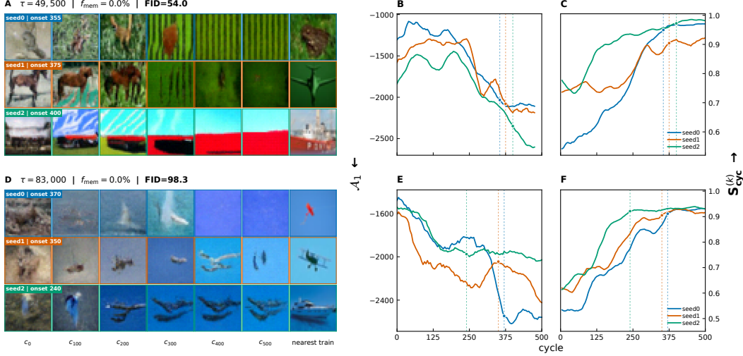
Figure 4: Cyclic denoising reveals degenerate attractors. CIFAR-10 ( n = 8192 , \gamma = 0.05 ) at \tau_{\text{gen}} = 49,500 (A–C) and \tau = 83,000 (D–F). (A,D) Three trajectories from c_0 to c_{500} with the nearest training image to the final state; no attractor matches a single training image. (B,E) \Delta\mathcal{A}_1 and (C,F) S_{\text{cyc}}^{(k)} across cycles. Markers show the residence onset, which does not indicate memorization.
