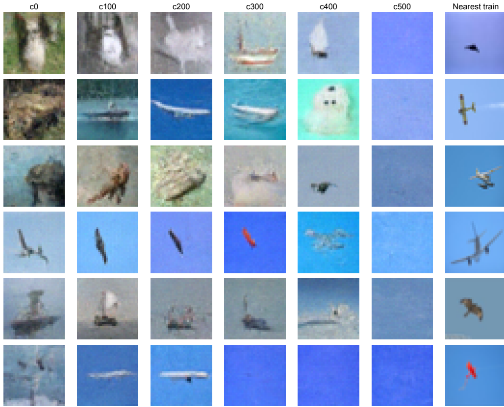
Figure 10: Fading structure on CIFAR-10. \tau = 83,000 , \gamma = 0.05 ; f_{\text{mem}}^{\text{gen}} = 0\% and full-cohort f_{\text{mem}}^{\text{CD}}(500) = 3.1921\% . Six appearance-selected trajectories lose semantic structure and approach nearly monochromatic blue configurations.
