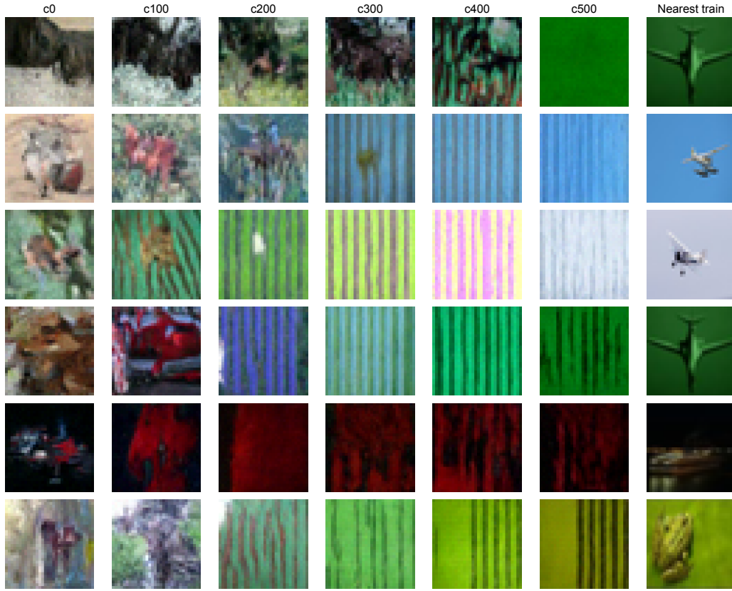
Figure 11: Stripe-like and monochromatic degeneration on CIFAR-10. \tau = 49,500 , \gamma = 0.05 ; f_{\text{mem}}^{\text{gen}} = 0\% and full-cohort f_{\text{mem}}^{\text{CD}}(500) = 0\% . Trajectories develop repeated spatial bands or nearly monochromatic fields.
