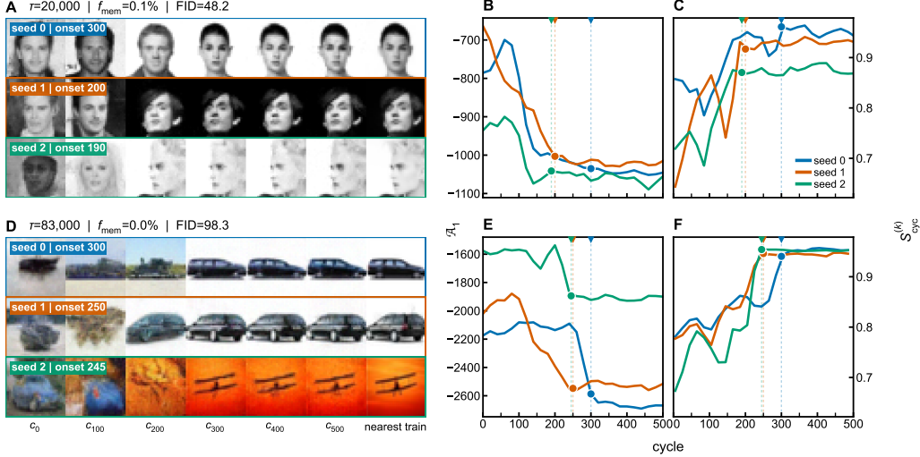
Figure 14: Trajectories discover and reside in basins corresponding to training samples. (A) CelebA trajectories ( n = 4096 , Adam, \gamma = 0.10 ) from c_0 to c_{500} , with the nearest training image to each final state. The marked onset is the first cycle at which a trajectory satisfies the f_{\text{mem}} criterion and remains classified as memorized for the rest of the run. (B) Score divergence \mathcal{A}_1 decreases as the trajectories approach these states; the decline can begin before the marked onset. (C) Consecutive-state LPIPS cosine similarity S_{\text{cyc}}^{(k)} increases and reaches a high plateau, consistent with residence after the approach. (D–F) The corresponding CIFAR-10 trajectories ( n = 8192 , Adam, \gamma = 0.05 ) and measurements. Colors identify trajectories across panels. Dotted lines and markers show their onsets. Divergence and similarity are displayed with a centered 50-cycle moving average. Annotations above A and D give the training step \tau , one-shot f_{\text{mem}} , and FID.
