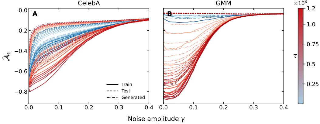
Figure 20: Normalized score divergence versus noise amplitude \gamma across all training checkpoints , for CelebA (a) and the GMM (b). Each curve is one checkpoint, coloured by training regime: blue for the generalized regime and orange for the memorized regime, with lighter to darker shades as the training step \tau increases within each regime. Line style distinguishes train, test, and generated samples. In the generalized regime (blue) the curves are shallow and cluster together across all \gamma . In the memorized regime (orange) the normalized divergence is strongly negative at small \gamma and rises toward zero as \gamma increases, with the effect deepening as \tau grows.
