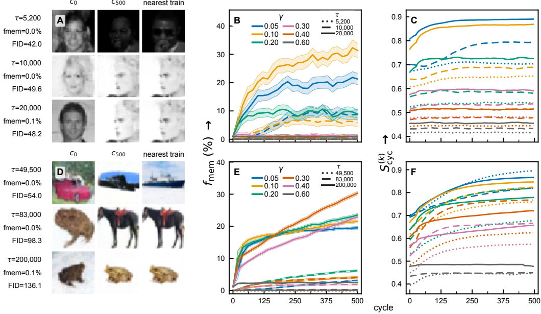
Figure 3: Cyclic denoising exposes latent memorization inside the generalization window. CelebA ( n = 4096 , Adam; A–C) and CIFAR-10 ( n = 8192 ; D–F) at checkpoints from \tau_{\text{gen}} to \tau_{\text{mem}} . (A,D) Generated samples at c_0 and c_{500} ( \gamma = 0.10 ) with their nearest training images. (B,E) f_{\text{mem}} and (C,F) S_{\text{cyc}}^{(k)} across cycles for several \gamma .
