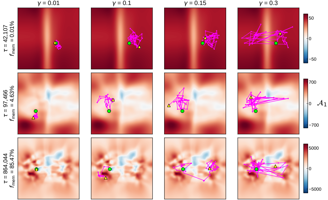
Figure 8: Cyclic-denoising trajectories on the GMM score-divergence landscape. GMM, n = 512 . Rows are checkpoints of increasing \tau , with their one-shot f_{\text{mem}} ; columns are cycling amplitudes \gamma . The background is the exact score divergence \mathcal{A}_1 of the learned score on a two-dimensional plane spanned by the direction joining the two component means and the leading orthogonal principal direction of the training data; red marks negative (contracting) values. Each row has its own colour scale, since the range grows from about \pm 60 to \pm 6,000 during training. The magenta path joins the projected states of one trajectory every 5 cycles over 200 cycles, from the start (green dot) to the end (yellow triangle). Because states are projected onto the plane, the path shows direction of motion rather than exact position on the background.
