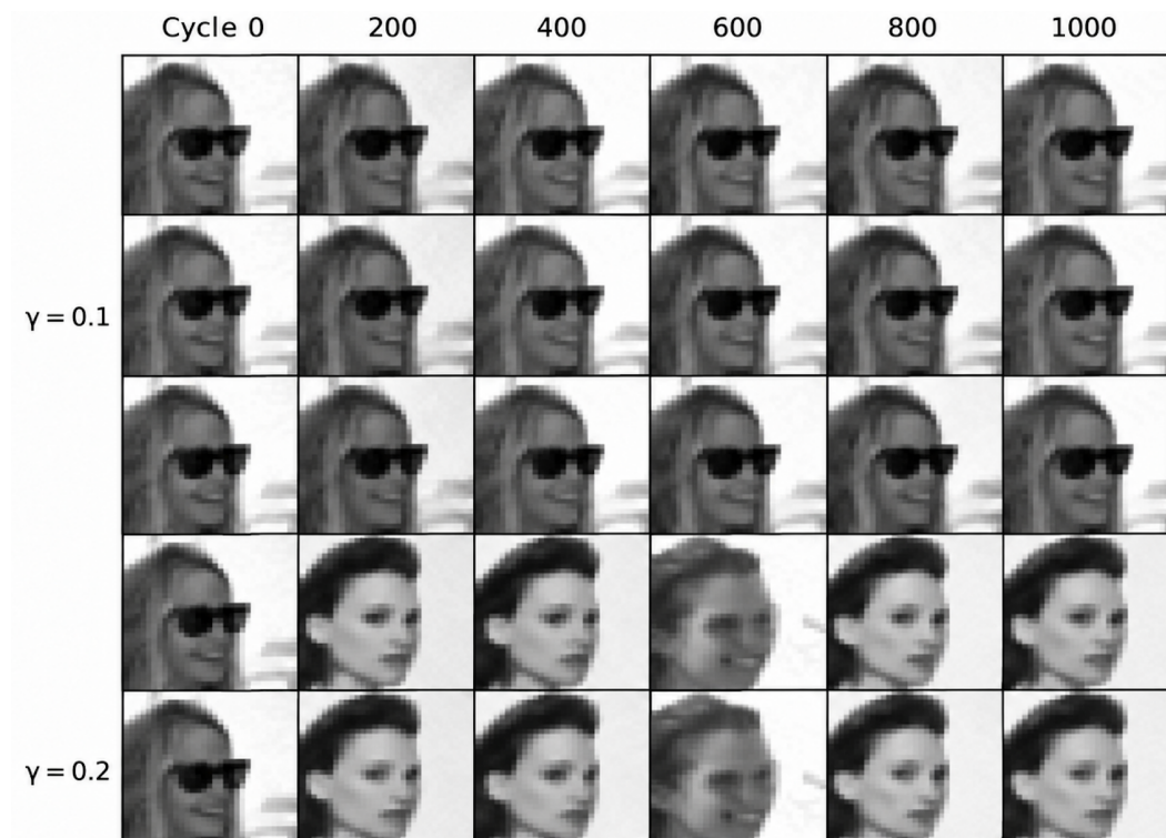
Figure 15: Basin residence and jumping under repeated cycling at \tau = 40,000 (run: CelebA32, UNet, n = 4096 , Adam). Both sets begin in the basin associated with the same memorised training example. At \gamma = 0.1 (top), trajectories remain in this basin. At \gamma = 0.2 (bottom), stronger perturbations induce basin jumping, followed by sustained residence in another attractor, consistent with greater stability under cycling.
