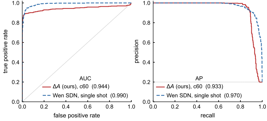
Figure 23: ROC (left) and precision–recall (right) at c = 60 . Class balance is 1:4; the dotted line in the right panel marks the positive rate.
