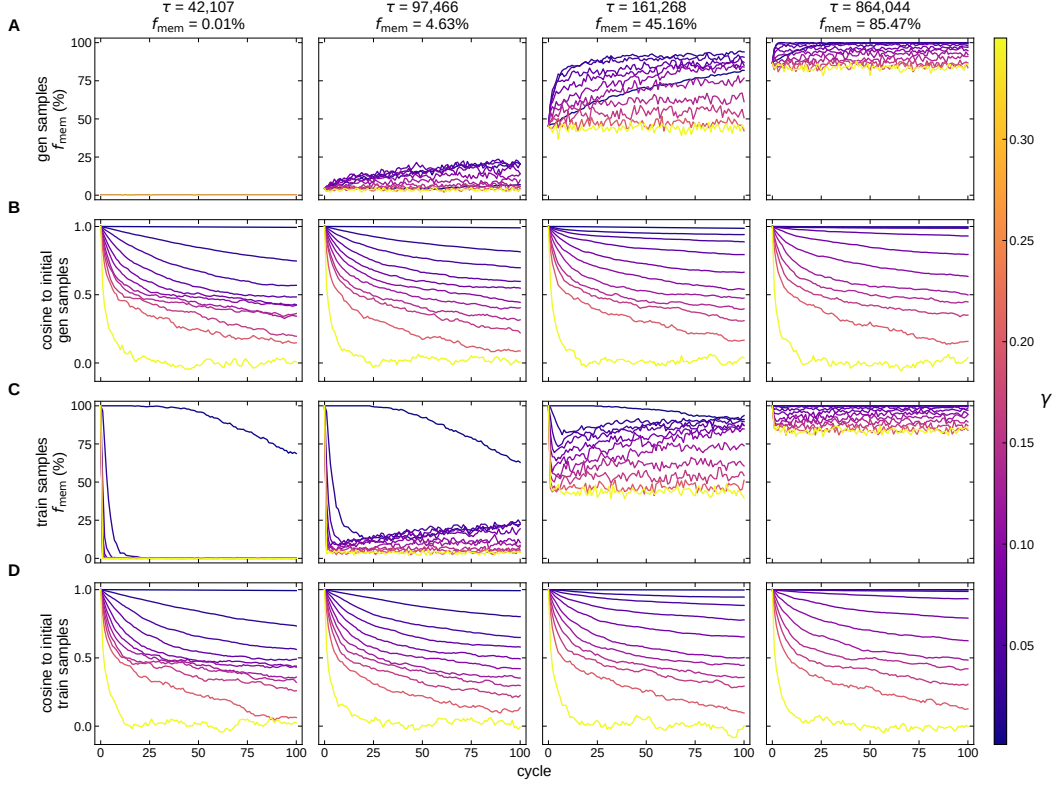
Figure 7: Cyclic denoising on the GMM across training. GMM, n = 512 . Columns are checkpoints of increasing \tau , with their one-shot f_{\text{mem}} . Each panel shows 512 trajectories per amplitude, coloured by \gamma ( 0.001 \leq \gamma \leq 0.35 ). (A) f_{\text{mem}} versus cycle for trajectories started from generated samples. (B) Mean cosine similarity between each state and its starting sample, computed on the raw 8-dimensional vectors, for the same trajectories. (C, D) The same quantities for trajectories started from the training points. Cycling raises f_{\text{mem}} above its one-shot value at small \gamma once basins have formed, while at \tau = 42,107 even training points are not retained.
