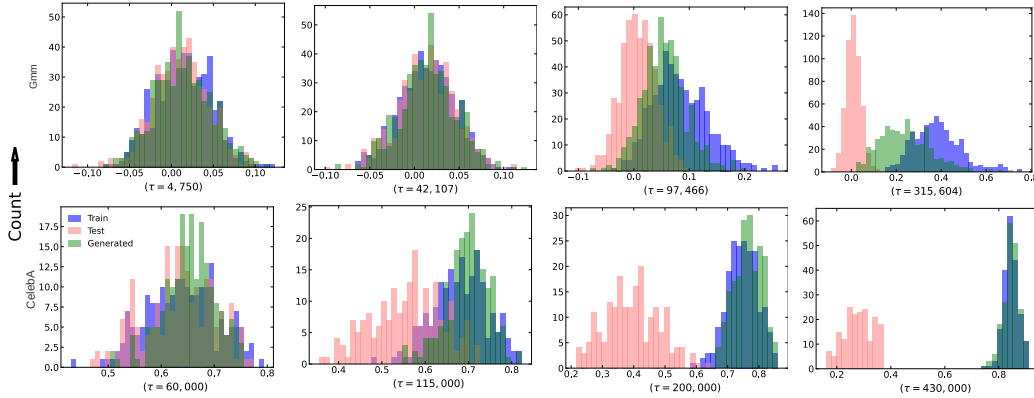
Figure 16: Distribution of the membership score (the sign-flipped normalized score divergence \hat{A}_1 ) for training (blue), held-out test (red), and generated (green) samples, at increasing training steps \tau (left to right), for GMM (top row) and CelebA (bottom row). The three distributions overlap in the generalized regime and separate—with training and generated moving together, away from test—as the model memorizes.
