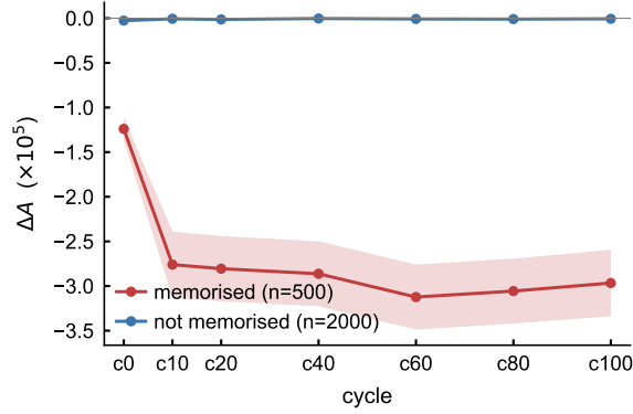
Figure 24: Raw \Delta A against cycle, population means with 95% intervals. Memorised prompts move from -1.24 \times 10^5 at c = 0 to -3.12 \times 10^5 at c = 60 ; non-memorised prompts remain within 0.03 \times 10^5 of zero.
