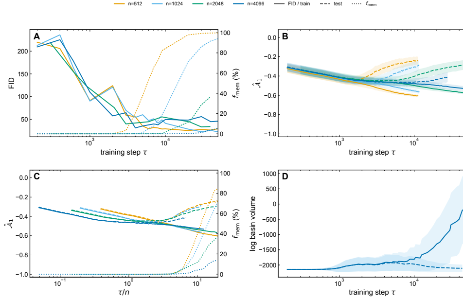
Figure 17: CelebA width-64 U-Net trained with Adam, number of training samples - n = 512, 1024, 2048, 4096 . A: FID and memorization fraction, f_{mem} , versus training step \tau . B: The normalized score divergence \hat{\mathcal{A}}_1 for train and held-out test samples versus \tau ; bands show \pm 1 standard deviation across samples. Consistent lag between train-test \hat{\mathcal{A}}_1 split and onset of f_{mem} . C: The same \hat{\mathcal{A}}_1 curves and f_{mem} versus normalized training steps \tau/n . D: For the n = 4096 run, mean log basin-volume proxy for training and test images versus \tau , with \pm 1 standard deviation.
