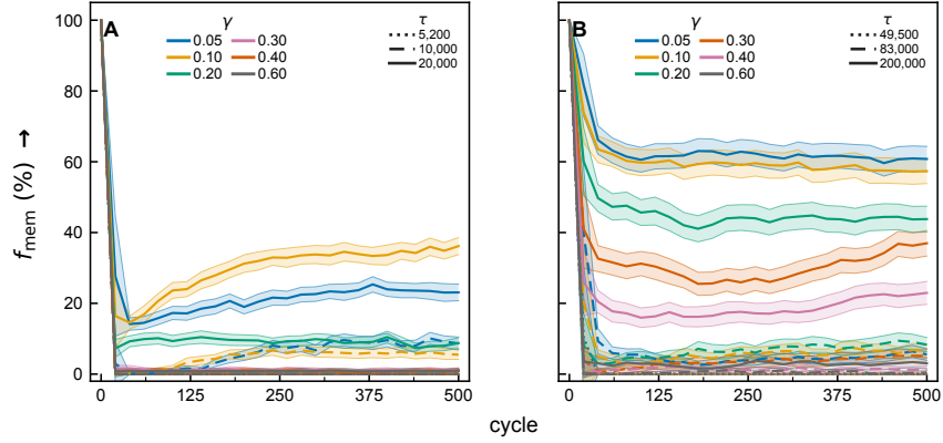
Figure 13: Cyclic denoising from training samples. Memorization fraction f_{\text{mem}} across 500 cycles for trajectories initialized from training images in (A) CelebA ( n = 4096 , Adam, linear noise schedule) and (B) CIFAR-10 ( n = 8192 , Adam, cosine noise schedule). Although f_{\text{mem}} starts at 100%, it drops sharply under cycling. At \tau_{\text{gen}} , it remains near zero, whereas later checkpoints retain or recover a larger fraction, depending on \gamma . Classification is against the full training set and does not require returning to the initial training image. Shaded bands combine the reported bootstrap standard errors with variation within each cycle bin. The memory of the initial train samples can be lost under cycling, basin residence only remains in a subset of train samples that become attractors (subject to cycling amplitude). Cycling moves trajectories to other stronger attractor basins.
