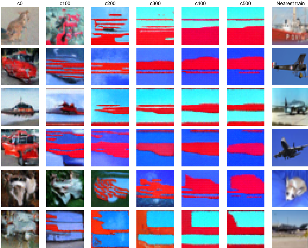
Figure 9: Saturated geometric degeneration on CIFAR-10. \tau = 49,500 , \gamma = 0.05 ; f_{mem}^{gen} = 0\% and full-cohort f_{mem}^{CD}(500) = 0\% . Repeated CD replaces recognizable content with saturated bands and colour blocks. The final column shows the nearest training image to c500.
