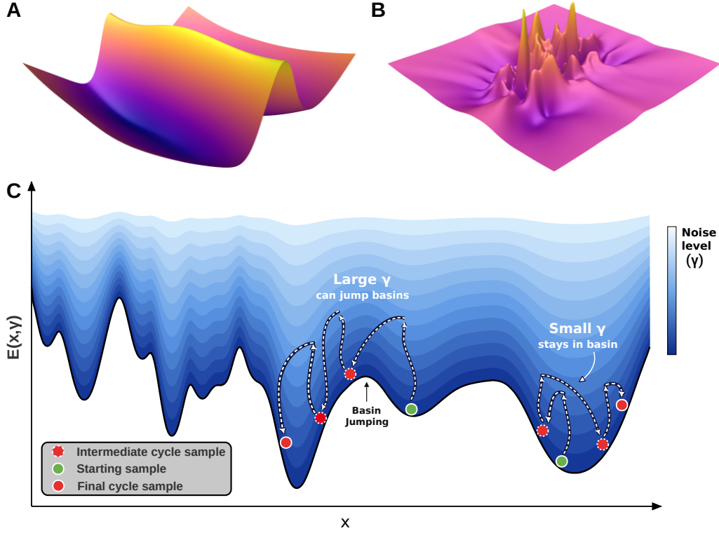
Figure 1: Memorization forms sharp, localized basins in the learned score field. (A,B) Normalized score divergence \hat{\mathcal{A}}_1 for an eight-dimensional Gaussian mixture model (GMM), on a two-dimensional slice of the sample space obtained with the projection of Bihani et al. (2024) (App. G.6). (A) In the generalized regime, the field is smooth, with no prominent structure around training samples. (B) As memorization emerges, strongly negative regions form around training samples. (C) Schematic of cyclic denoising: at low noise, trajectories remain within a basin, whereas at sufficiently large noise they jump to neighbouring basins.
