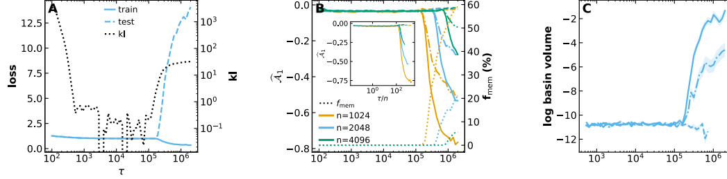
Figure 6: Geometric signatures across training on the GMM. (A) Train loss (solid) and test loss (dashed) at \gamma = 0.01 on the left axis, and D_{\text{KL}}(P_\theta \| P_0) (dotted, log scale) on the right axis, versus training step \tau , for n = 2048 . (B) Mean normalized score divergence \hat{\mathcal{A}}_1 on the left axis and f_{\text{mem}} (dotted) on the right axis, versus \tau . Line style denotes the sample group: train (solid), test (dashed), generated (dash-dot). Colour denotes the training-set size: n = 1024 (orange), n = 2048 (blue), n = 4096 (green). Inset : the same divergence curves against \tau/n . (C) Mean log basin volume versus \tau for n = 2048 , with the line styles of (B); bands show one standard deviation across samples.
