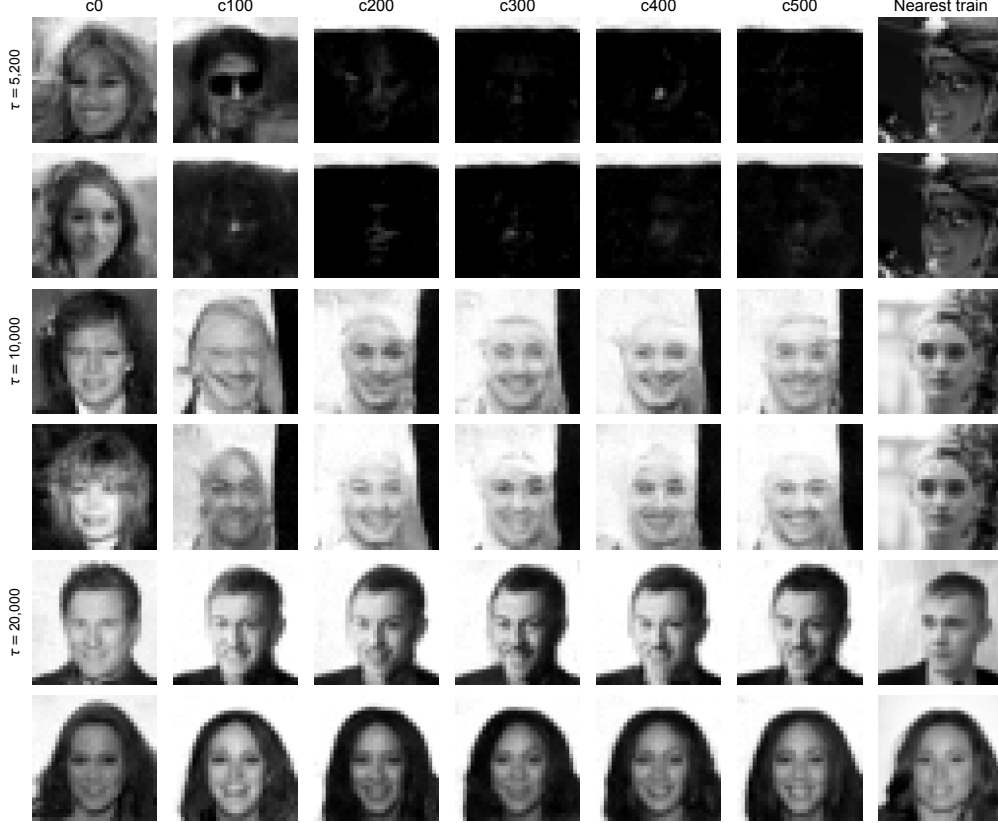
Figure 12: CelebA CD trajectories across training checkpoints , \gamma = 0.05 . Top, middle and bottom pairs correspond to \tau = 5,200 , 10,000 and 20,000 , respectively. Their logged f_{\text{mem}}^{\text{gen}} values are 0%, 0% and 0.1308%; full-cohort f_{\text{mem}}^{\text{CD}}(500) values are 0%, 9.8% and 21.12%. At \tau = 5200 the images move towards mere monochromatic darkness and remain stable there. For \tau = 10000 and \tau = 20000 more facial structure emerges for these non memorized basins.
