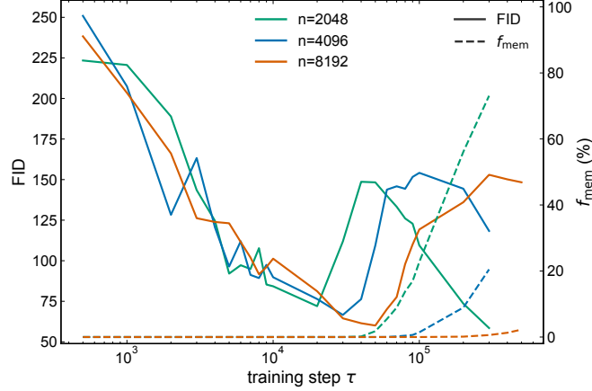
Figure 18: FID and memorization ratio of CIFAR-10 DiT-S runs with Adam optimizer and Cosine Noise Scheduler with n=2048, 4096, 8192 .
