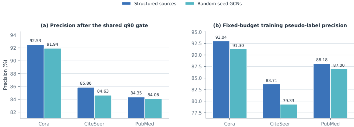
Figure 4: Pseudo-label quality for structured sources and three random-seed GCNs (five-seed means). Left: conditional precision after the shared q90 structural gate. Right: fixed-budget training pseudo-label precision without q90 filtering. The panels evaluate different branches and should not be compared numerically across panels.
