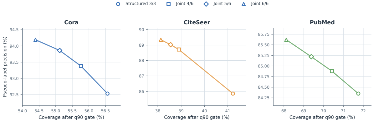
Figure 3: Precision-coverage tradeoff after the common q90 structural gate (five-seed means). Lines connect adjacent voting strictness levels only to show direction and are not continuous threshold curves.
