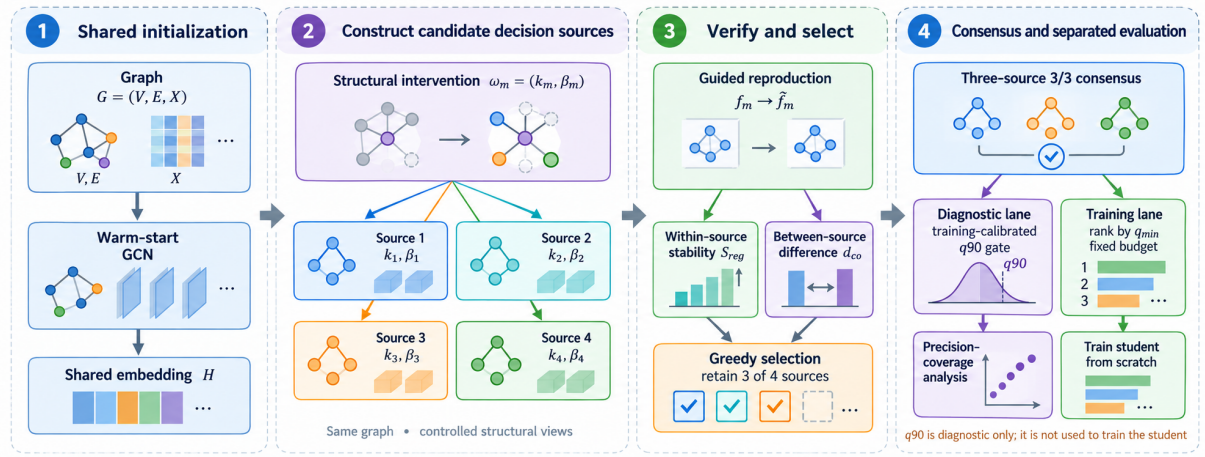
Figure 1: Overview of structured decision-source construction. Structural interventions (k, \beta) generate four candidates from a shared warm-start representation. Reproduction stability and between-source co-assignment differences select three sources. Their consensus candidates enter either the q90 quality diagnostic or minimum-confidence ranking for student training; the q90 gate is not used in student training.
