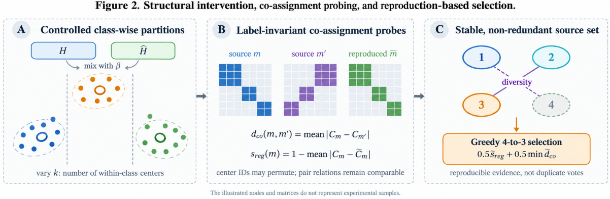
Figure 2: Structural intervention, co-assignment probing, and reproduction-based selection. Varying k and \beta creates different within-class partitions. Co-assignment matrices remove center-label permutations, and within-source stability s_{\text{reg}} and between-source difference d_{\text{co}} select three stable, nonduplicate sources. The illustrated nodes and matrices do not represent experimental samples.
