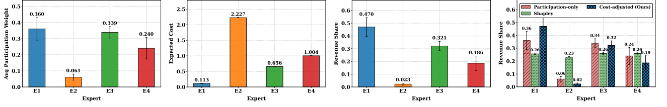
Figure 4: Revenue-allocation behavior on Breast Cancer (Case 1). From left to right, the panels show average participation weight, normalized expert unit cost, the proposed cost-adjusted revenue share at \lambda = 0.6 , and the comparison among participation-only, exact Shapley, and cost-adjusted allocation.
