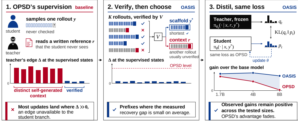
Figure 3: OPSD versus OASIS. (1) OPD distills along a single unverified rollout y , so most updates land where the teacher’s edge from the hidden reference r is large. (2) OASIS samples K rollouts, verifies them, and takes the shortest verified one as scaffold y^* and another same-problem rollout as context r , typically unverified as context r , where the teacher’s edge is small. (3) The student is trained against the frozen teacher with the unchanged OPD loss.
