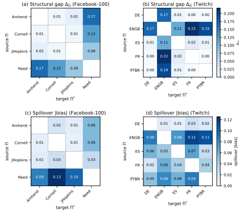
Figure 2: Structural gap \Delta_G (top) and transported spillover bias (bottom) across all within-family source-target pairs. The two panels in each row share one colour scale.
